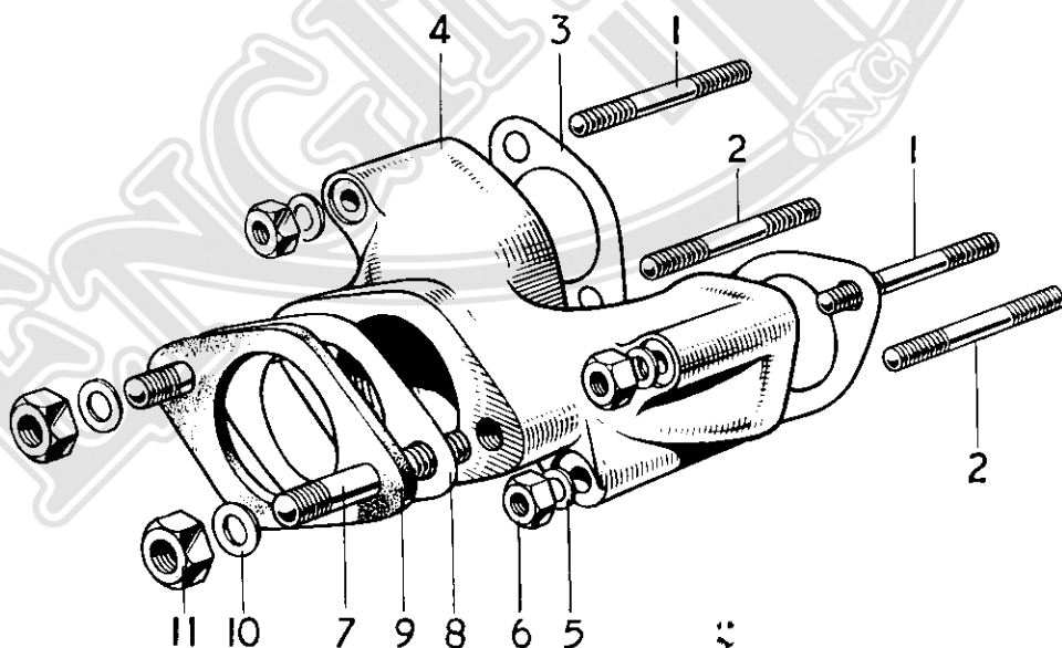
Fig. 3. OIL PUMP, RELEASE VALVE AND INLET MANIFOLD 951-940-5411
