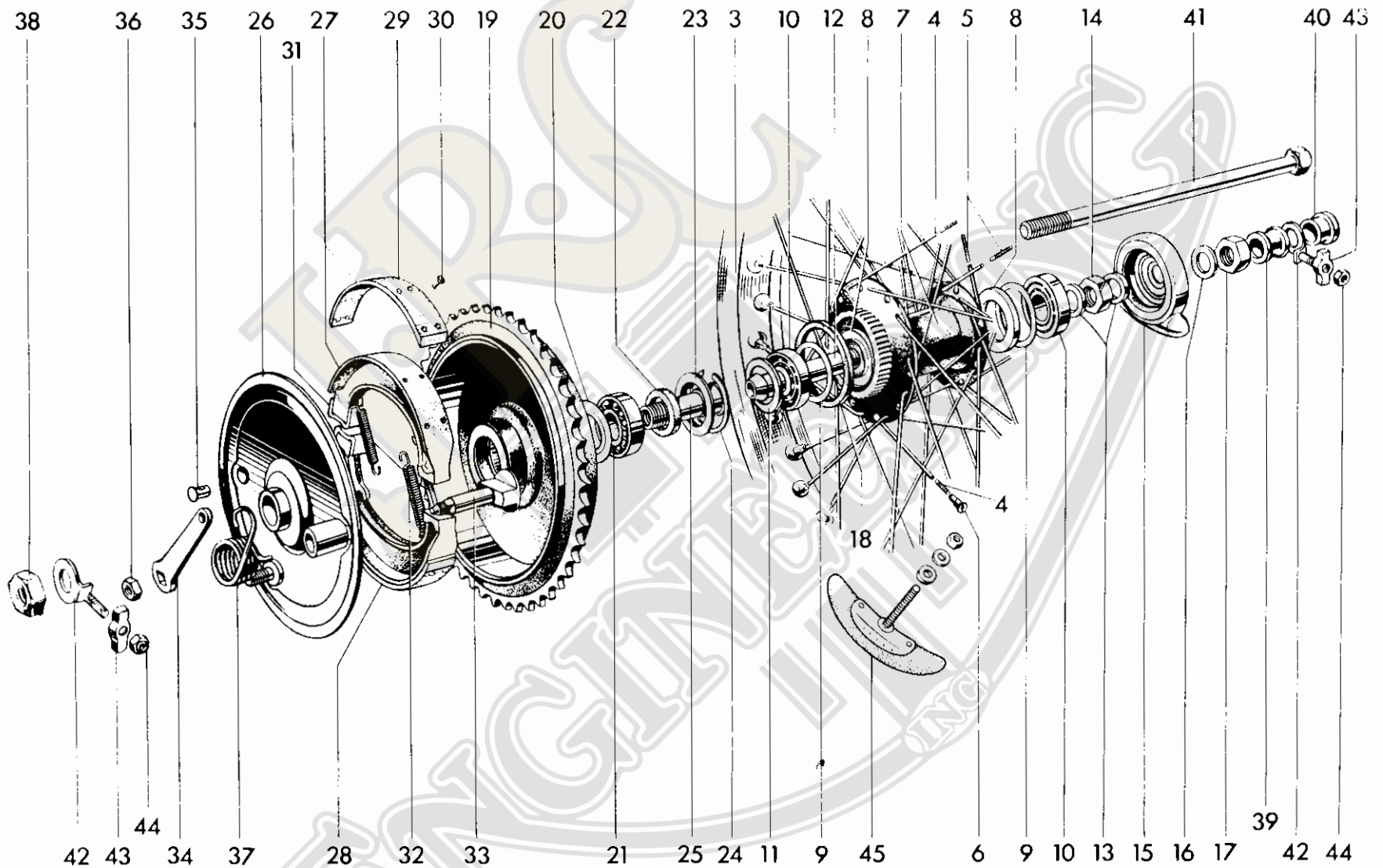
Fig. 19 WHEEL www.jrcengineering.com 951-940-5411
