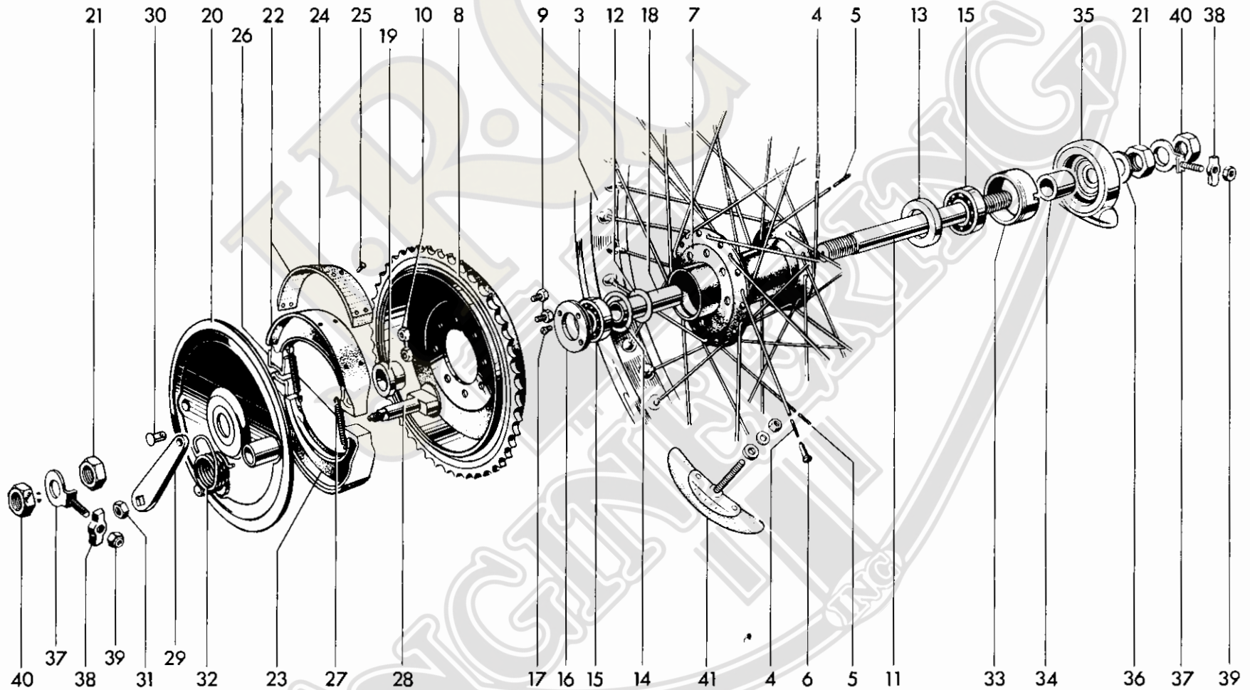
Fig. 18. REAR WHEEL
