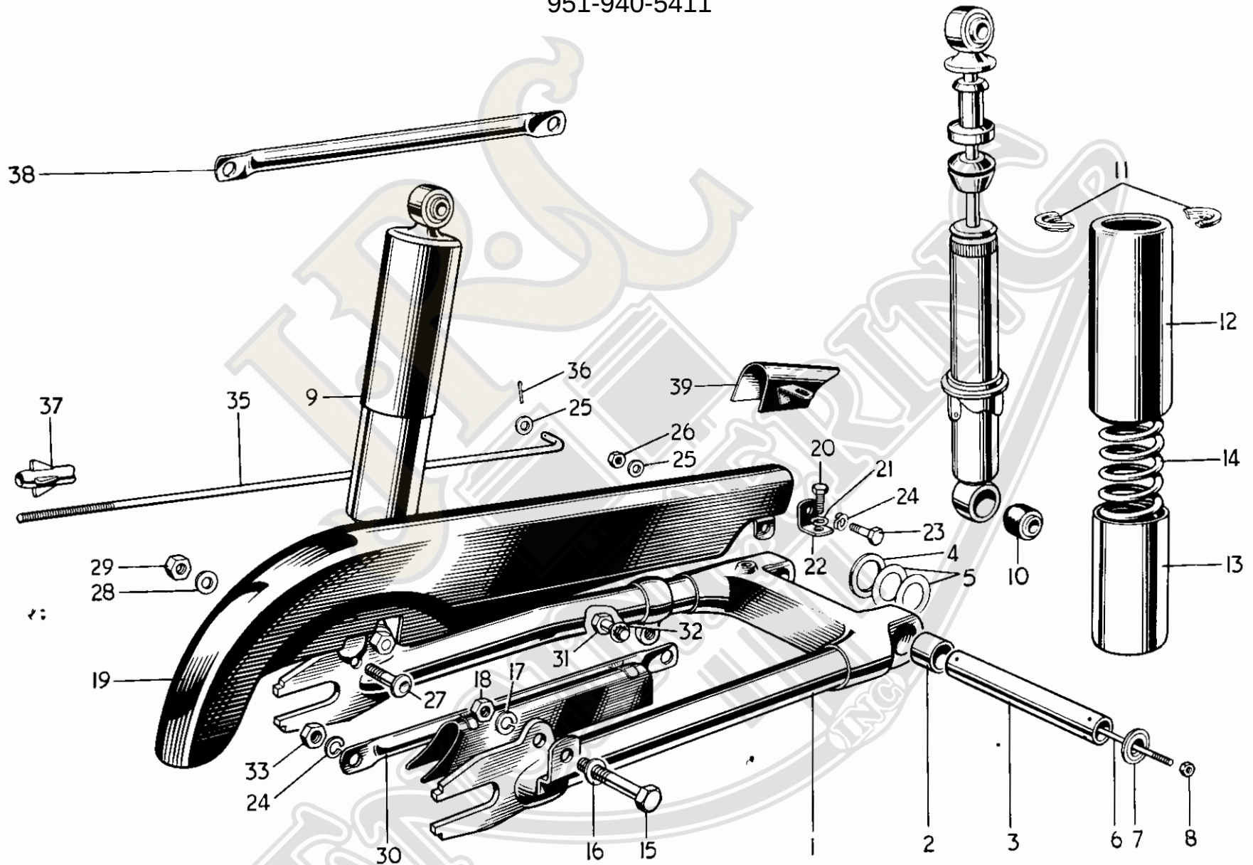
Fig. 13. SWINGING FORK, SUSPENSION UNITS AND CHAINGUARD www.jrcengineering.com 951-940-5411
