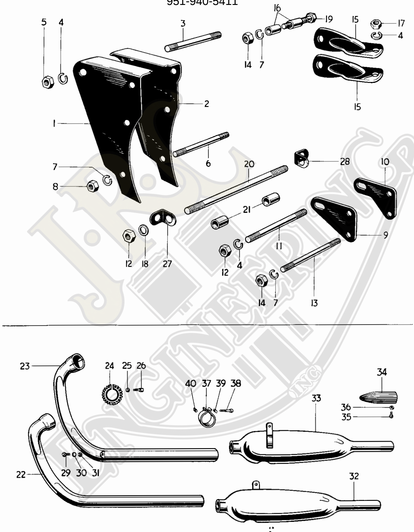
Fig. 11. ENGINE FITTINGS AND EXHAUST SYSTEM
