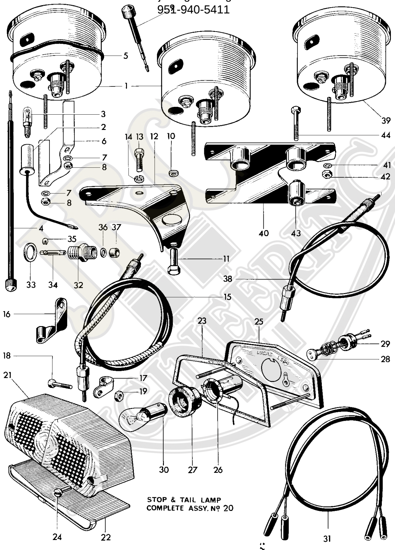
Fig. 29. STOP & TAIL LAMP COMPLETE ASSY. N° 20 www.jrcengineering.com 951-940-5411
