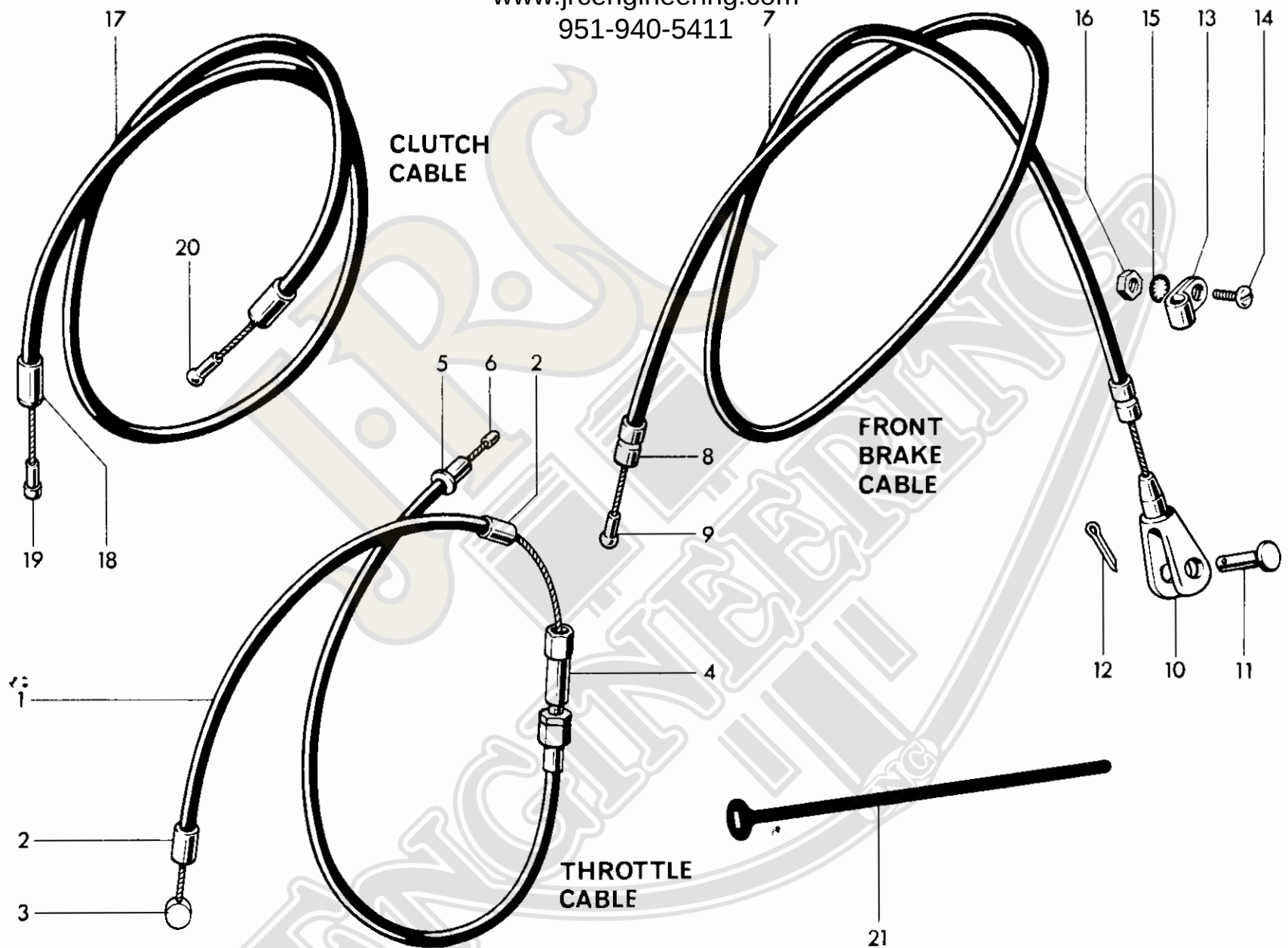
Fig. 25. CONTROL CABLES www.jrcengineering.com 951-940-5411
