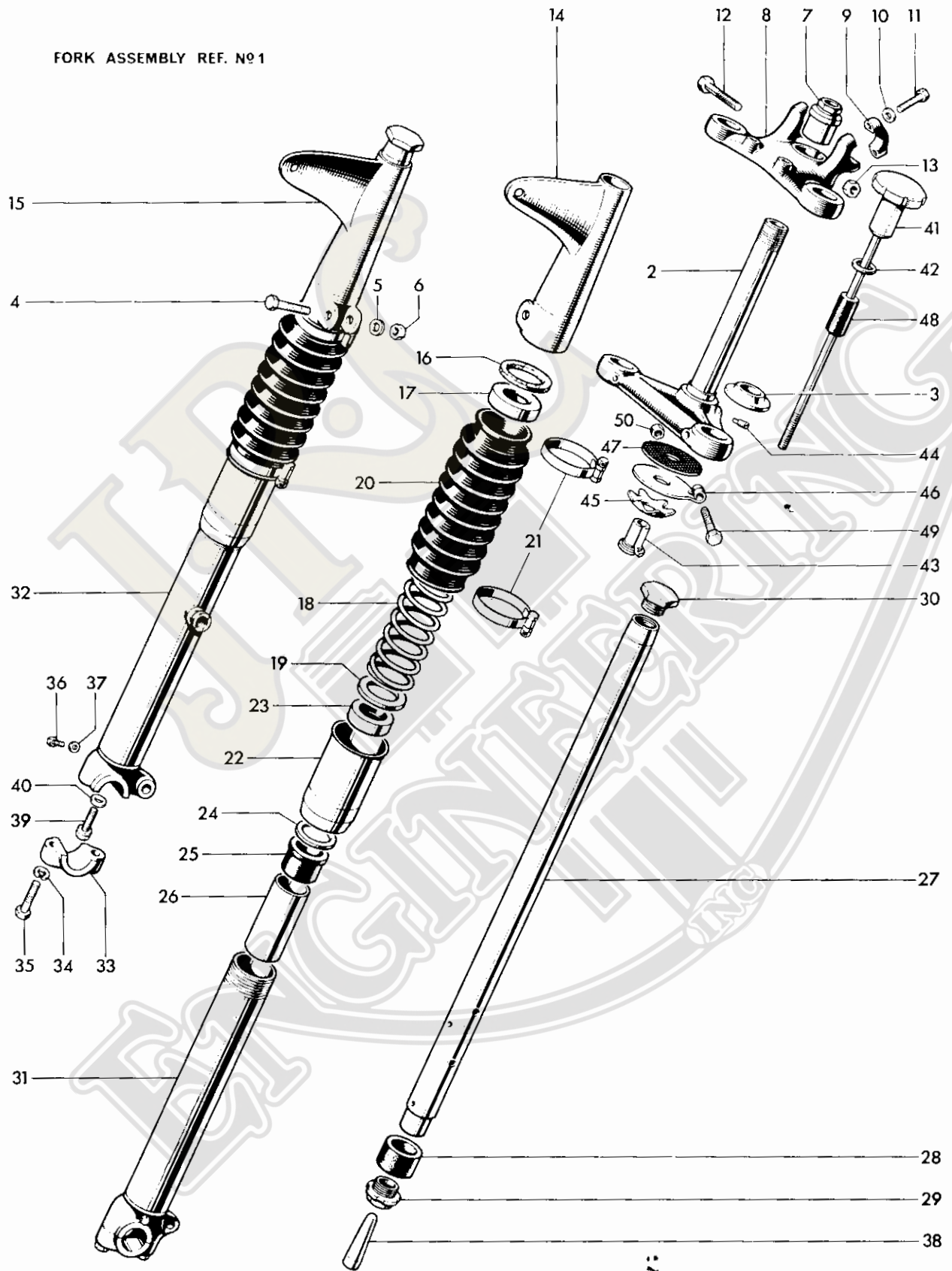
Fig. 16. TELESCOPIC FRONT FORK, T190 AND T100SS www.jrcengineering.com 951-940-5411
