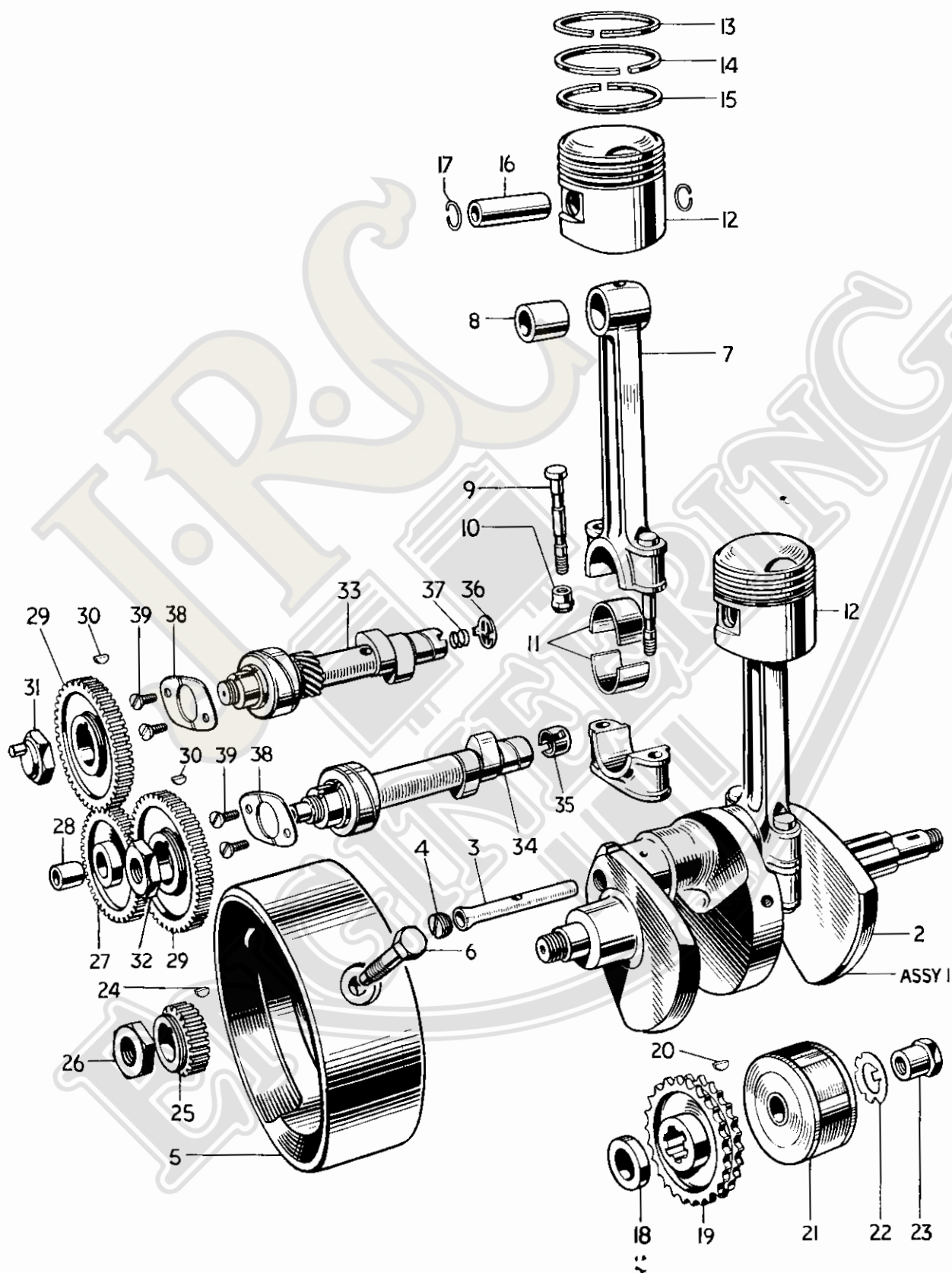
Fig. 1. CRANKSHAFT AND CONNECTING RODS www.jrcengineering.com 951-940-5411
