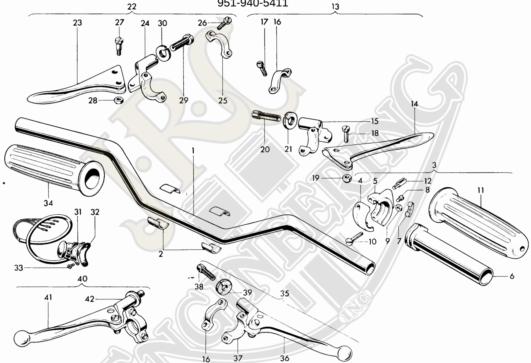
www.jrcengineering.com Fig. 28. HANDLEBARS AND CONTROL LEVERS 951-940-5411
