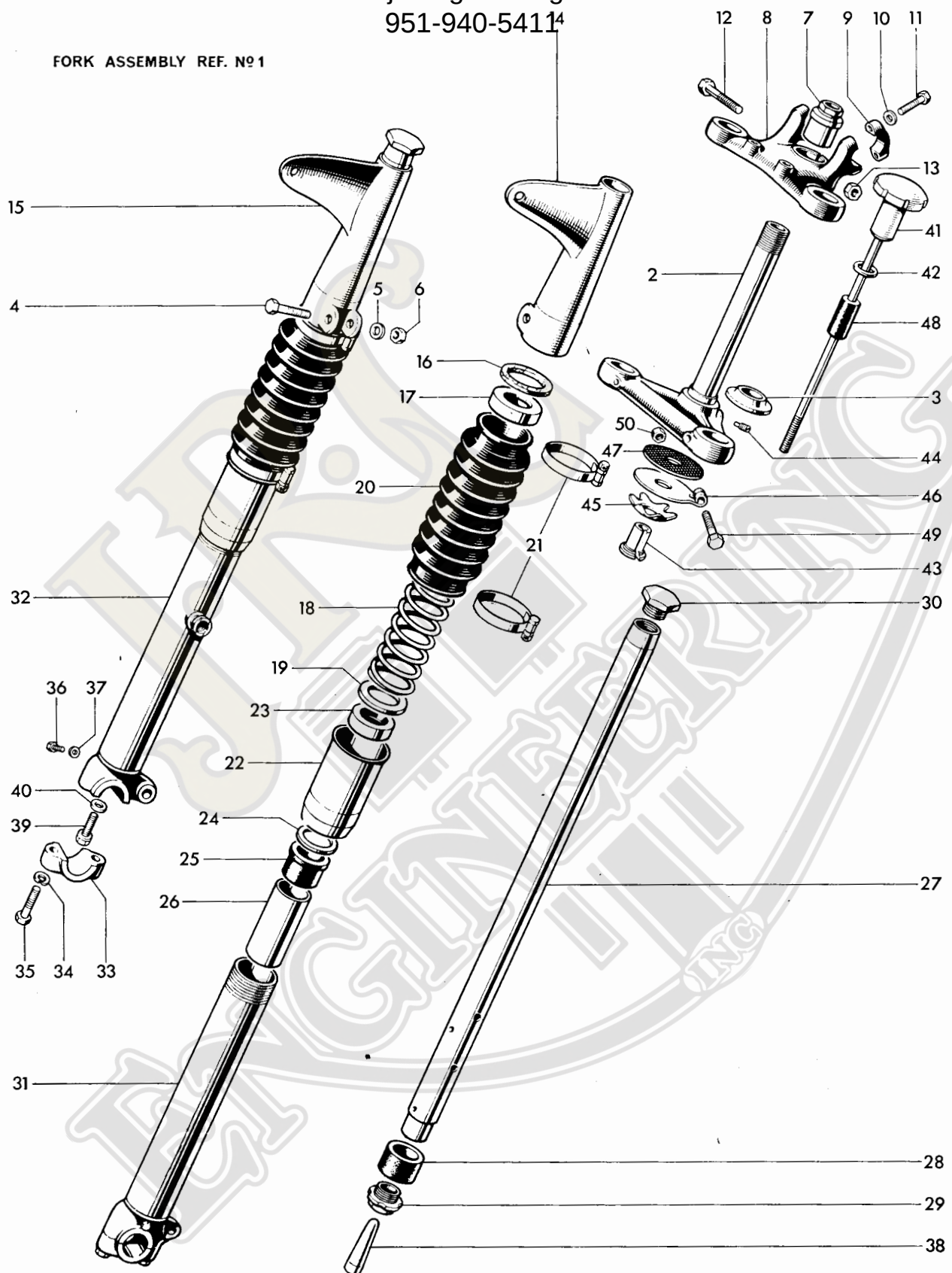
Fig. 17. TELESCOPIC FRONT FORK, T90 AND T100 www.jrcengineering.com 951-940-5411
