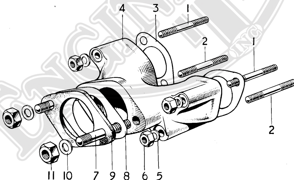
Fig. 3. OIL PUMP RELEASE VALVE MANIFOLD
