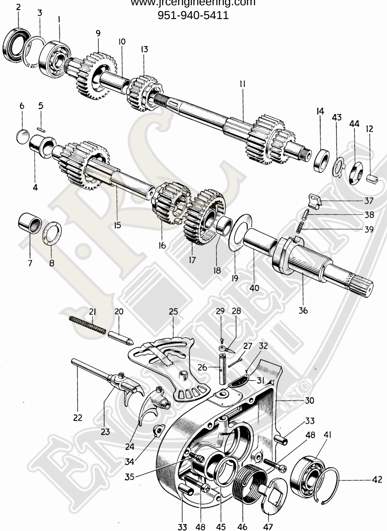
Fig. 7. GEARBOX SHAFTS, GEARS AND INNER COVER
