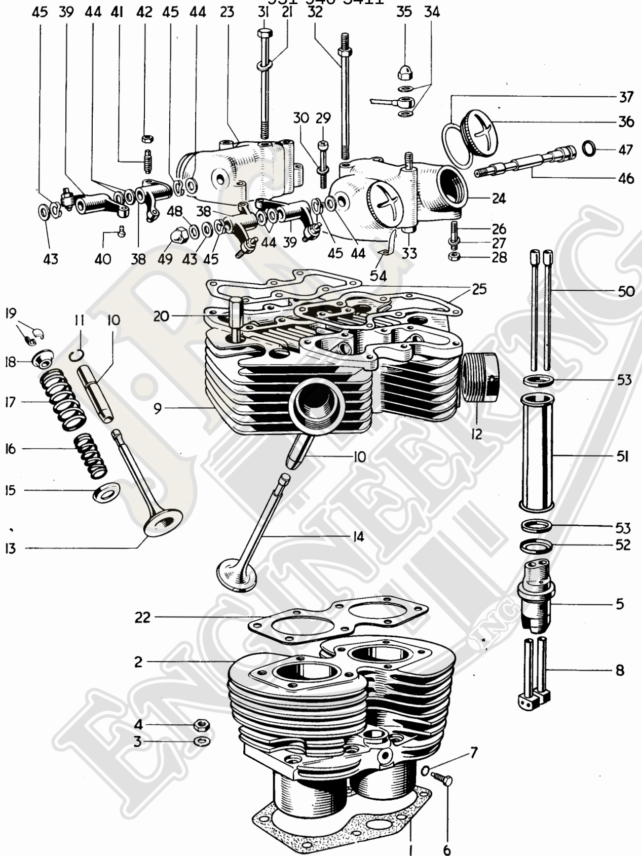
Fig. 4. CYLINDER BLOCK AND HEAD, 30A AND T90
