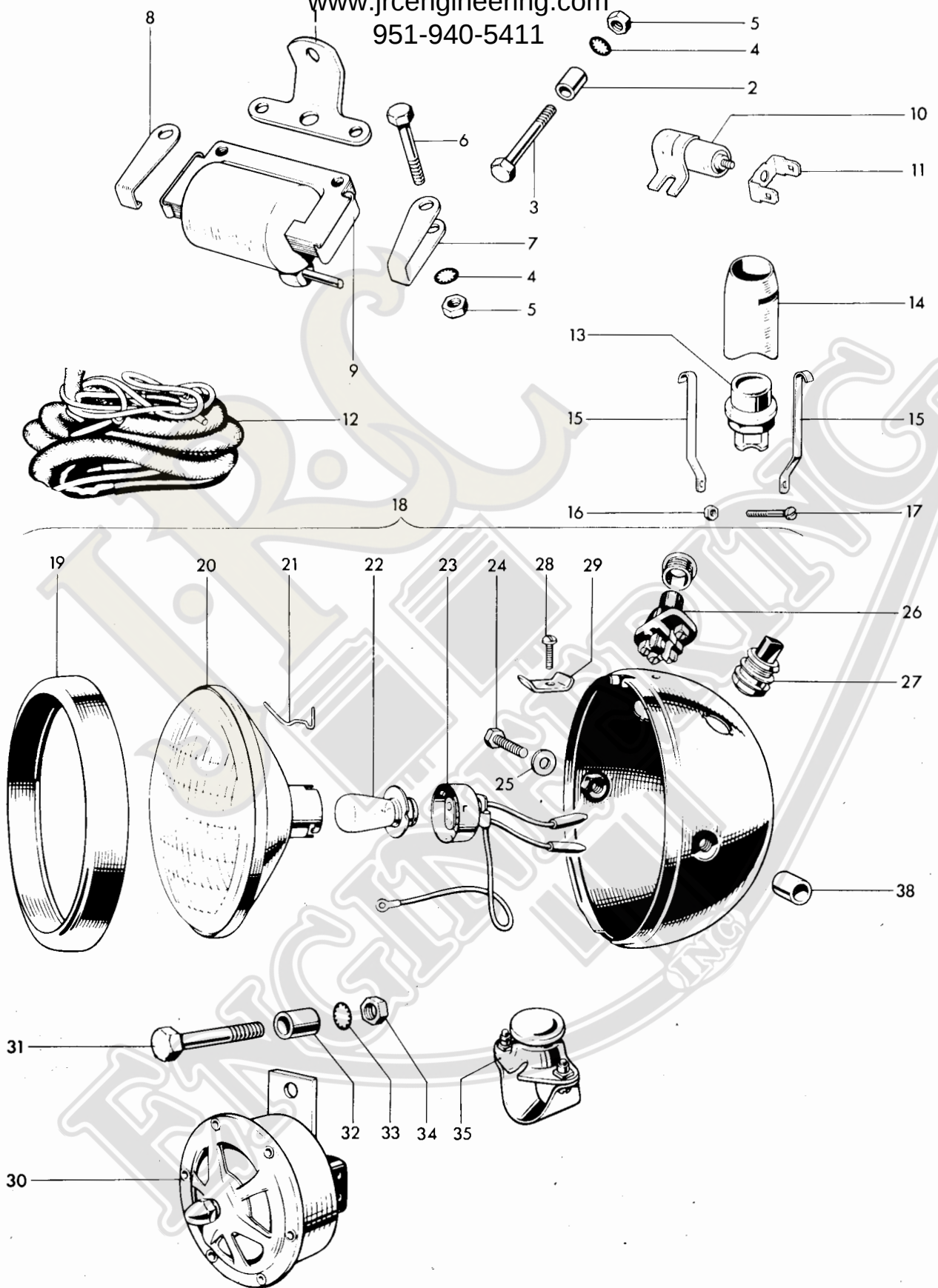
Fig. 32. A.C. MAGNETO IGNITION SYSTEM AND DIRECT LIGHTING www.jrcengineering.com 951-940-5411
