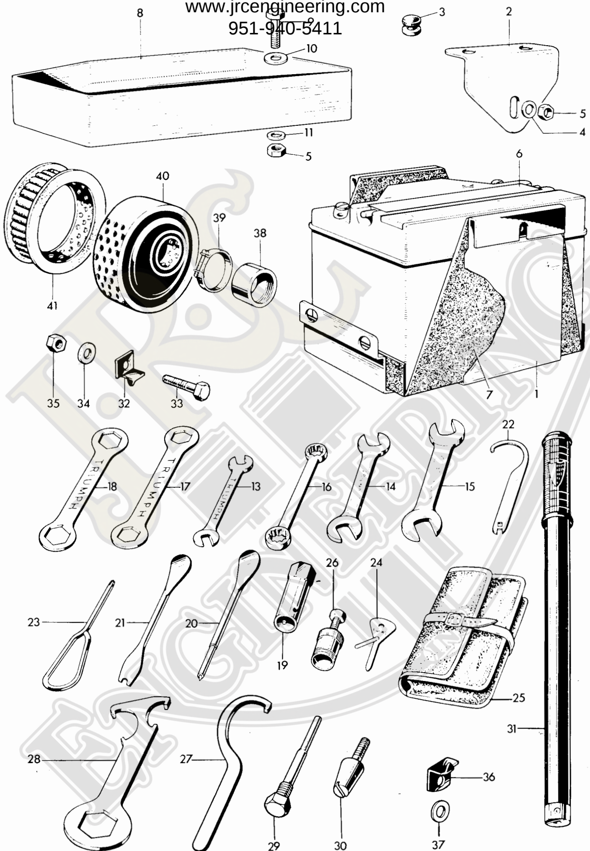
Fig. 27 BATTERY TOOLKIT AND AIR FILTER www.jrcengineering.com 951-940-5411
