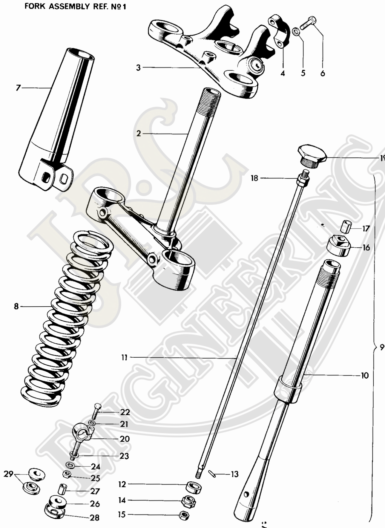
Fig. 18. TELESCOPIC FRONT FORK, U.S.A. T100C AND T100R
