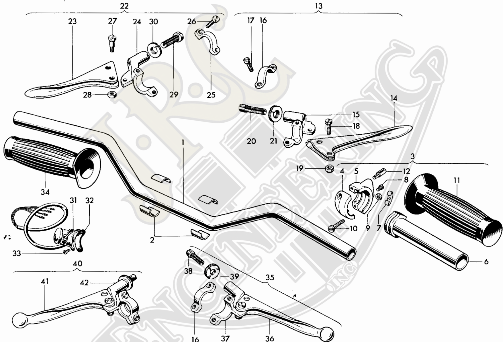
Fig. 27. HANDLEBARS AND CONTROL LEVERS www.jrcengineering.com 951-940-5411
