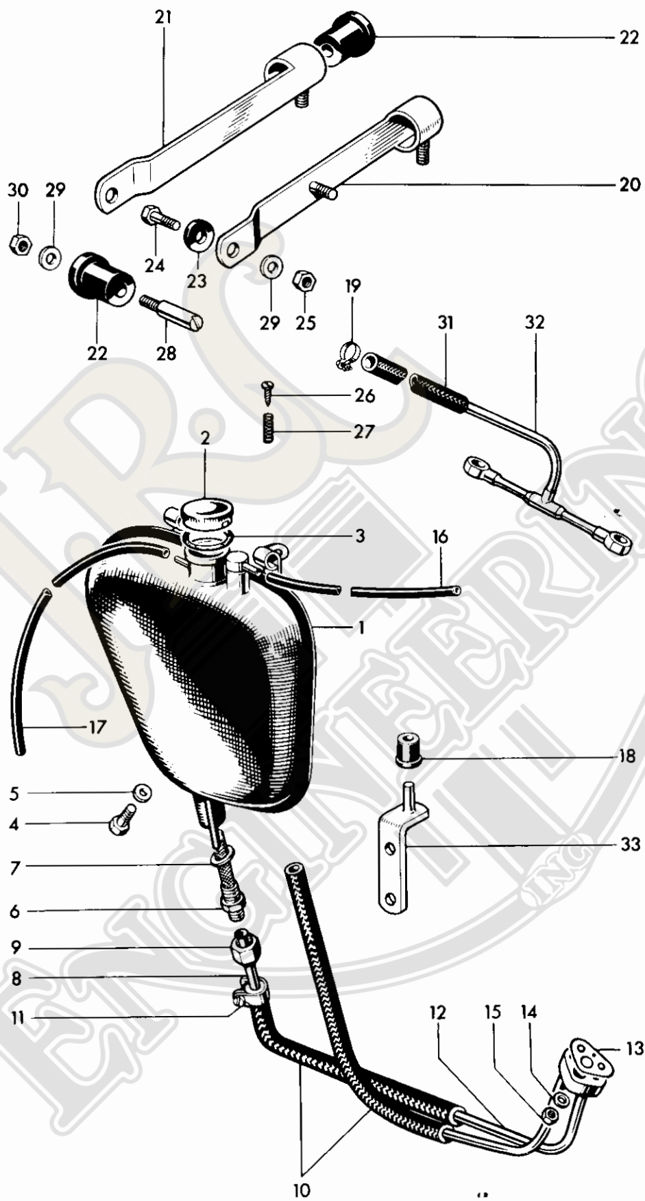
Fig. 25. OIL TANK
