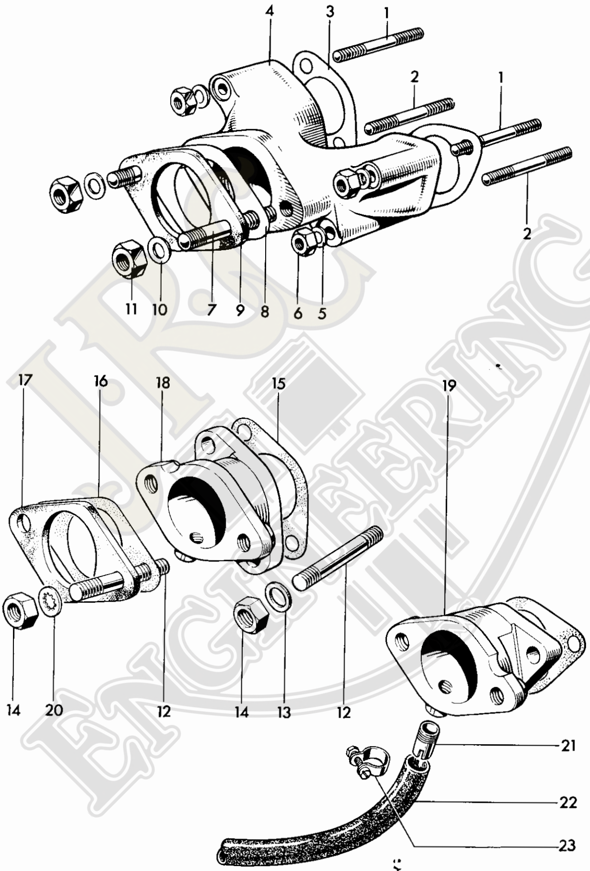
Fig. 4. INLET MANIFOLDS
