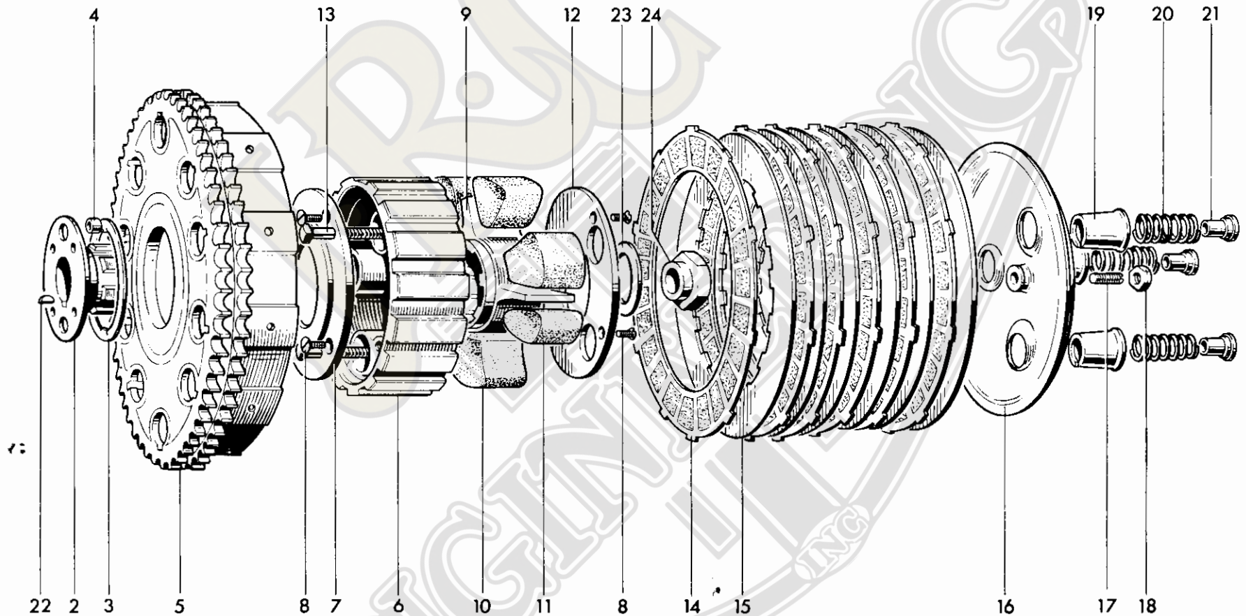
CLUTCH ASSEMBLY № 1
