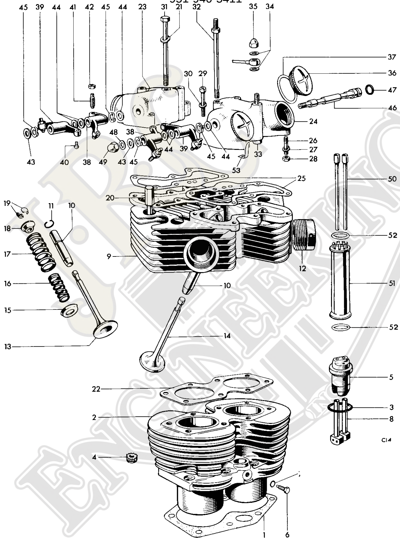
Fig. 6. CYLINDER BLOCK AND HEAD T1000 AND T100C
