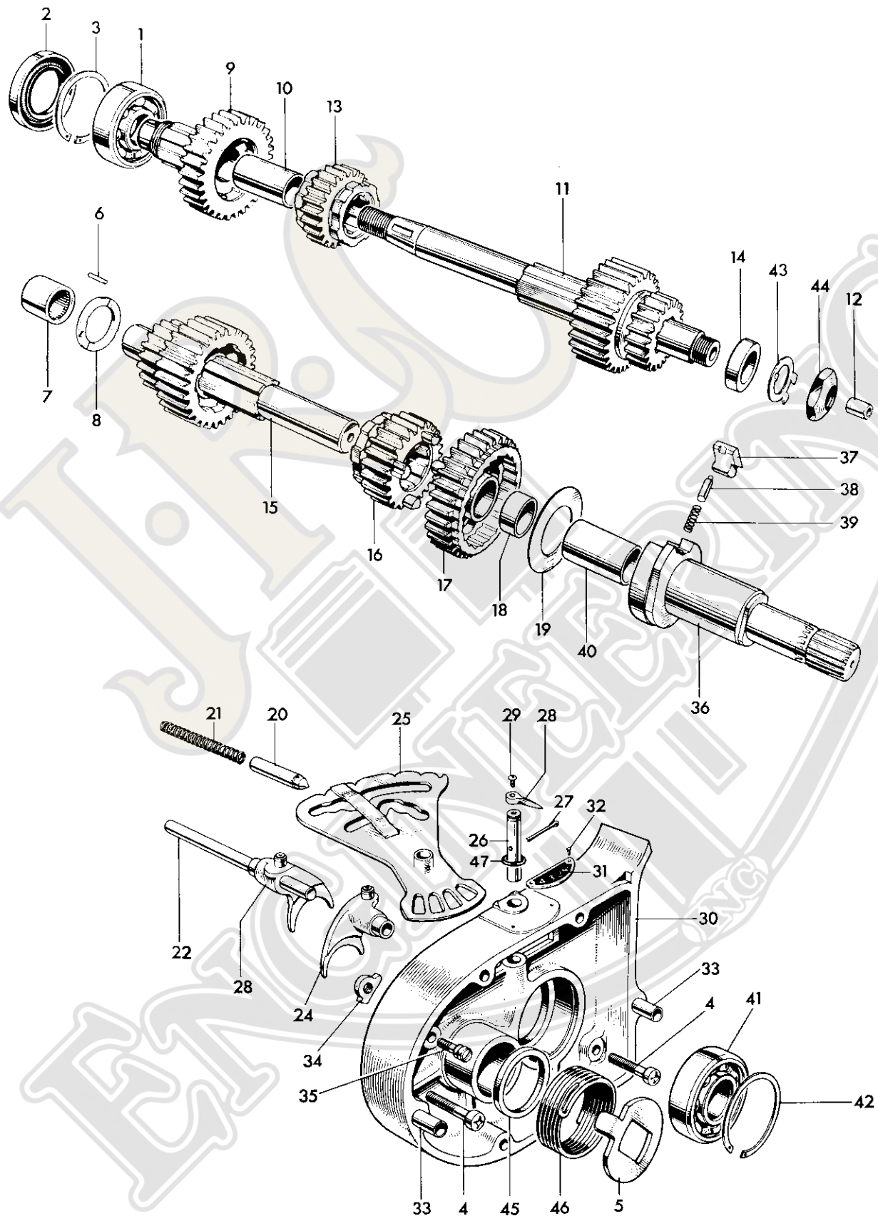
Fig. 9. GEARBOX WITH GEAR COVER AND INNER COVER
