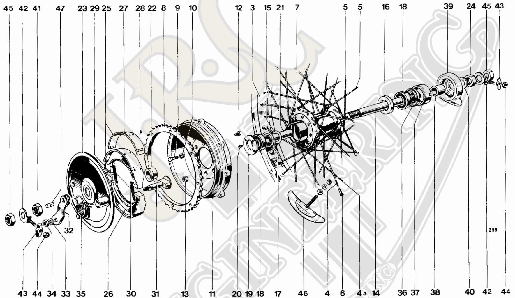
Fig. 21. REAR WHEEL
