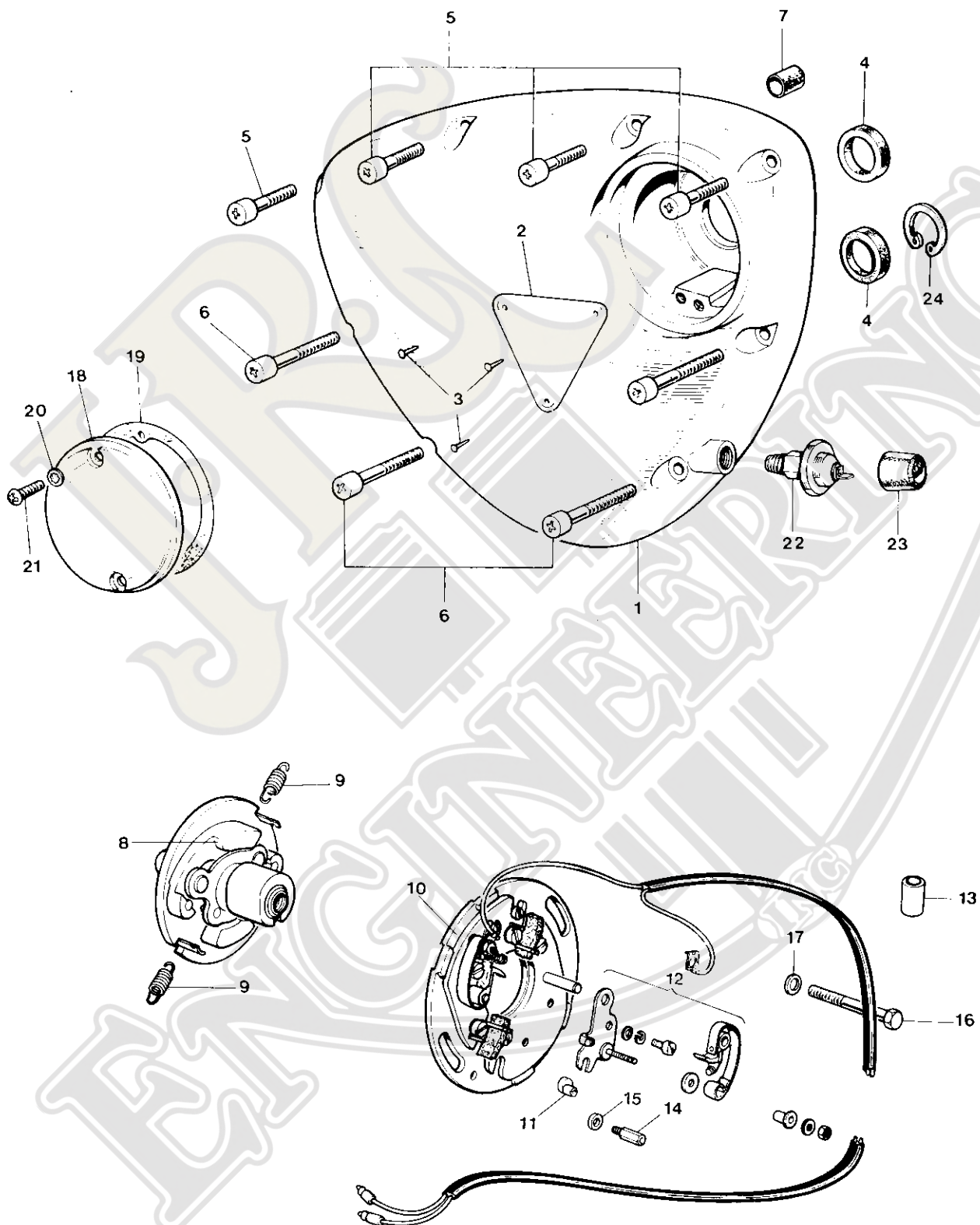
www.jrcengineering.com Fig. 8. TIMING COVER AND CONTACT BREAKER 951-940-5411
