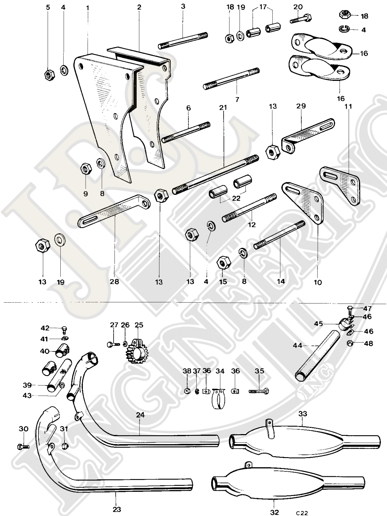
Fig. 13. ENGINE FITTINGS AND EXHAUST SYSTEM www.jrcengineering.com 951-940-5411
