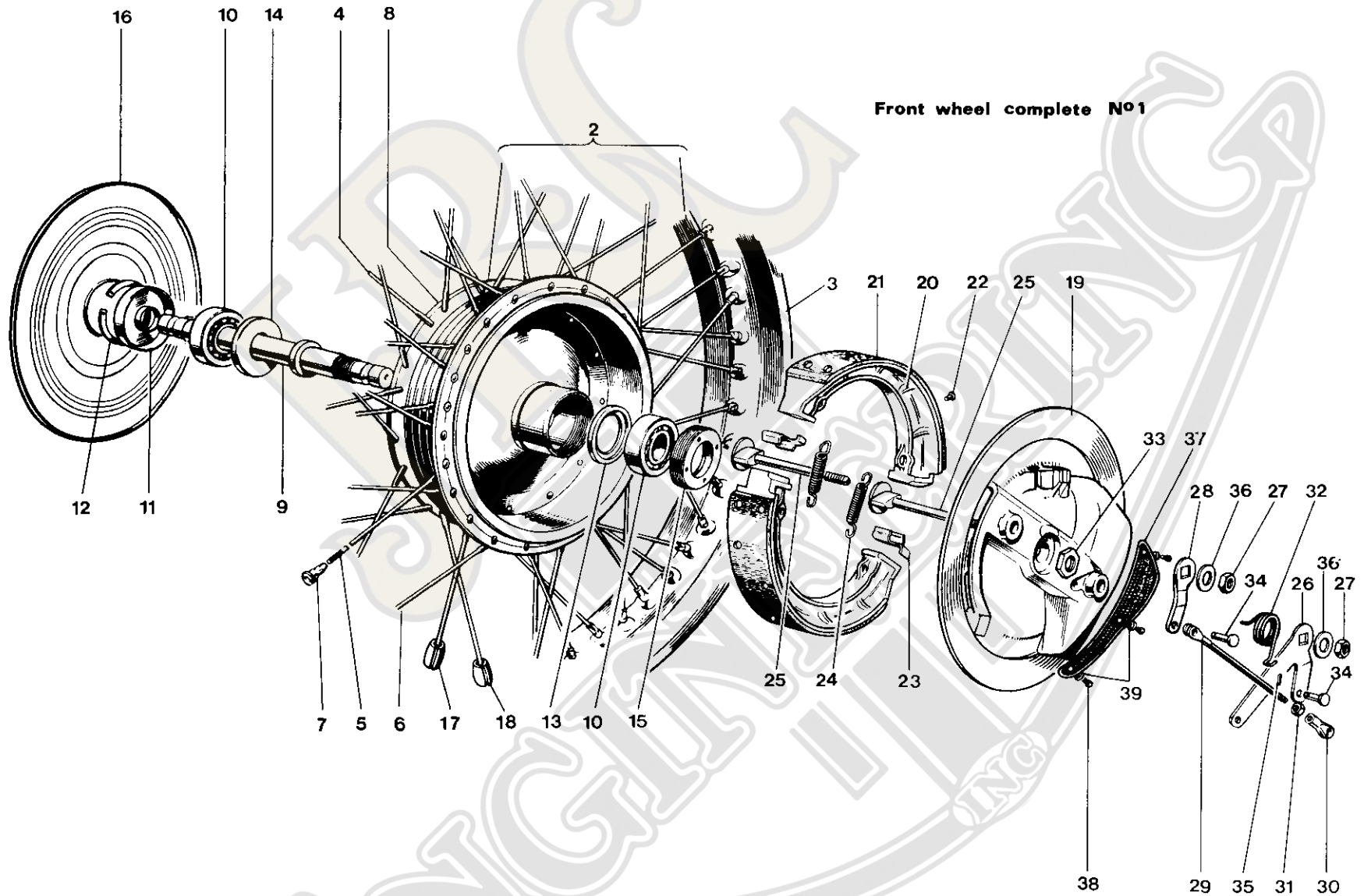
Fig. 19. FRONT WHEEL T100T, T100R
