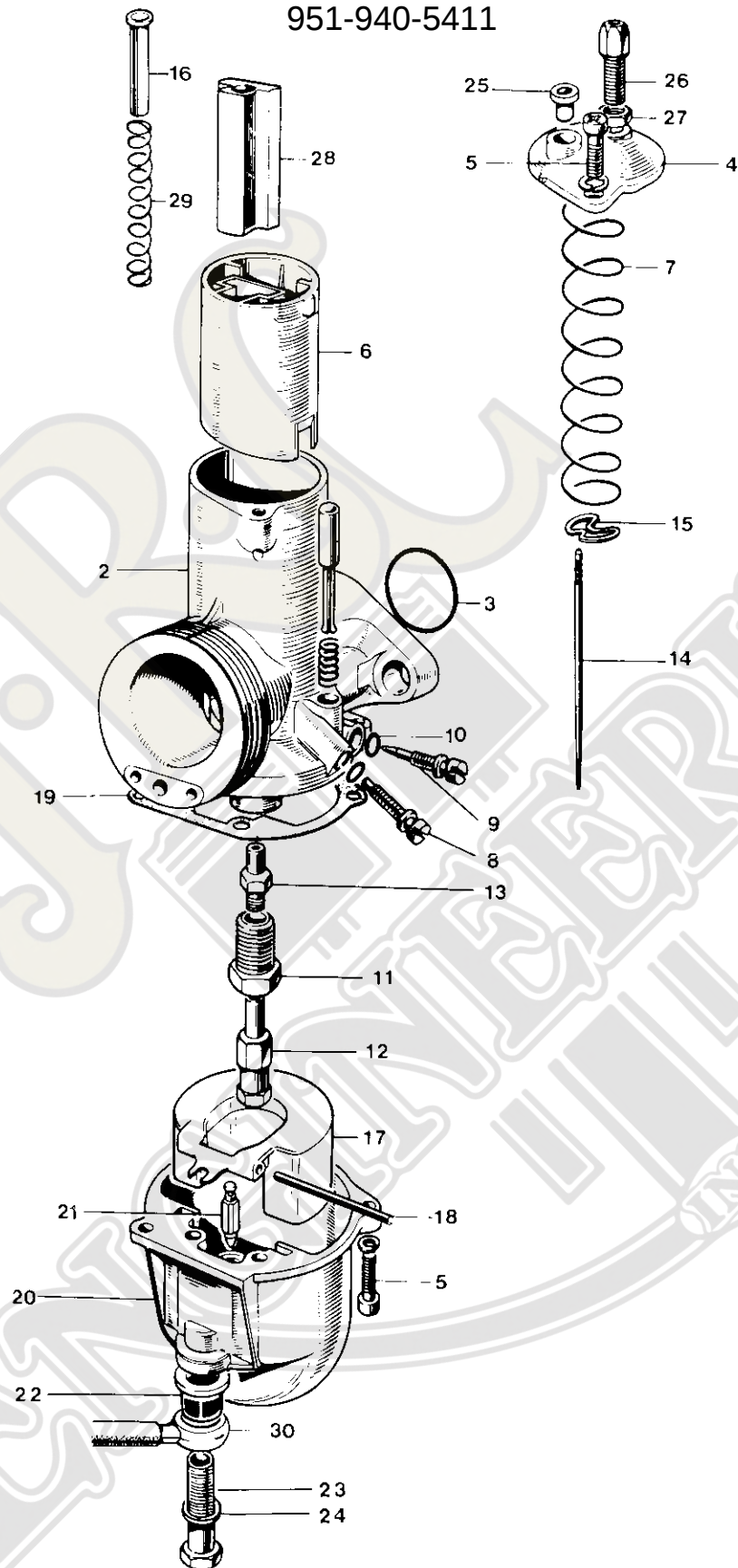
Fig. 31 CARBURETOR T100T AND T100R
