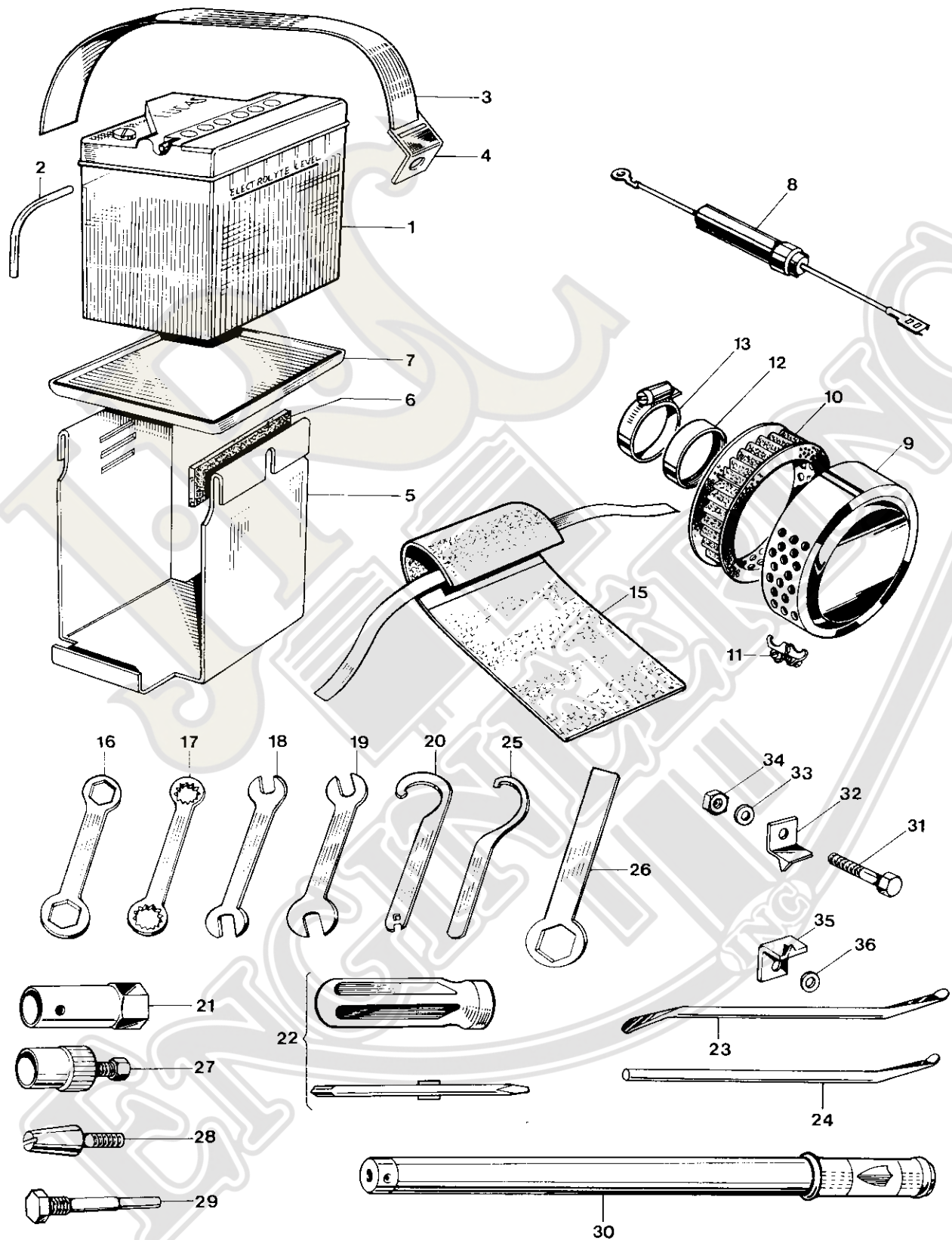
Fig. 27. BATTERY, TOOLKIT AND AIR FILTER www.jrcengineering.com 951-940-5411
