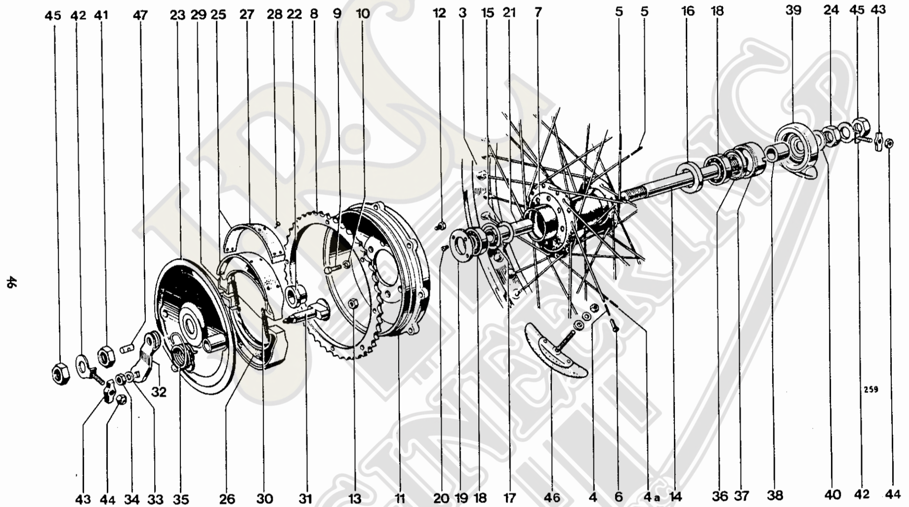
Fig. 21. REAR WHEEL
