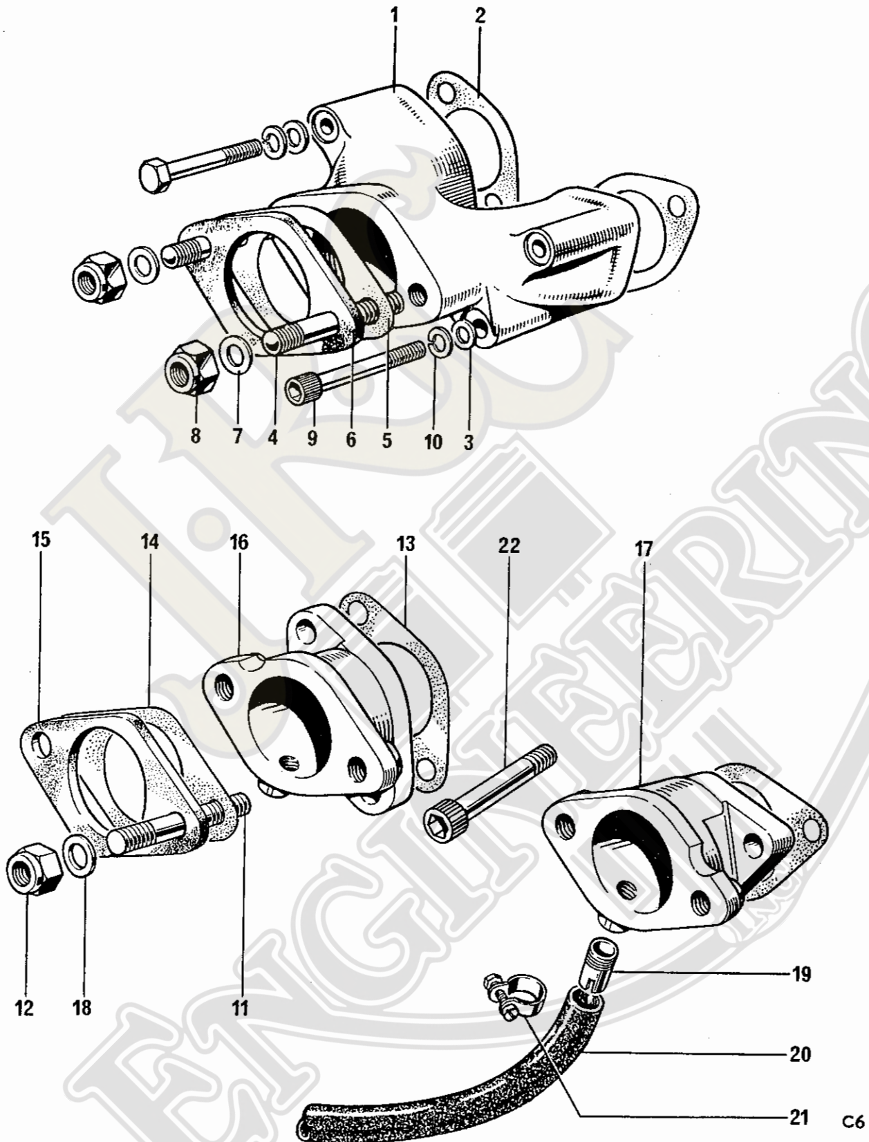
Fig. 4. INLET MANIFOLDS
