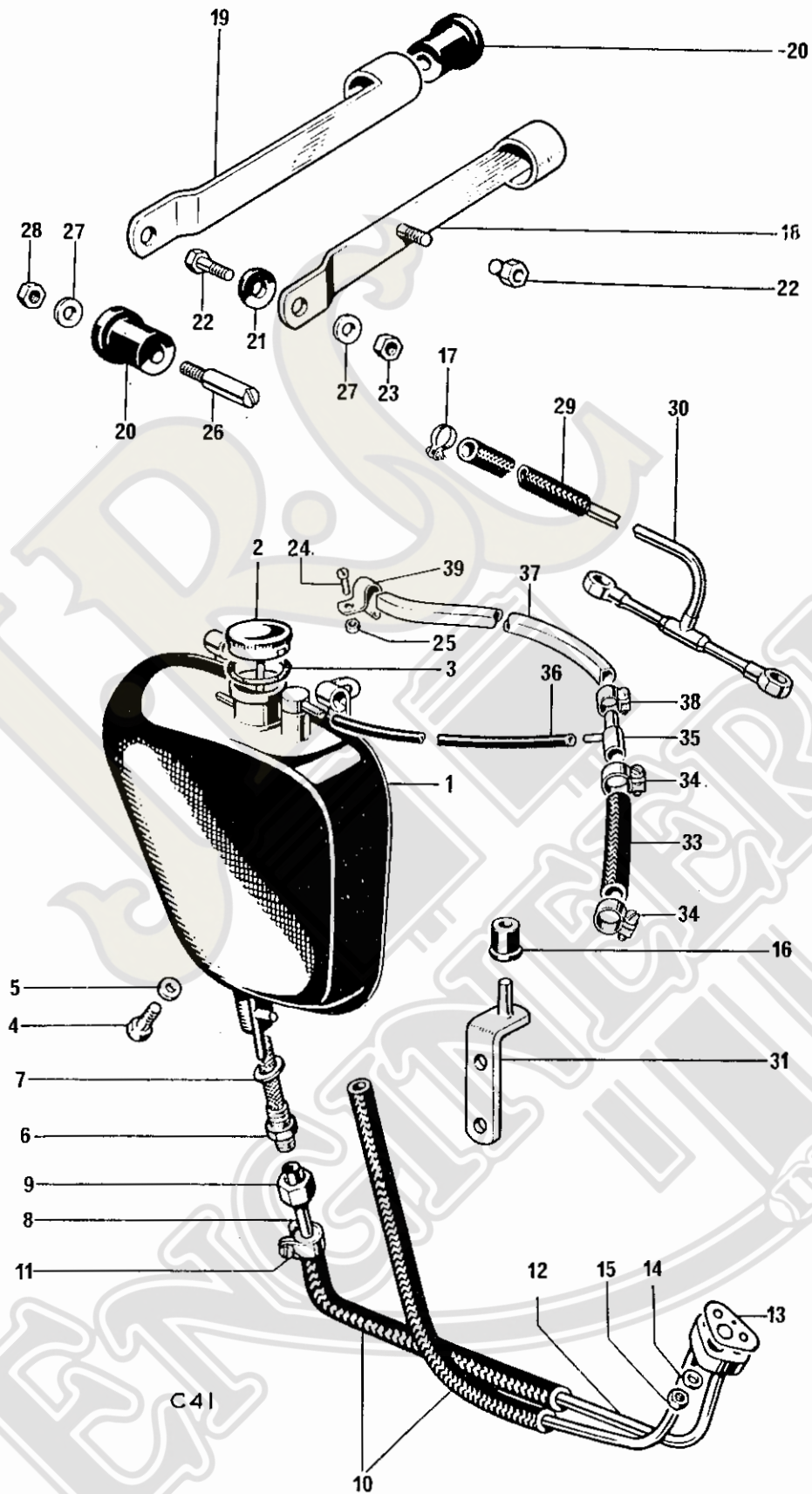
Fig. 26. OIL TANK
