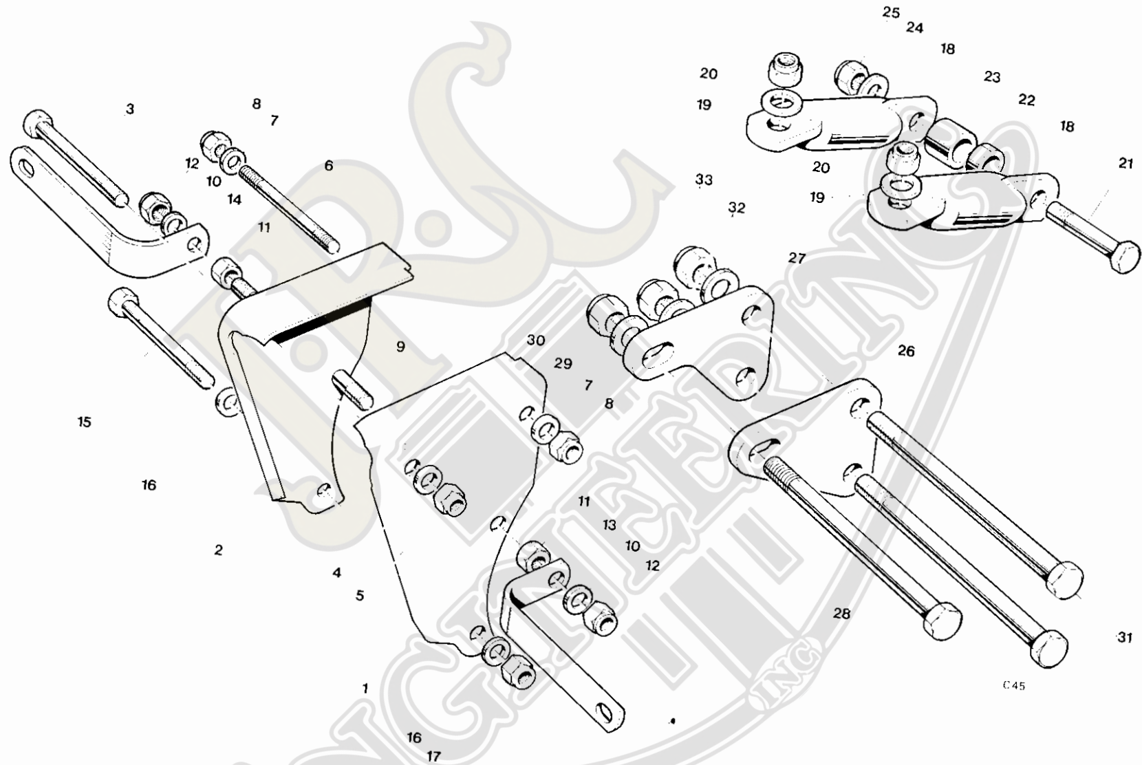
Fig. 16. MOTOR FITTINGS
