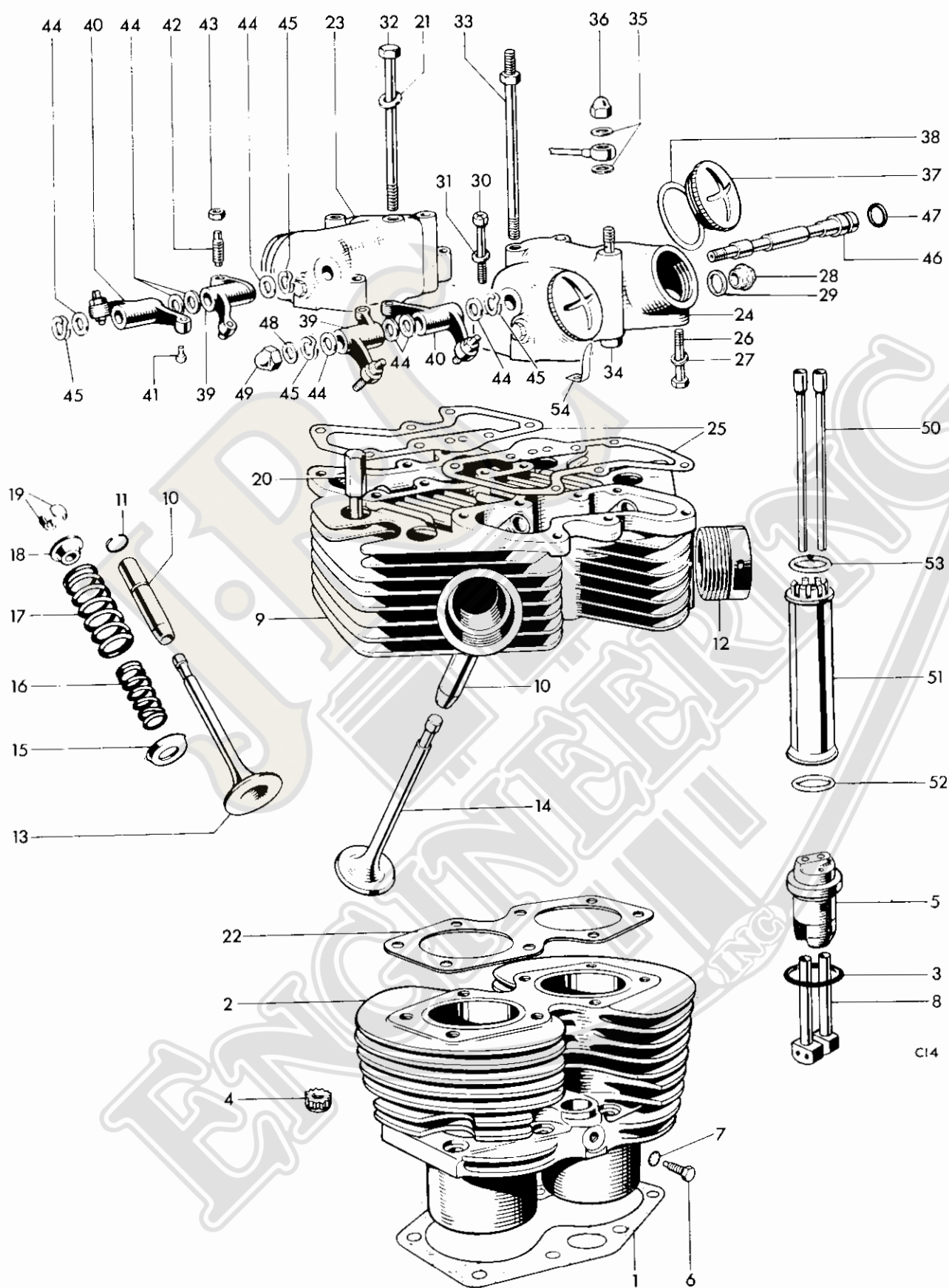
Fig. 7. CYLINDER BLOCK AND HEAD, T100R
