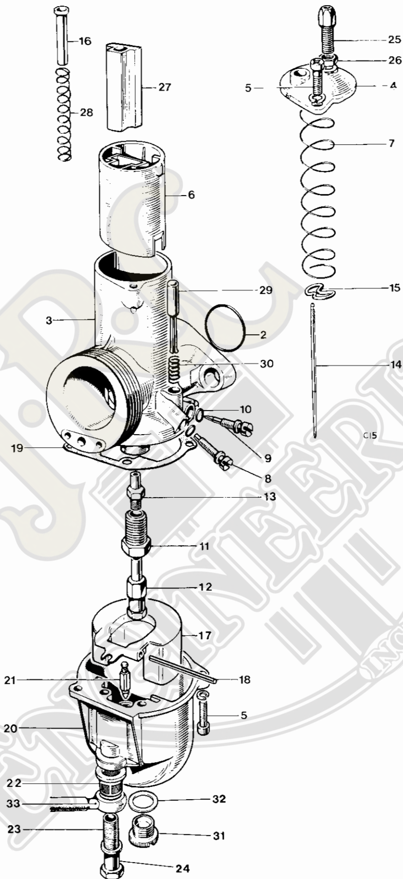
Fig. 5. CARBURETOR T100C
