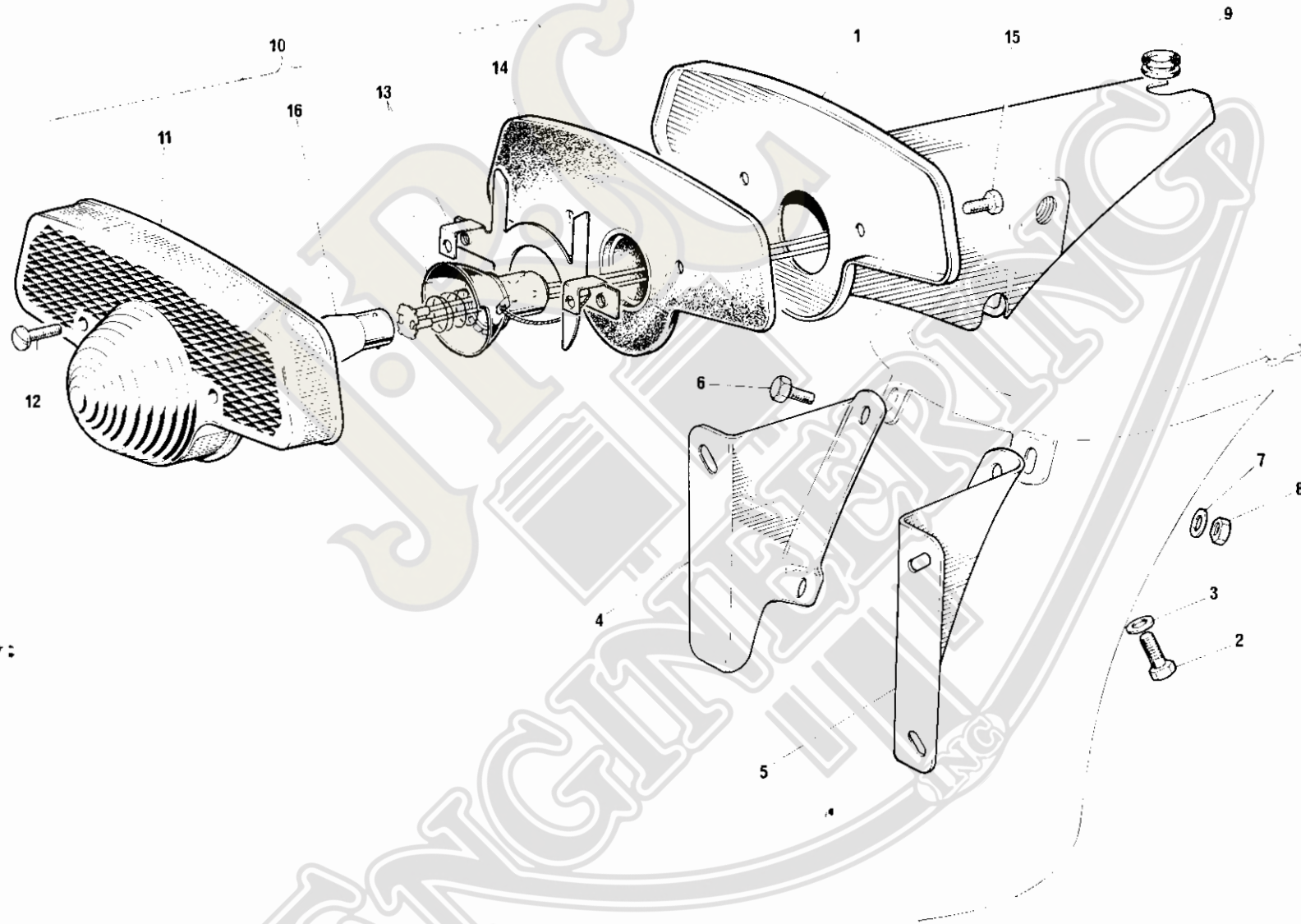
Fig. 25. TAIL LAMP AND SUPPORT
