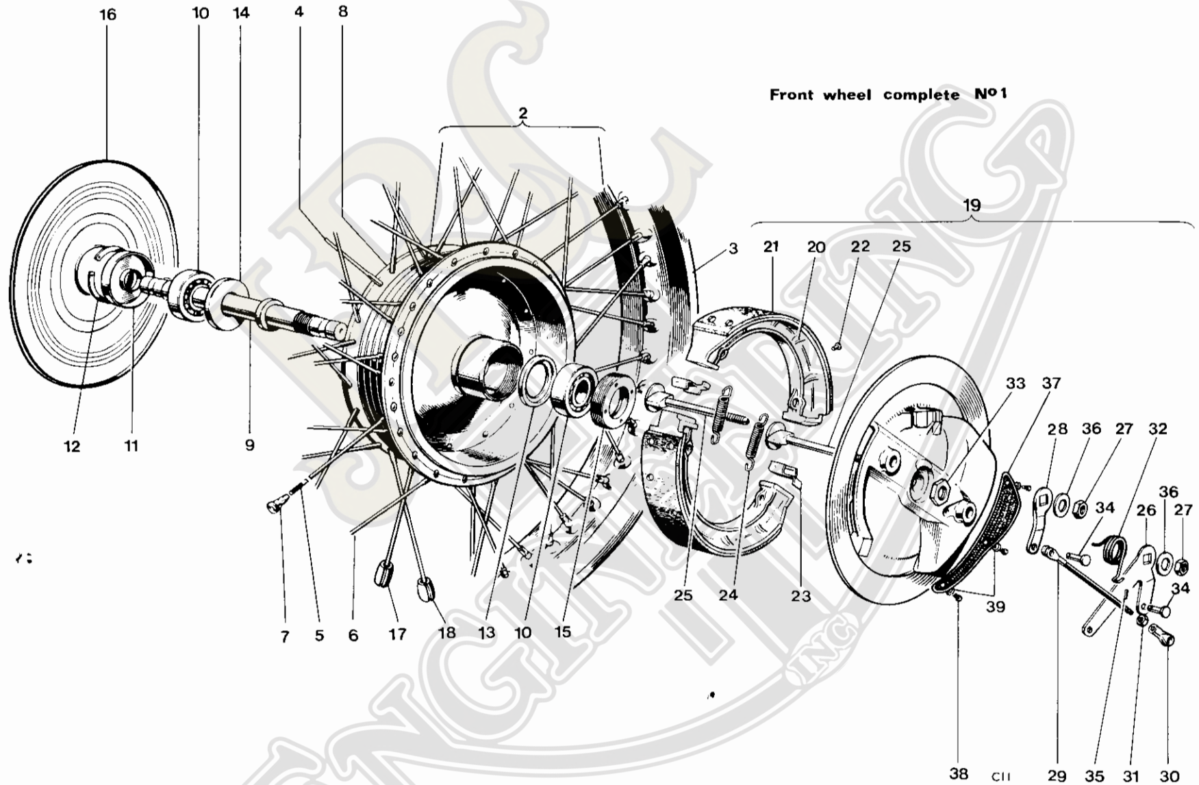
Fig. 22. FRONT WHEEL T100C
