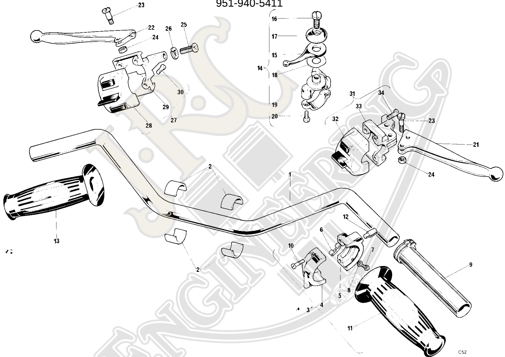
Fig. 30. HANDLEBAR AND CONTROL LEVERS www.jrcengineering.com 951-940-5411
