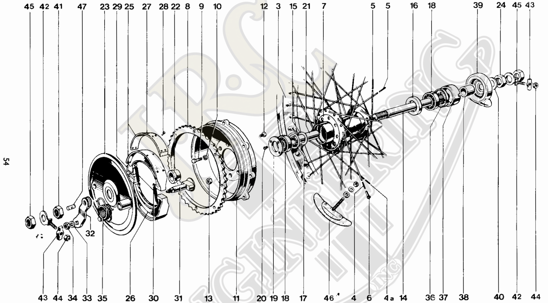
Fig. 32. REAR WHEEL
