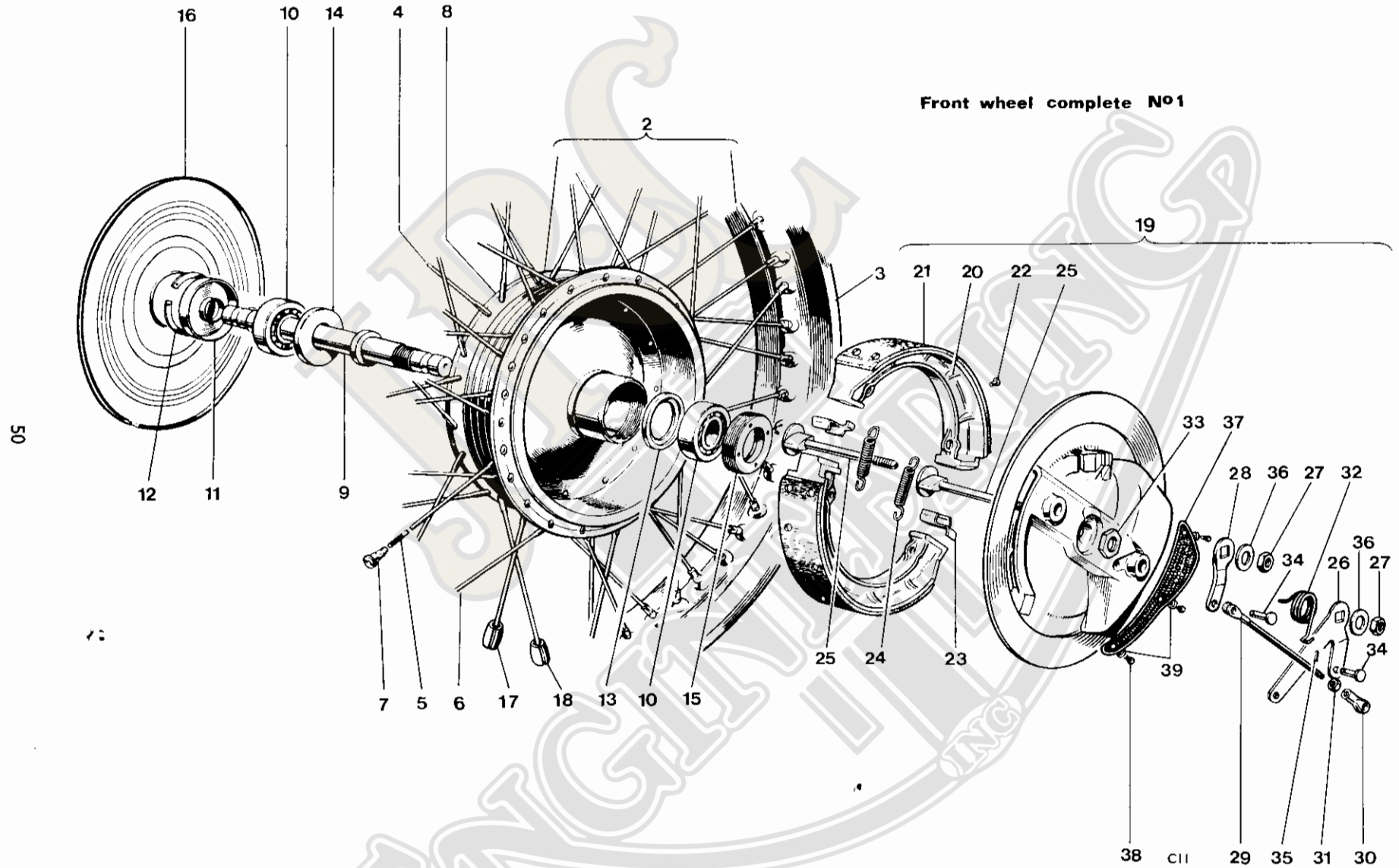
Fig. 21. FRONT WHEEL T100R
