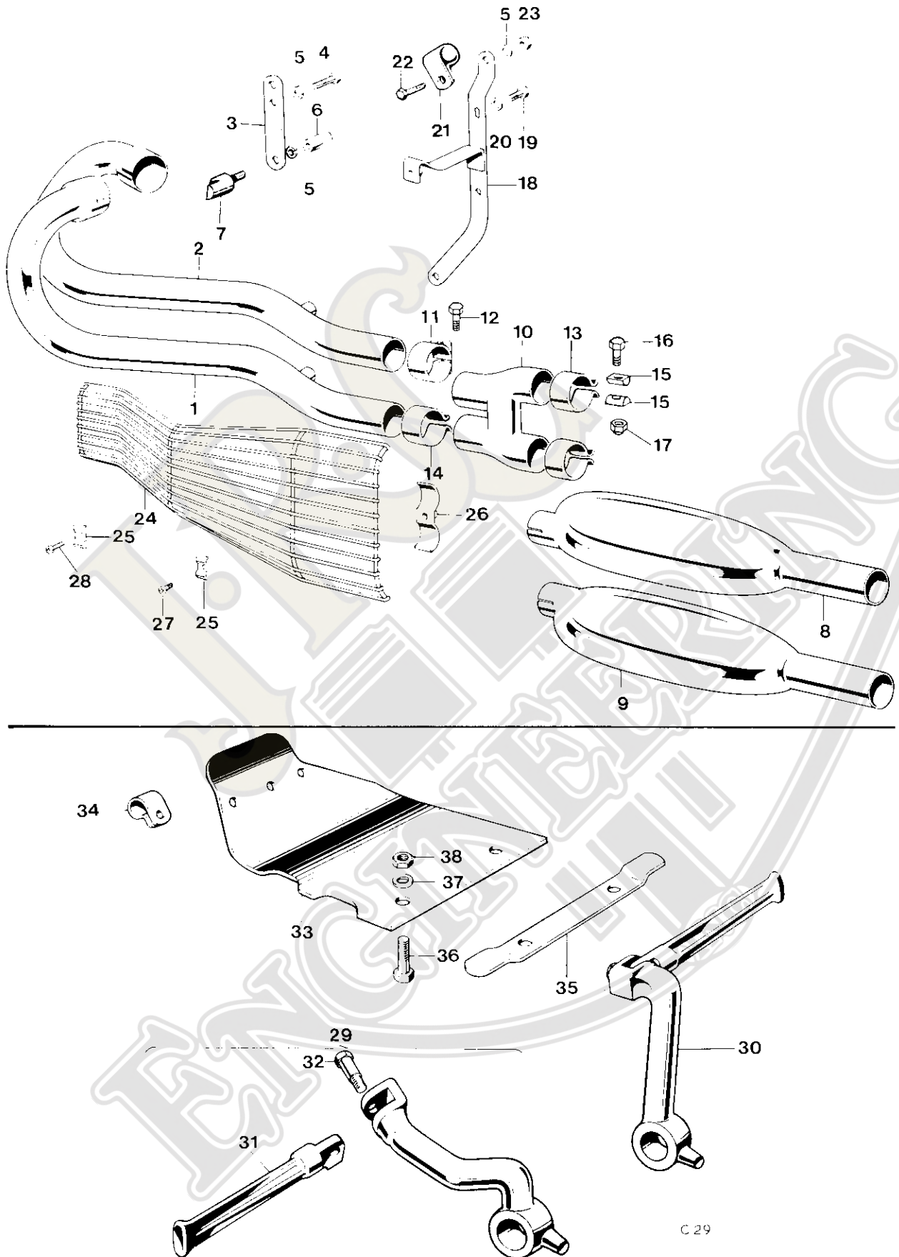
Fig. 17. EXHAUST PIPES, UNDERSHIELD AND FOOTPEGS (T100C)
