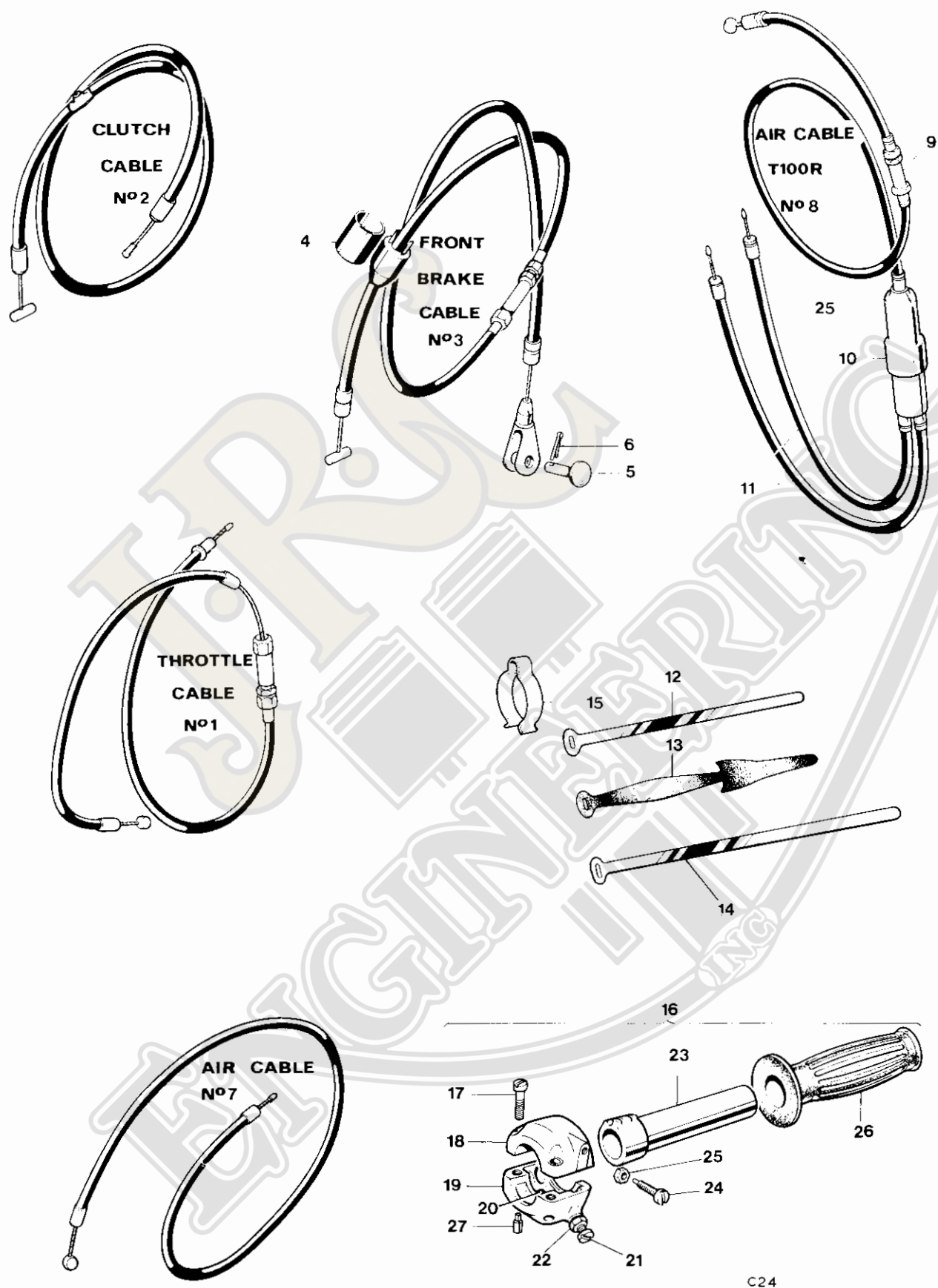
Fig. 32. CONTROL CABLES
