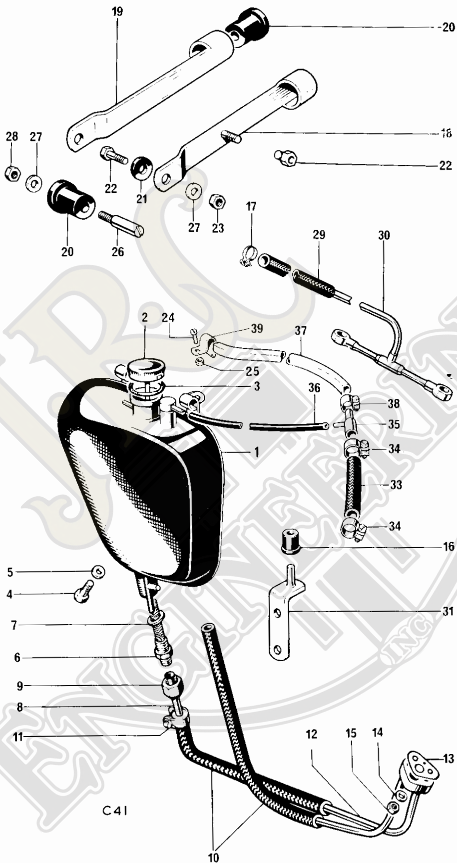
Fig. 28. OIL TANK
