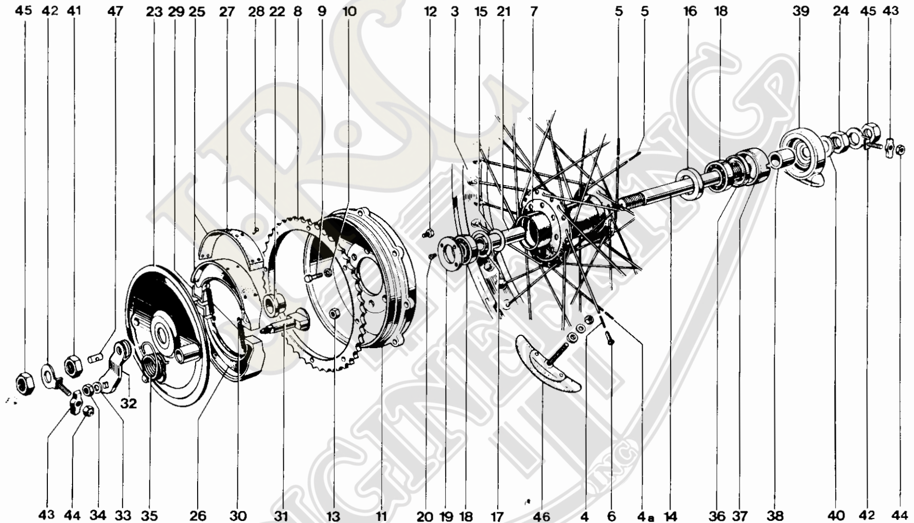
Fig. 18. REAR WHEEL
