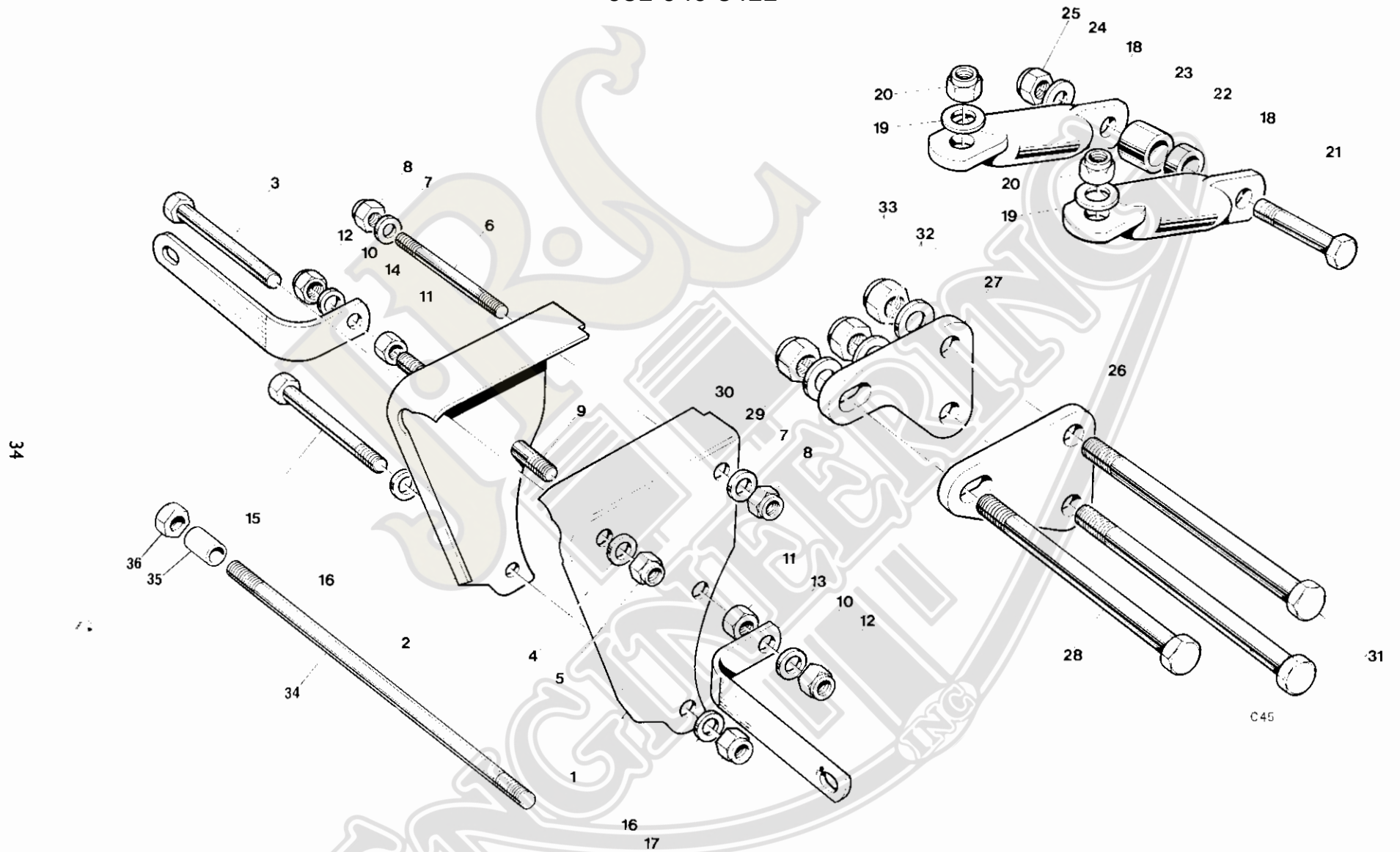
Fig. 13. MOTOR FITTINGS
