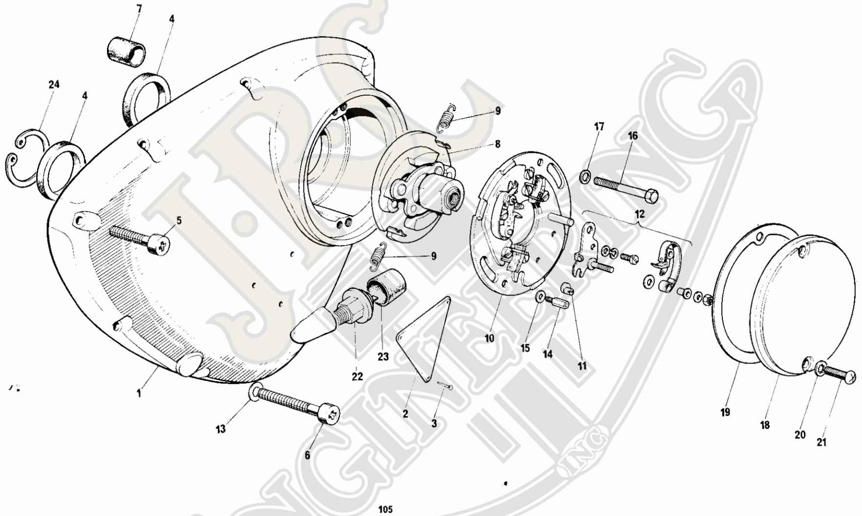
Fig. 7. TIMING COVER AND CONTACT BREAKER
