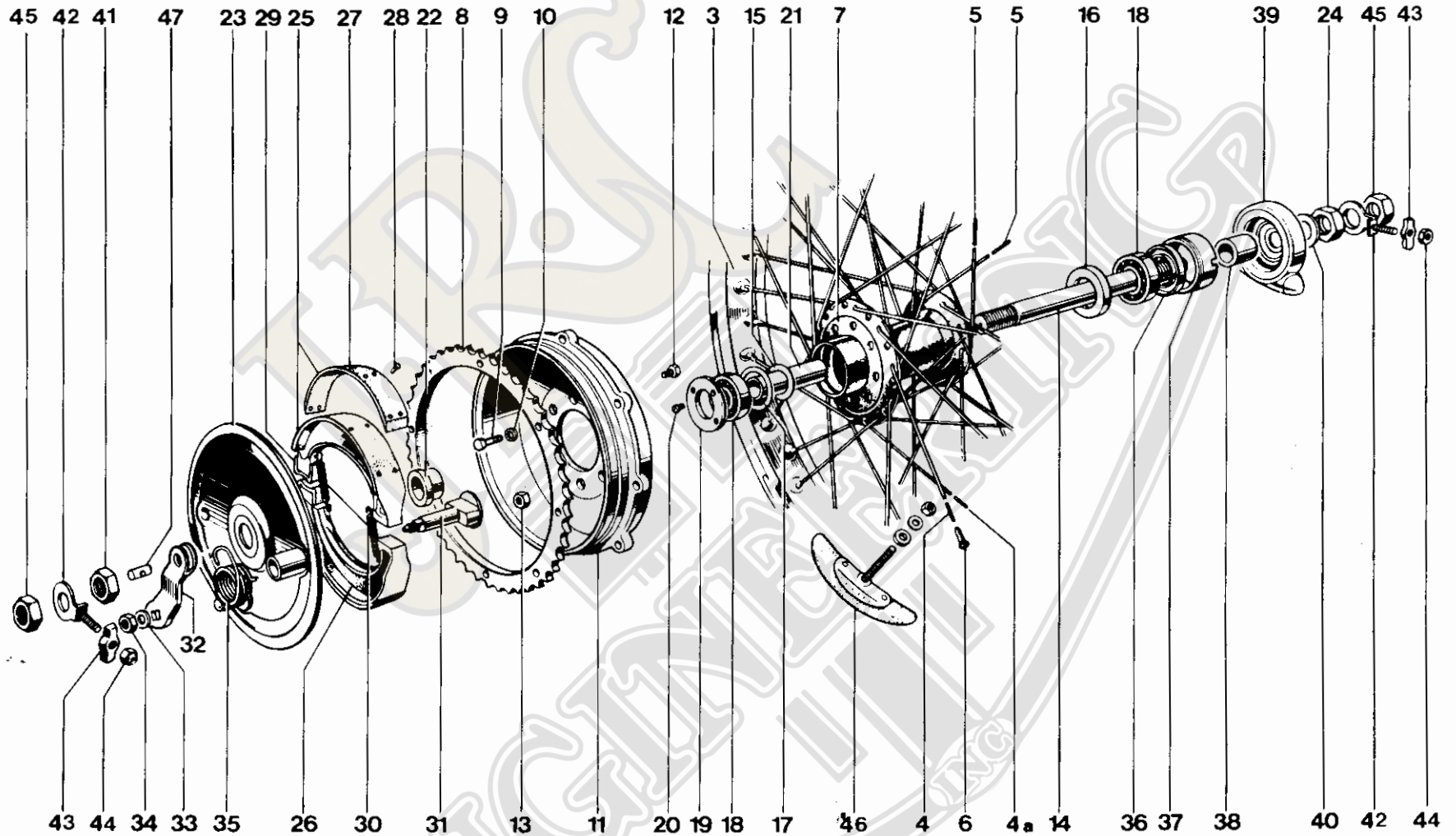
Fig. 18. REAR WHEEL
