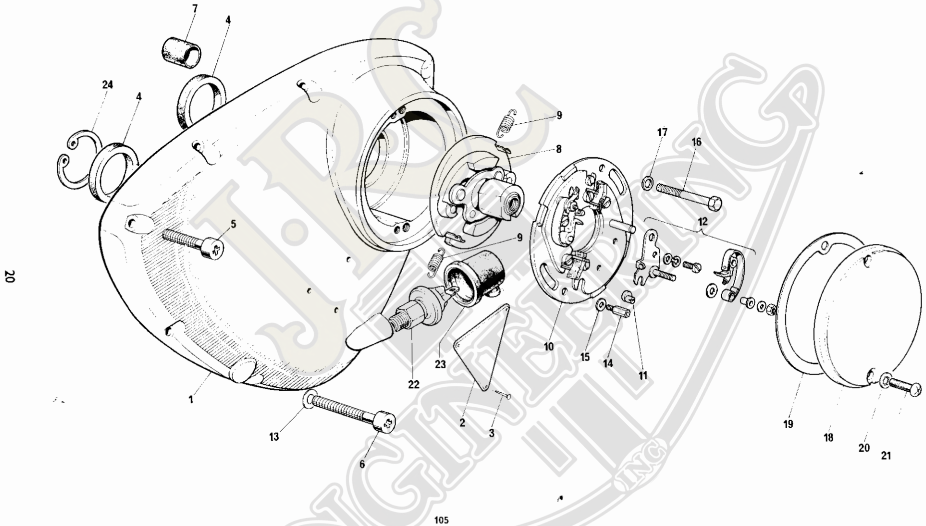
Fig. 7. TIMING COVER AND CONTACT BREAKER
