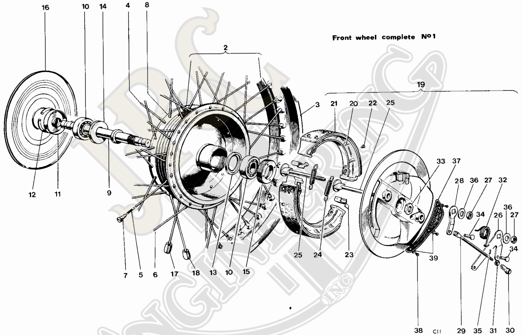
Fig. 17. FRONT WHEEL
