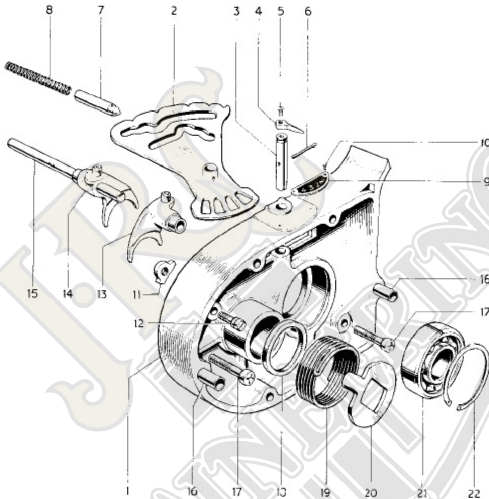
FIG. 7 GEARBOX INNER COVER
