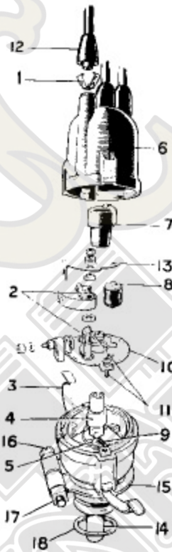
FIG. 20 LUCAS DISTRIBUTOR TYPE 18D2
