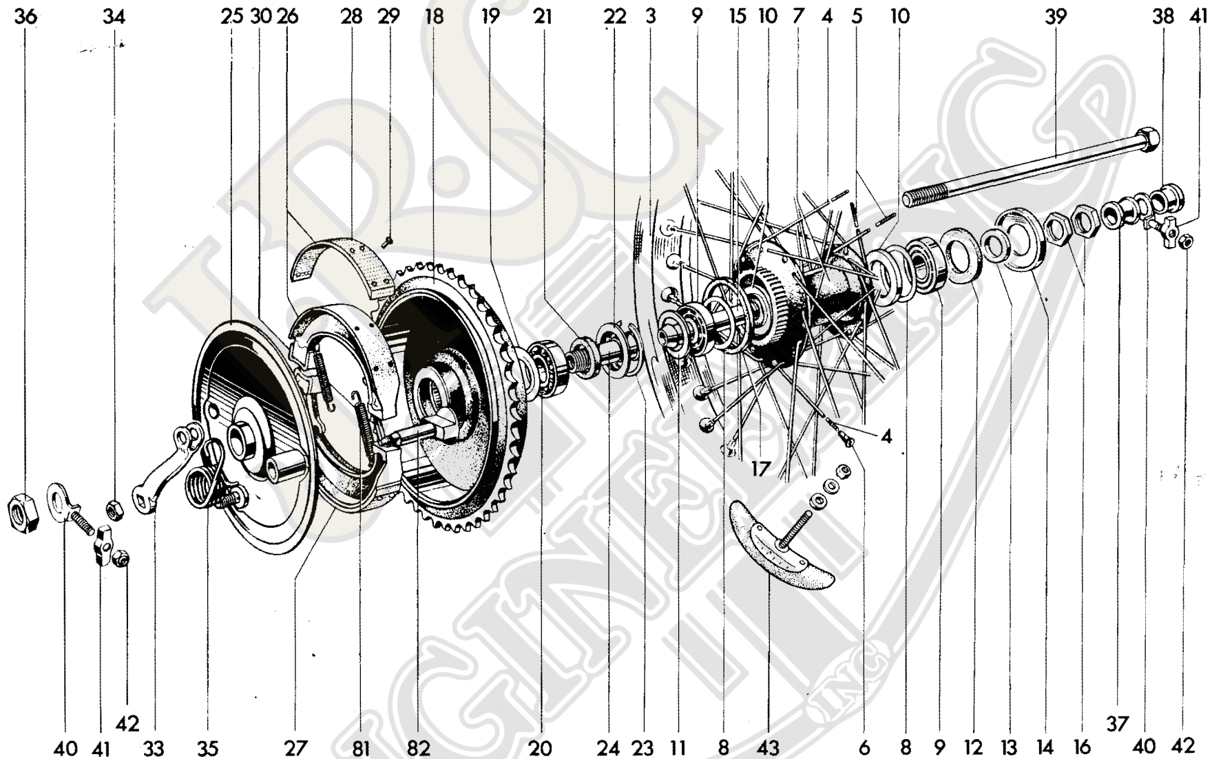
Fig. 21. QUICKLY DETACHABLE REAR WHEEL
