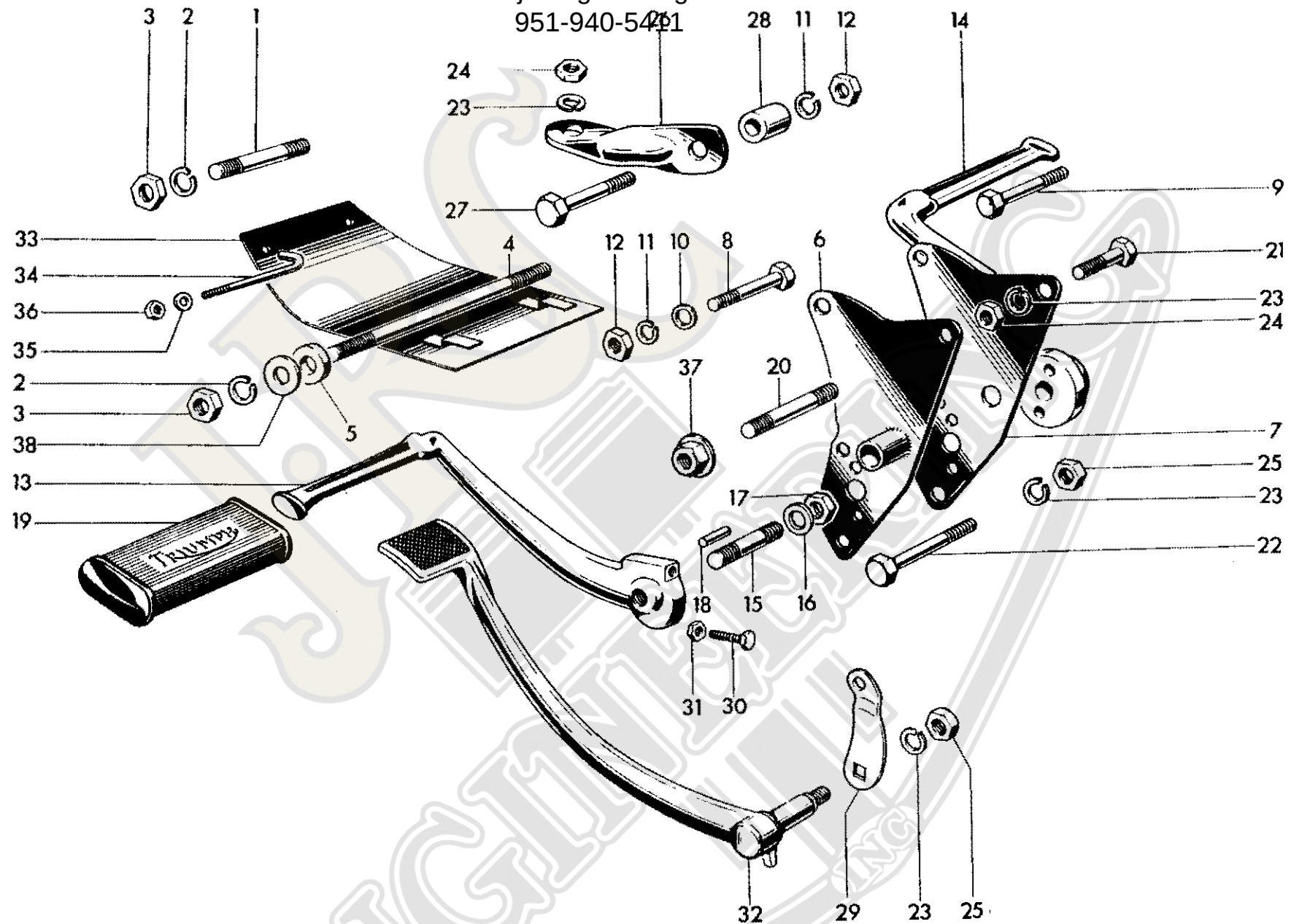
Fig. 14. ENGINE UNIT FITTINGS AND FOOTRESTS
