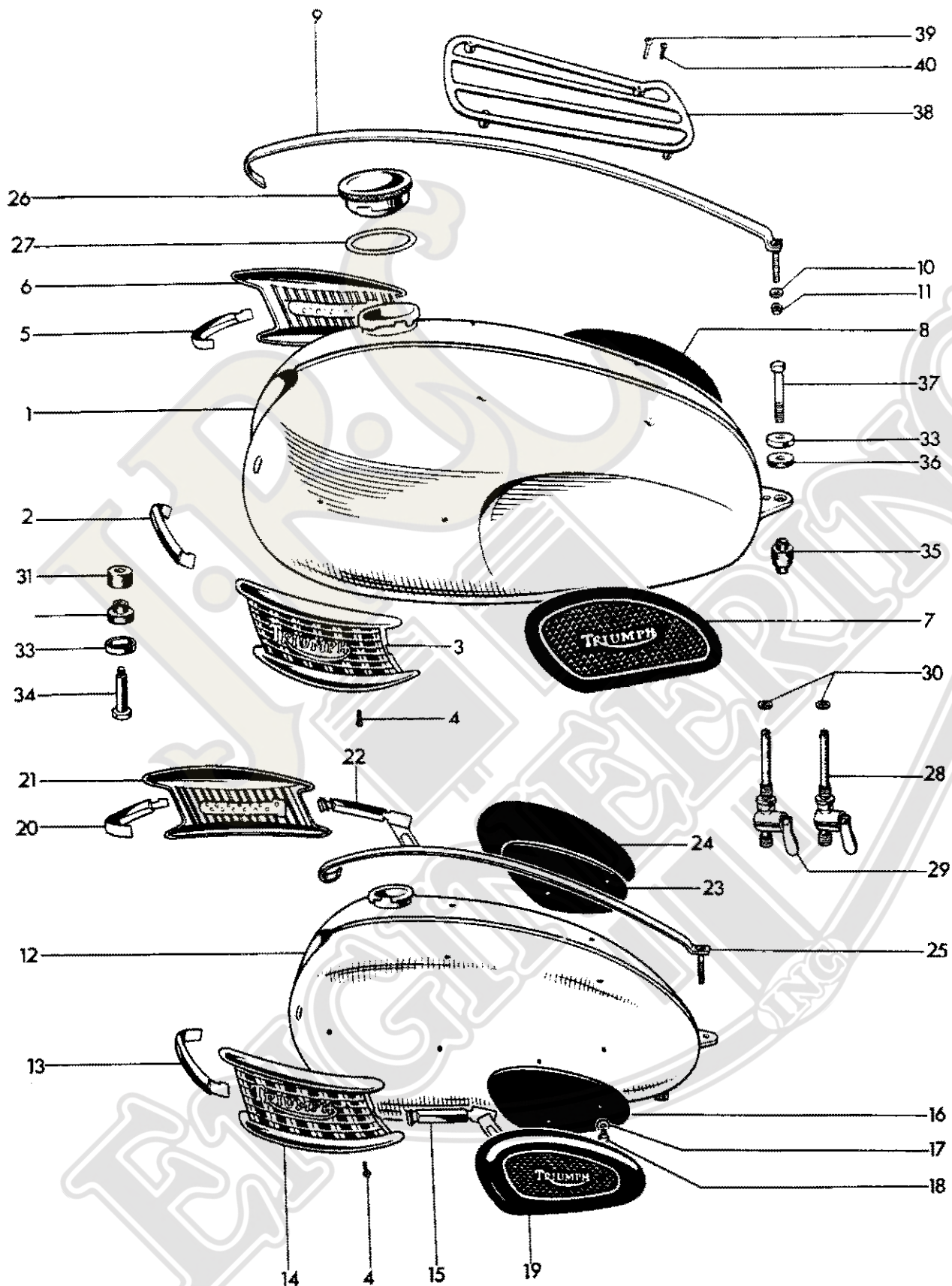
Fig. 22. PETROL TANKS
