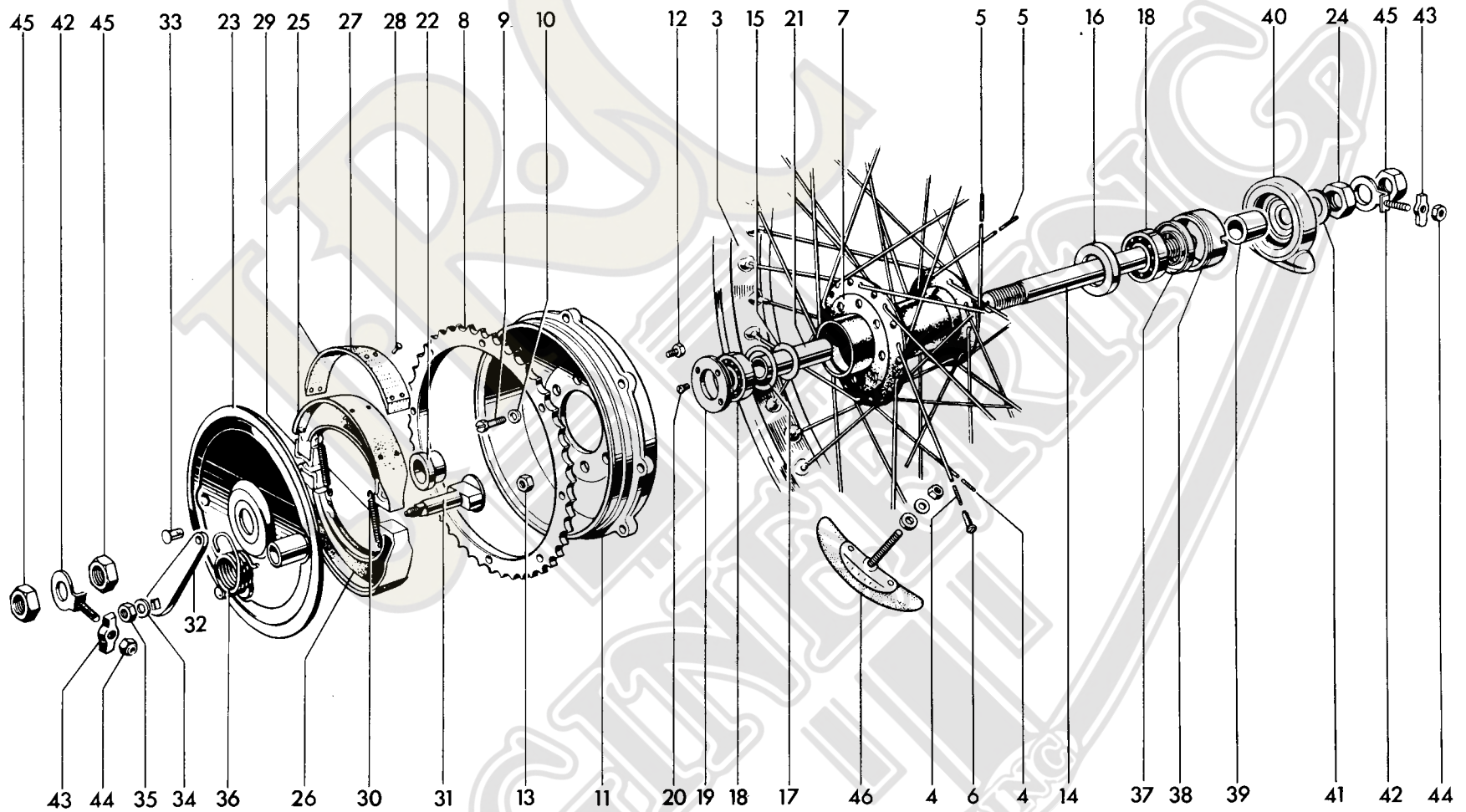
Fig. 23. REAR WHEEL
