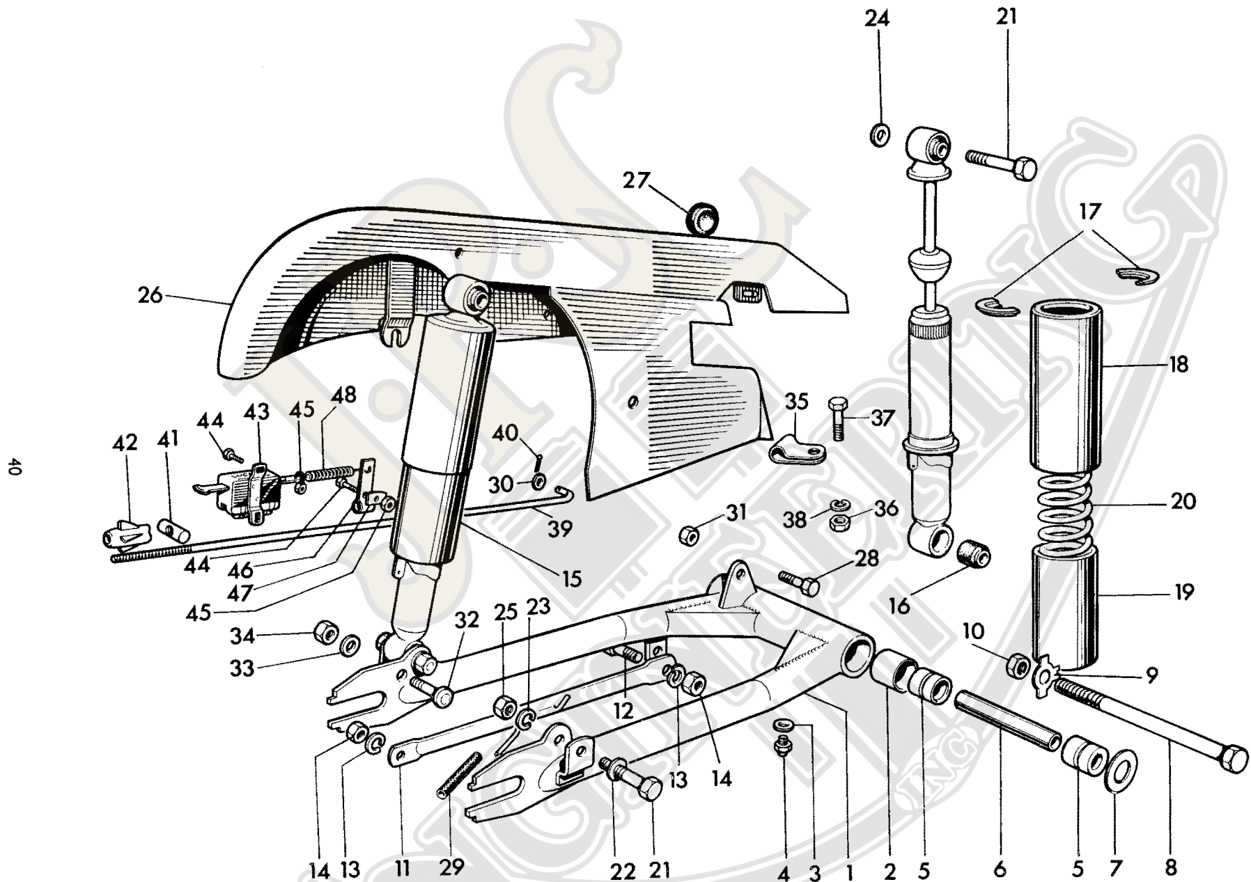
Fig. 13. SWINGING FORK AND SUSPENSION UNITS
