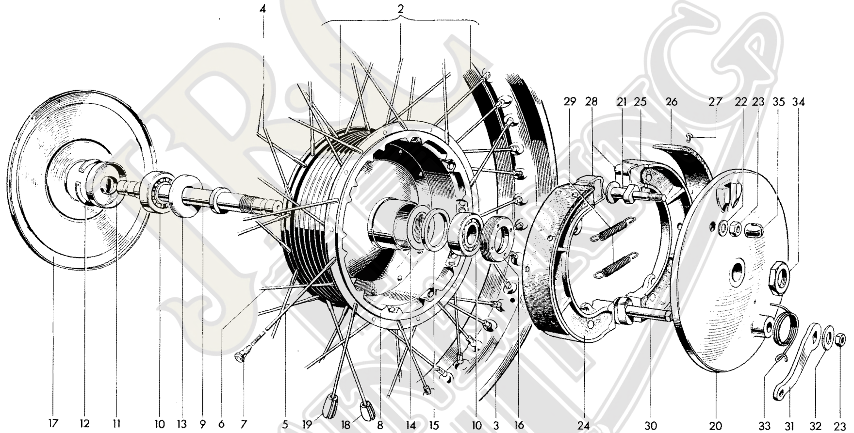
Fig. 19. FRONT WHEEL
