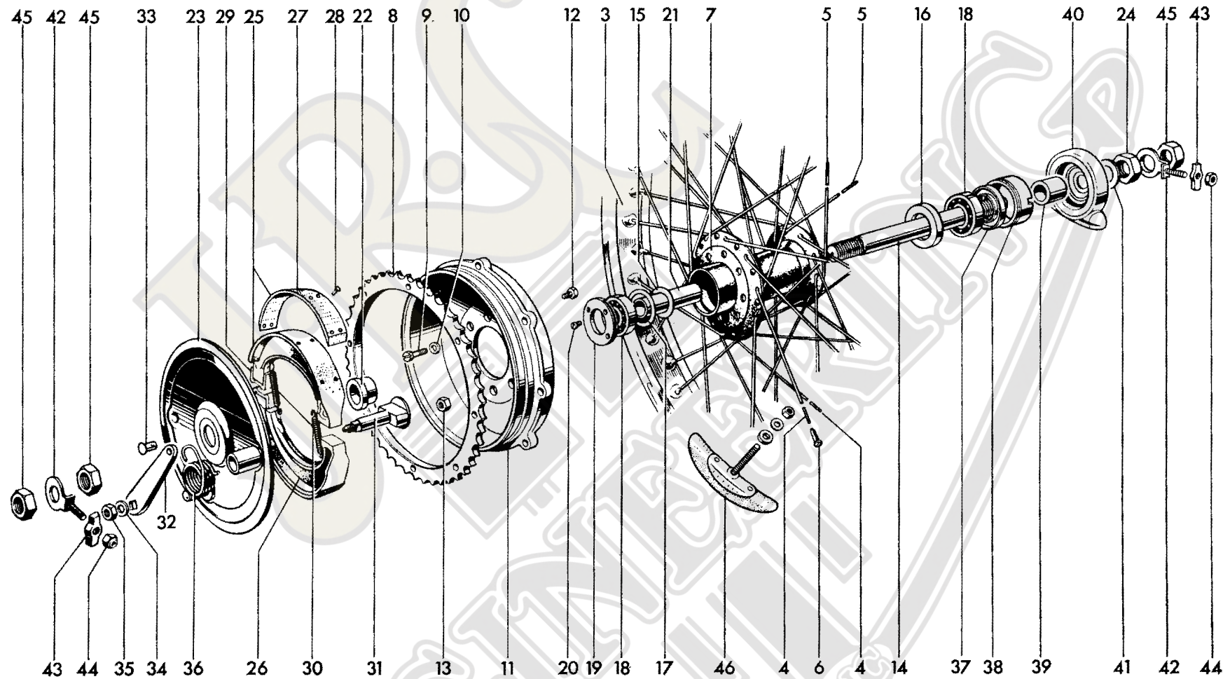
Fig. 20. REAR WHEEL
