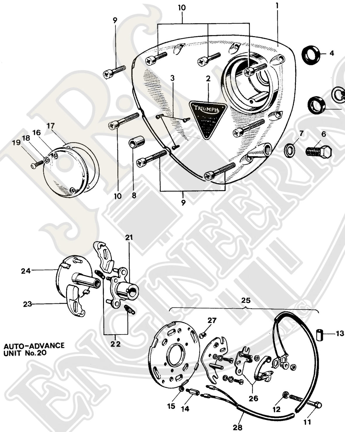
Fig. 6. TIMING COVER AND CONTACT BREAKER
