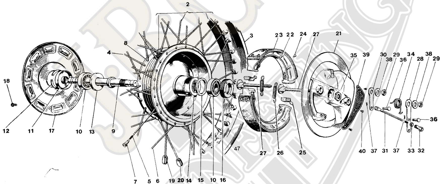
Fig. 19. FRONT WHEEL
