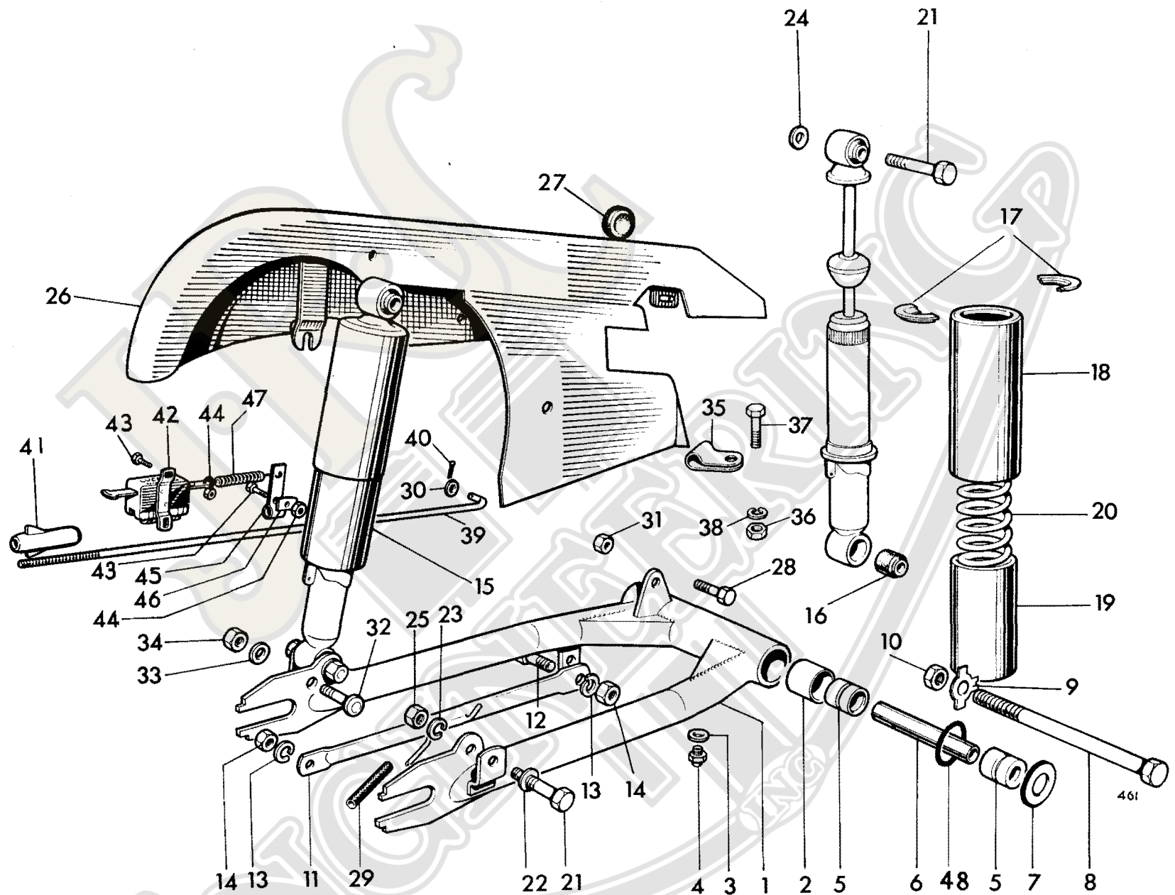
Fig. 13. SWINIGN FORK AND SUSPENSION UNITS
