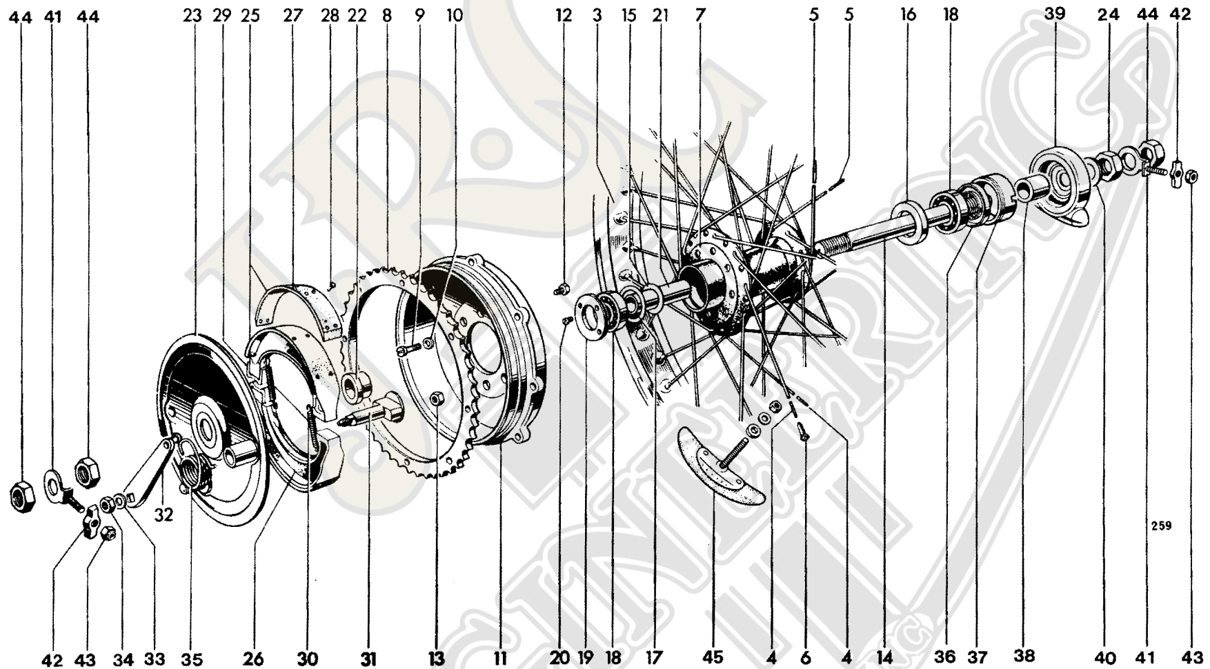
Fig. 20. REAR WHEEL
