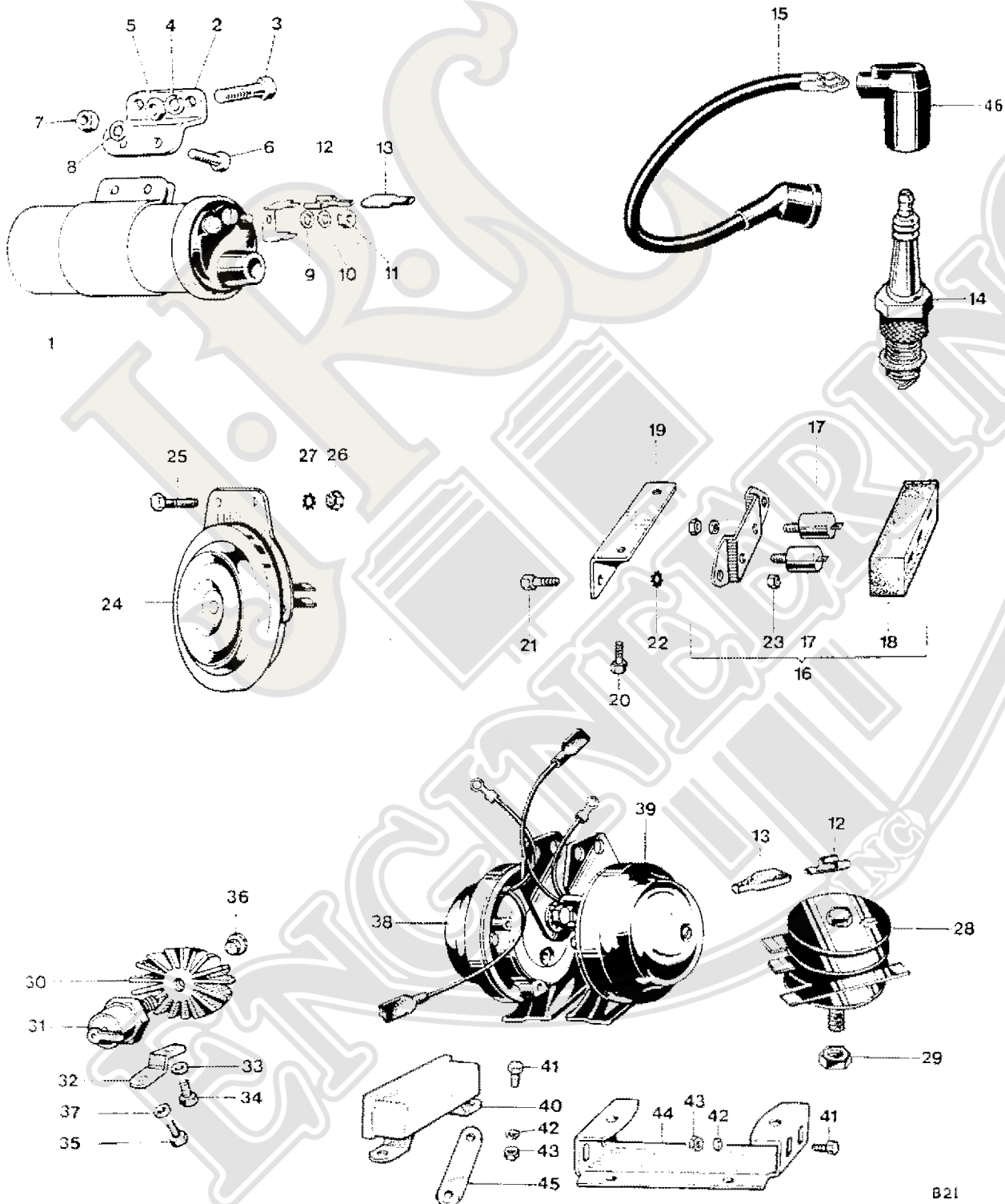
Fig. 33. IGNITION COILS, HORN, RECTIFIER AND ZENER DIODE
