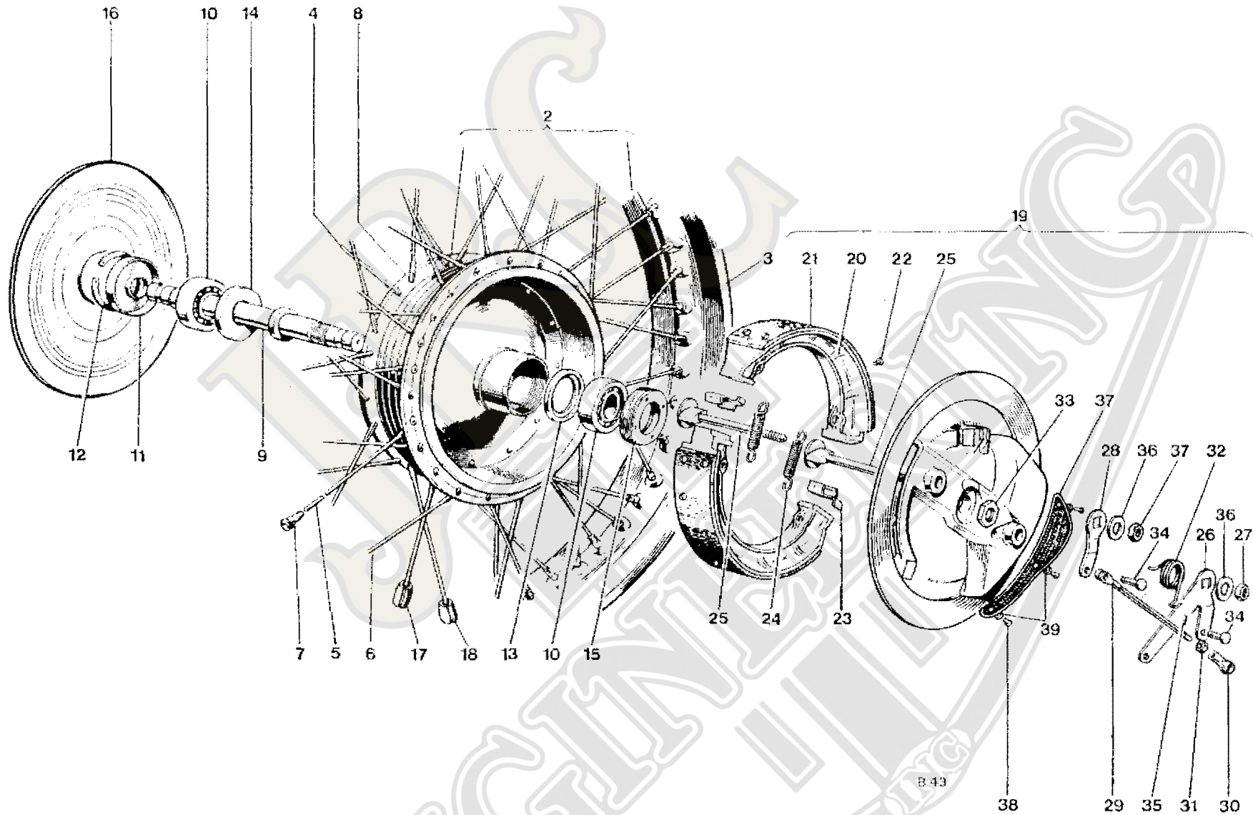
Fig. 19. FRONT WHEEL
