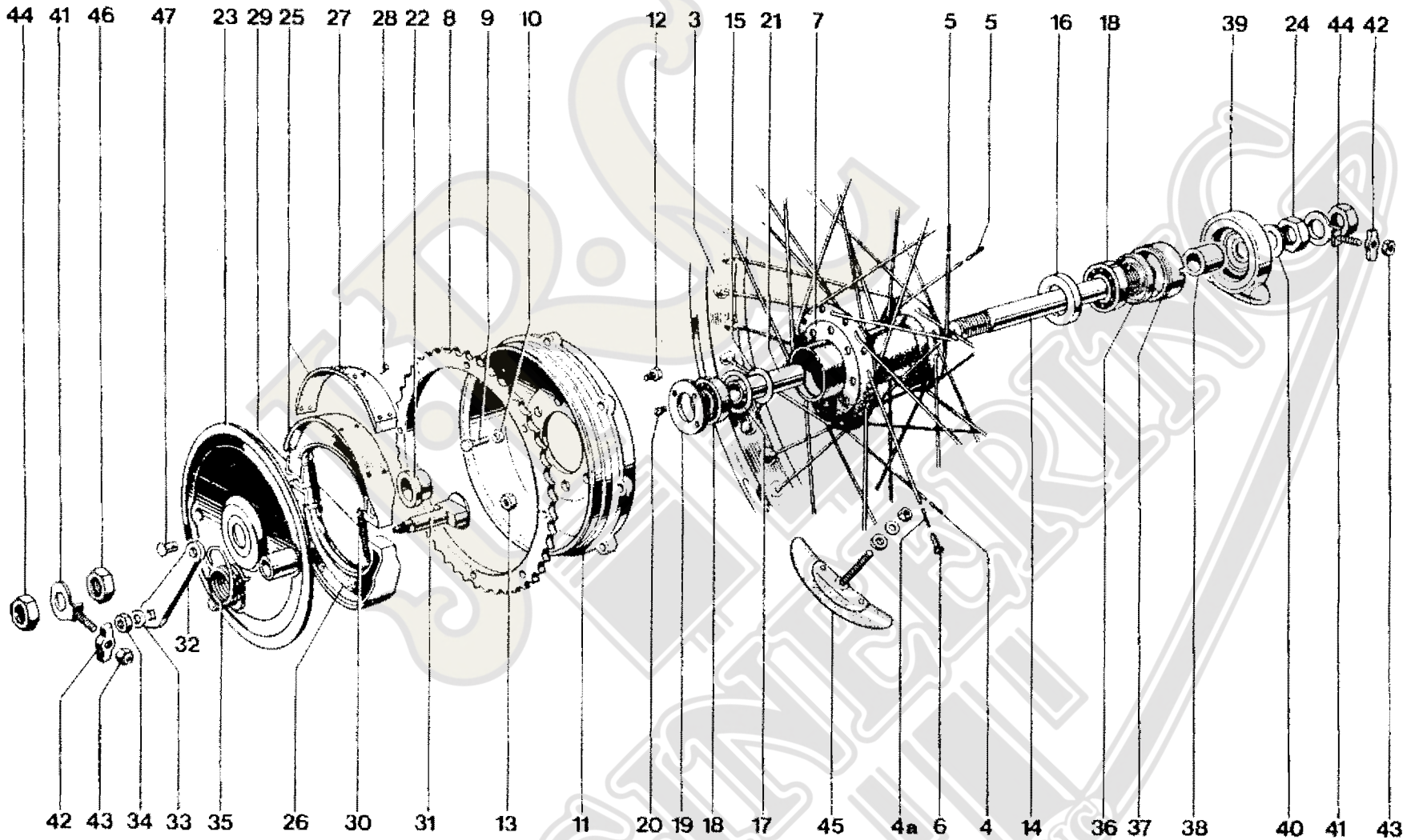
Fig. 20. REAR WHEEL
