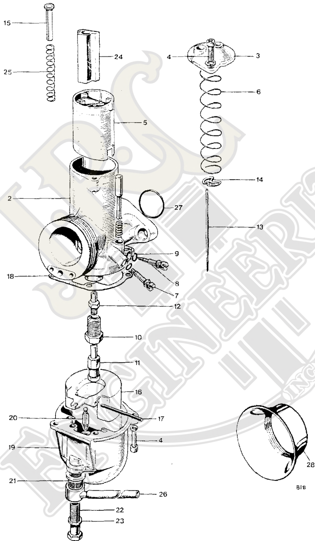
Fig. 29. AMAL CARURETOR, TR6R, TR6C www.jrcengineering.com 951-940-5411
