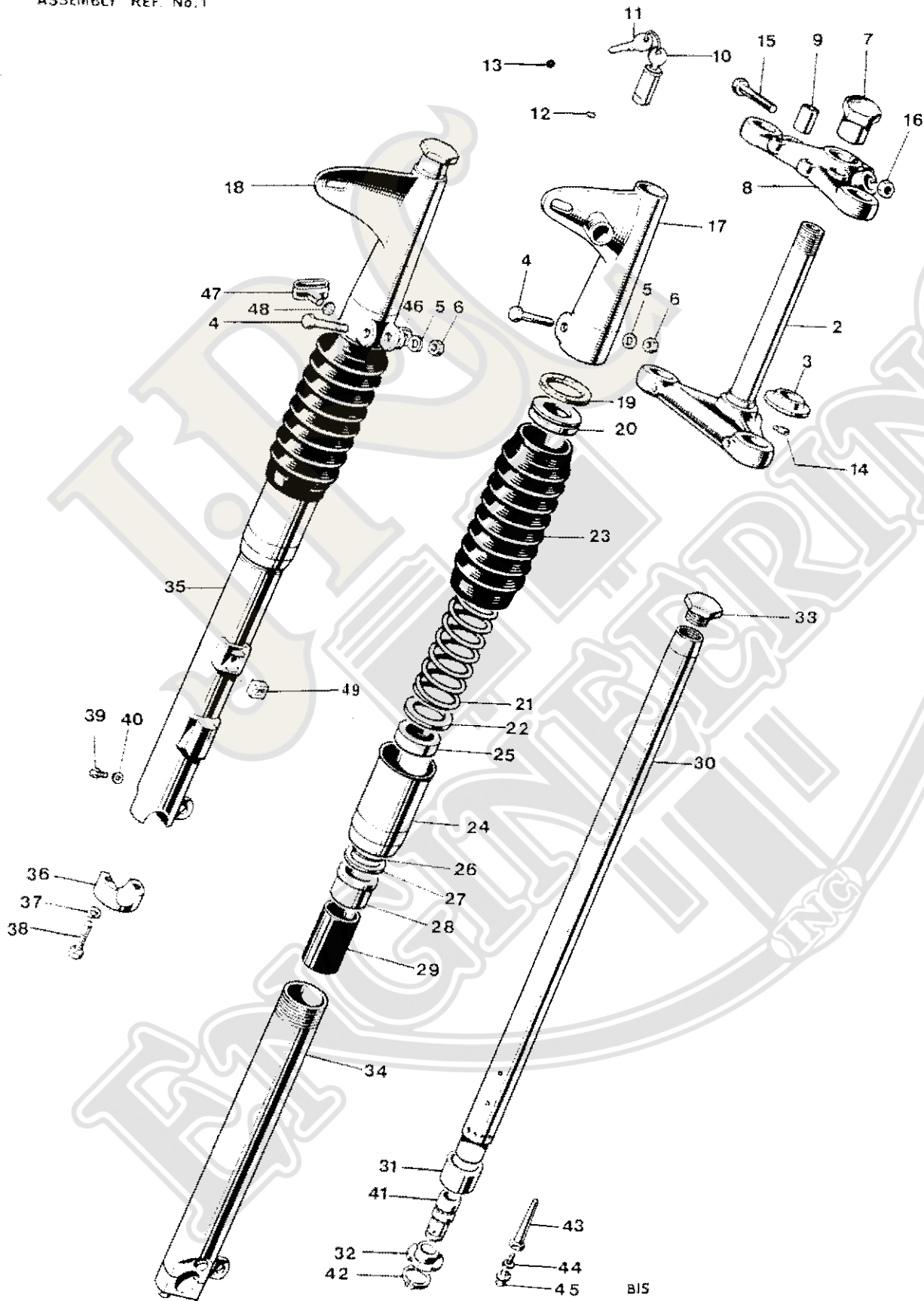
Fig. 16. TELESCOPIC FRONT FORK www.jrcengineering.com 951-940-5411
