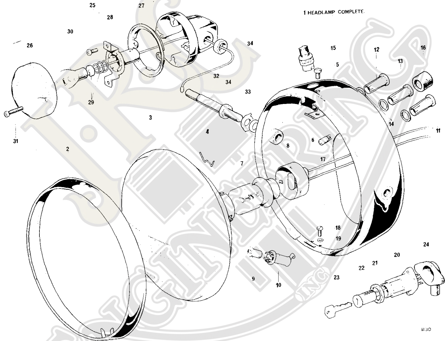
Fig. 31. HEADLAMP AND FLASHER LAMPS
