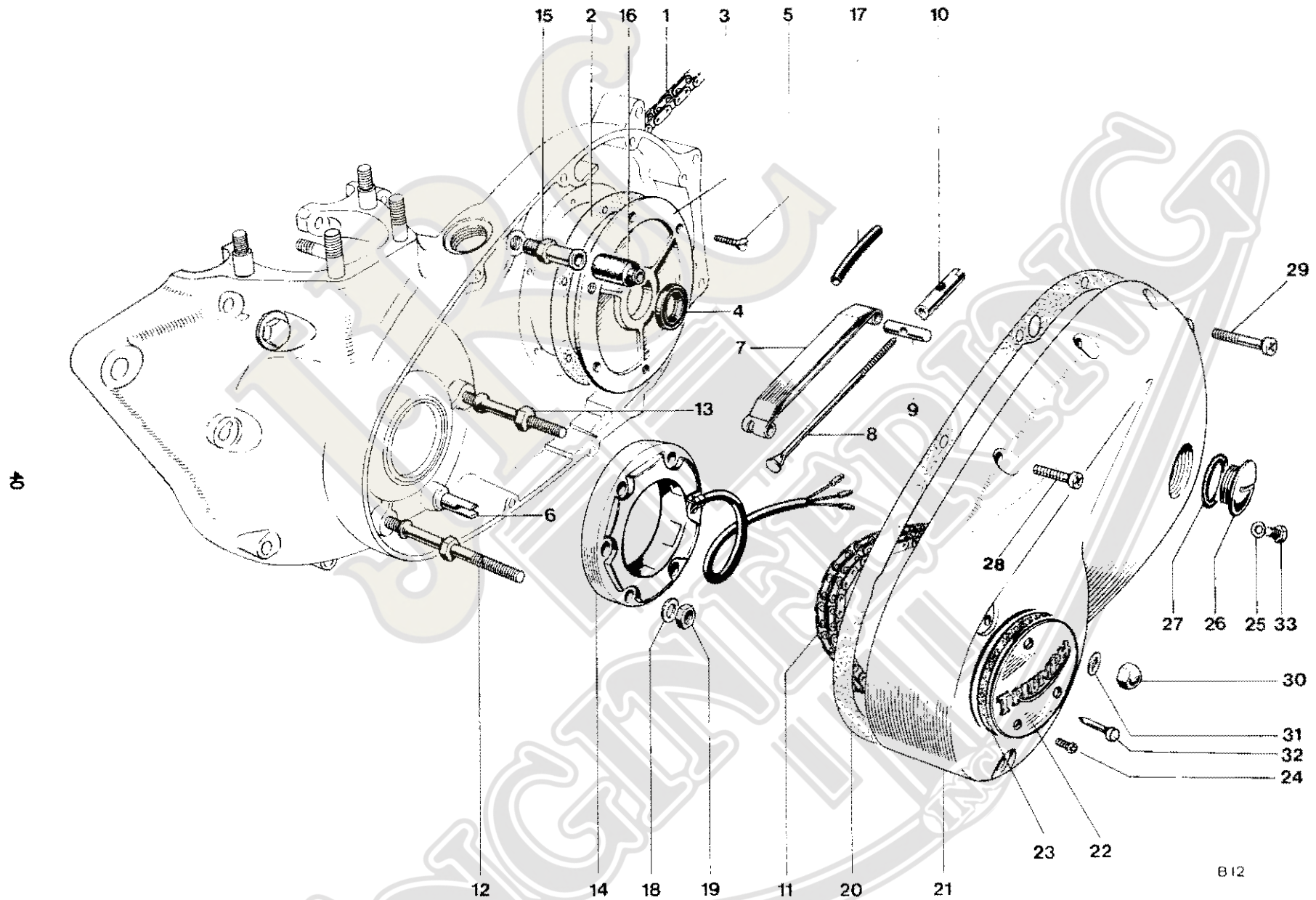
Fig. 13. CHAINCASE AND CHAINS
