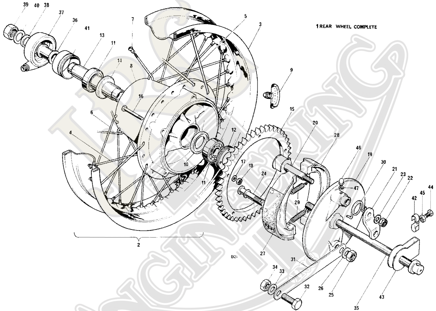
Fig. 25. REAR WHEEL
