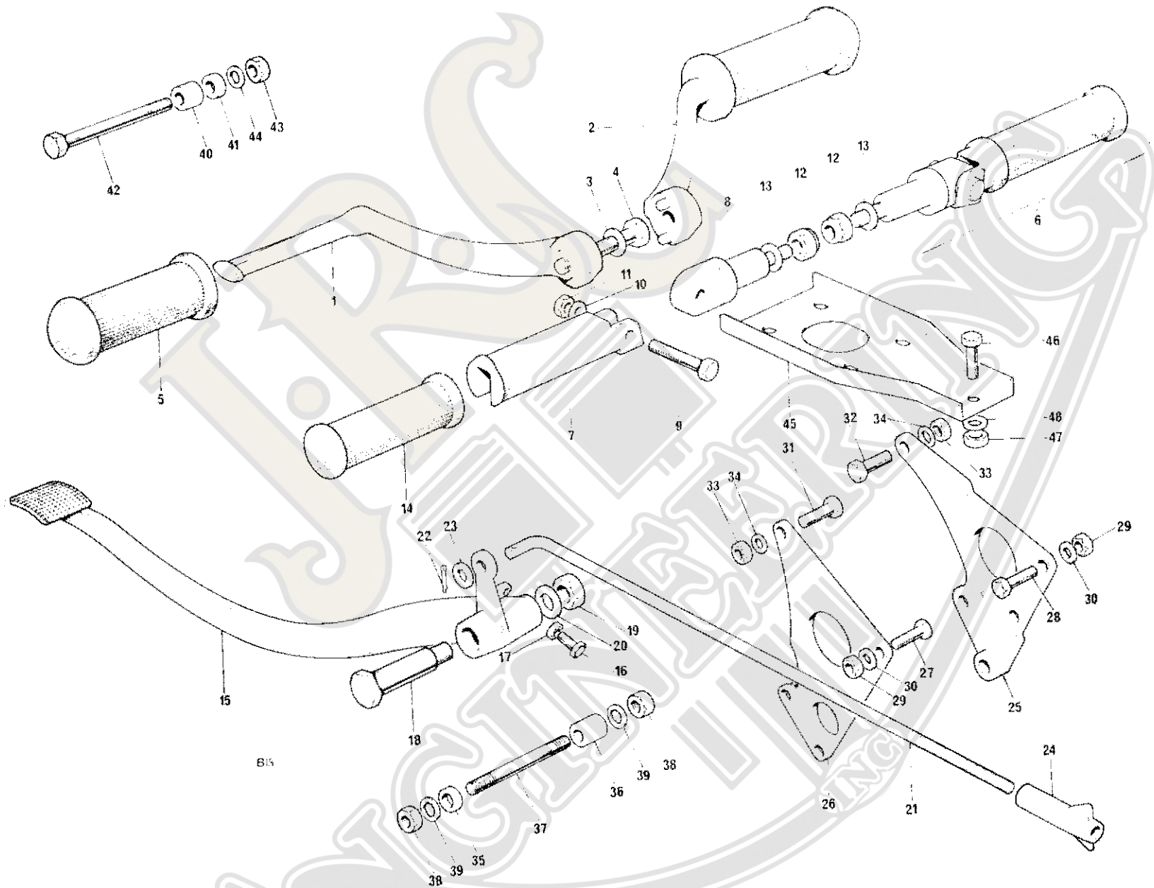
Fig. 19. MOTOR UNIT FITTING AND FOOTRESTS
