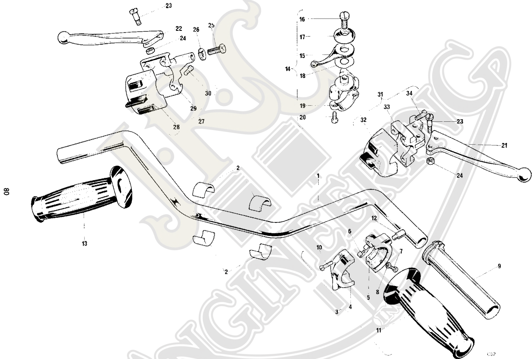
Fig. 29. HANDLEBAR AND CONTROL LEVERS
