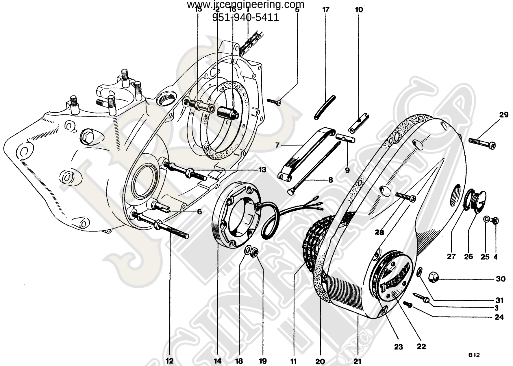
Fig. 15. CHAINCASE AND CHAINS
