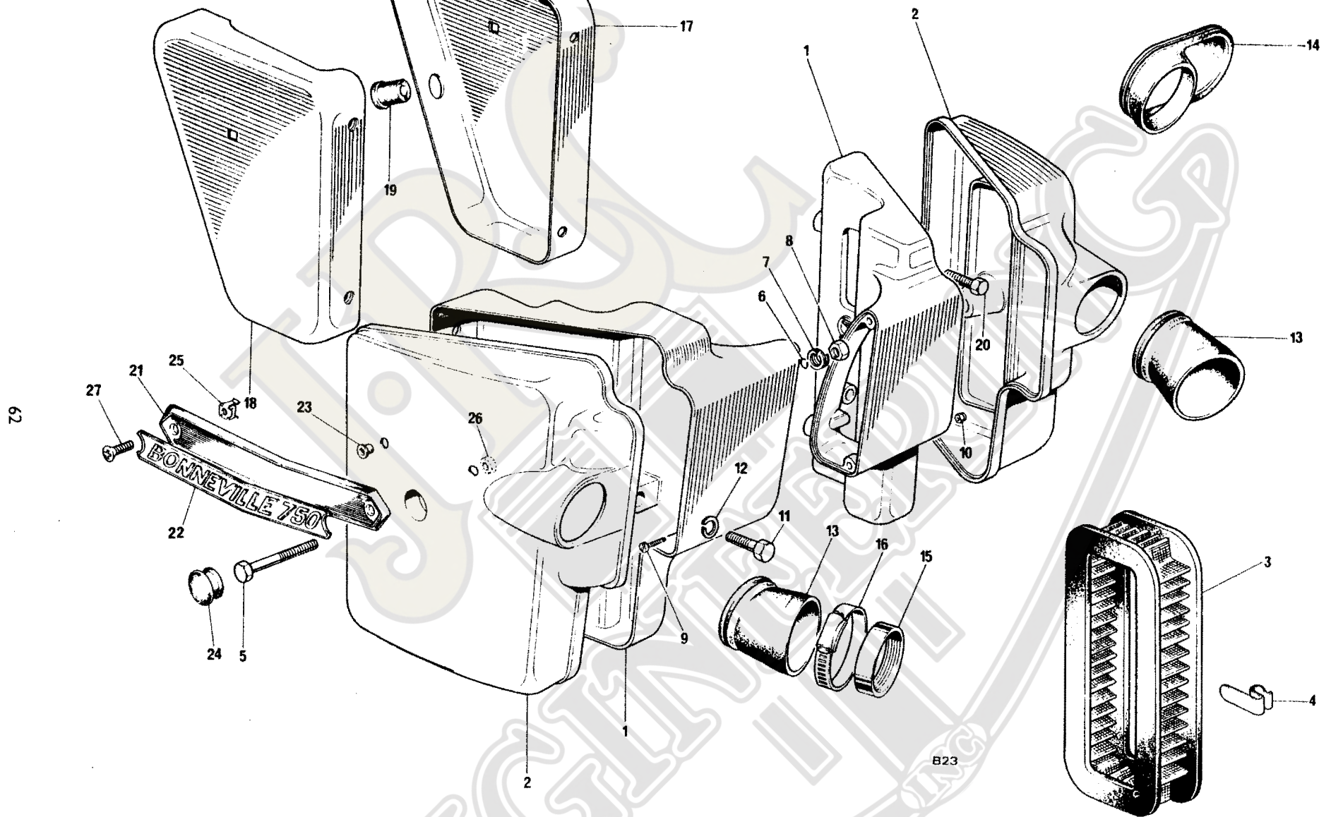
Fig. 26 AIR CLEANERS AND SIDE PANELS
