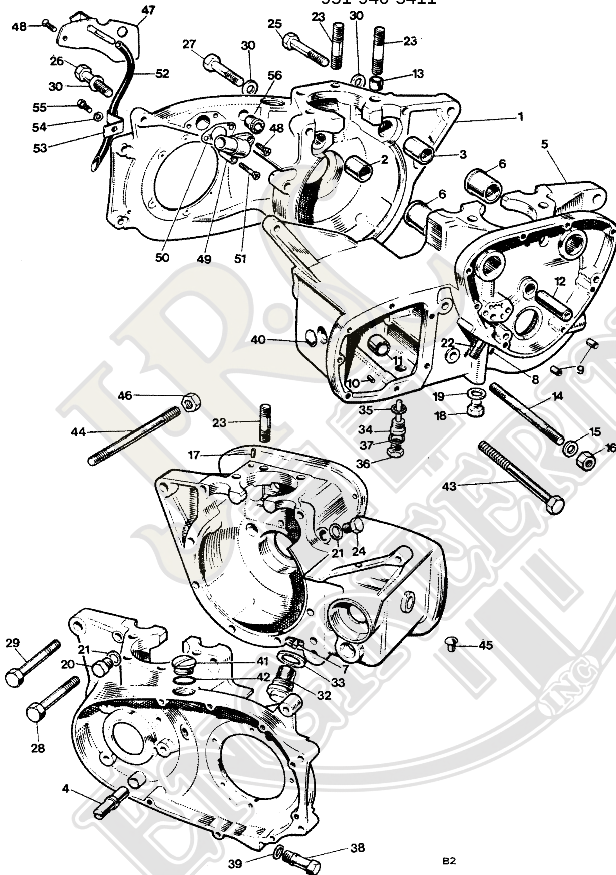
Fig. 2 CRANKCASE
