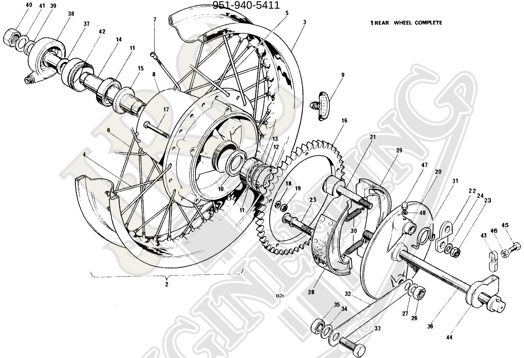
Fig 24. REAR WHEEL
