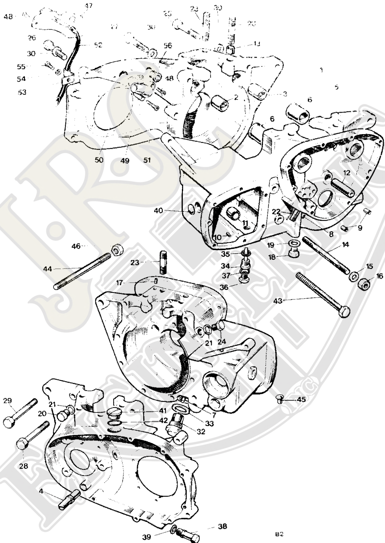
Fig. 2 CRANKCASE
