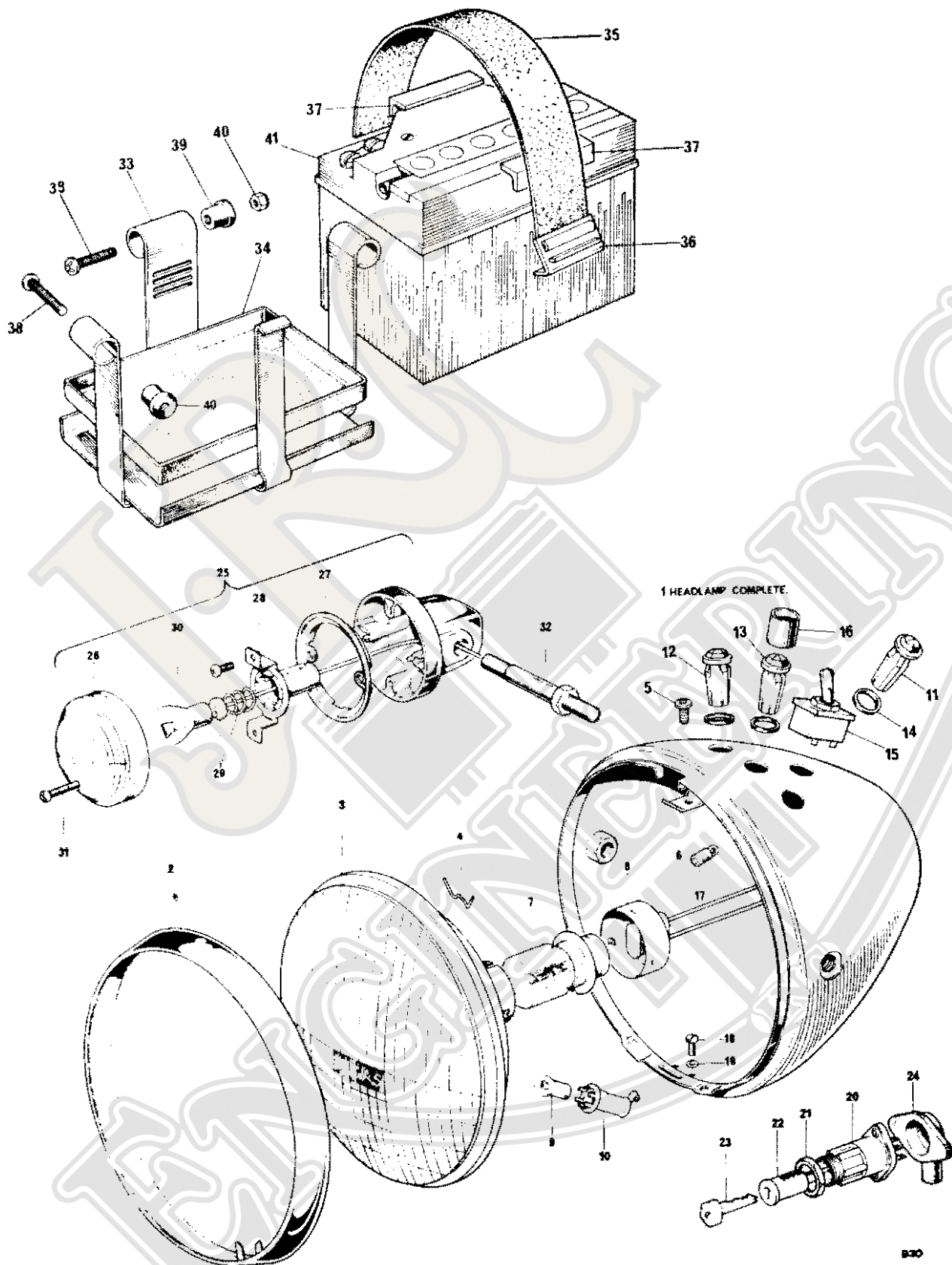
Fig. 34. HEADLAMP AND FLASHER LAMP
