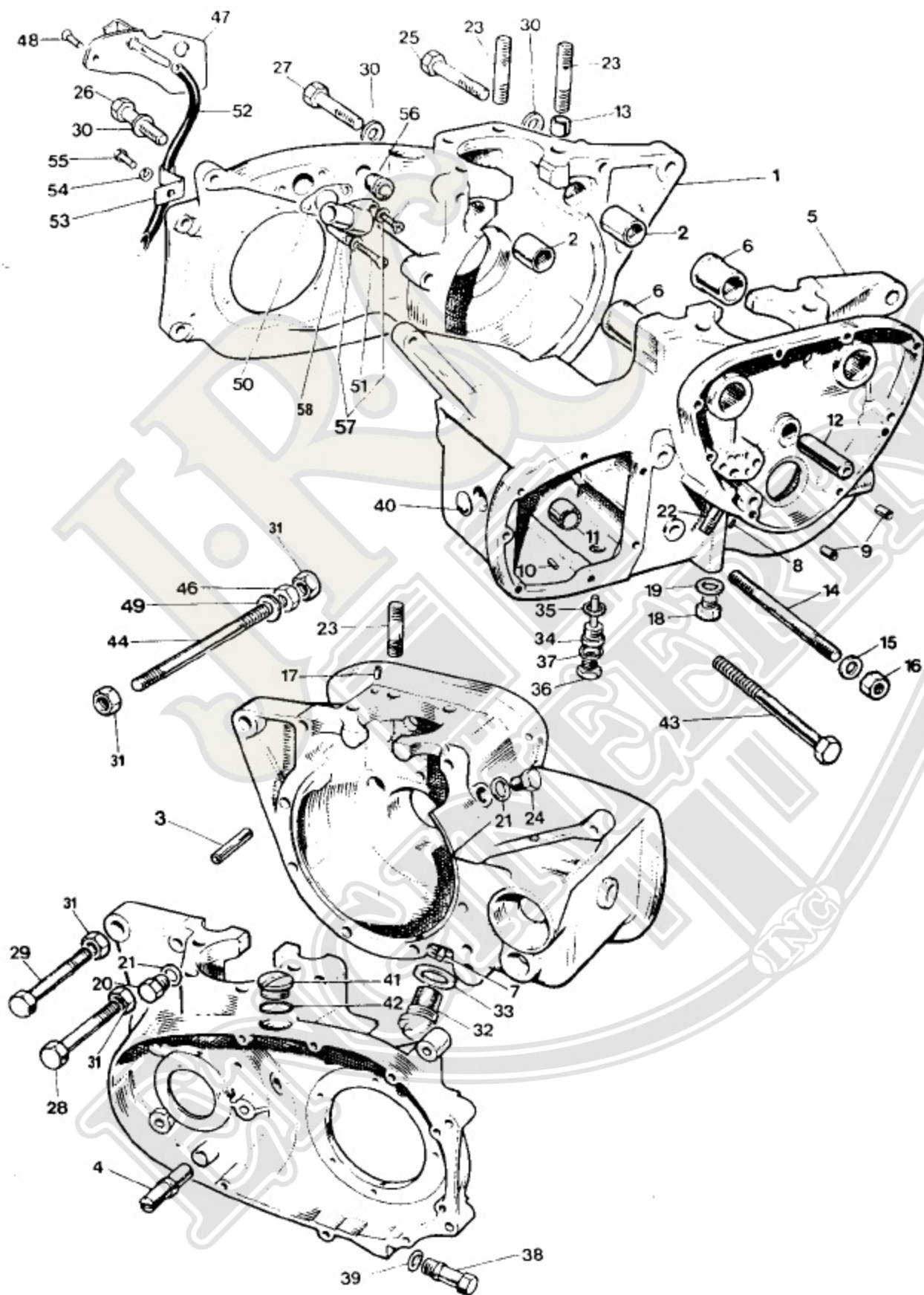
Fig. 2 CRANKCASE
