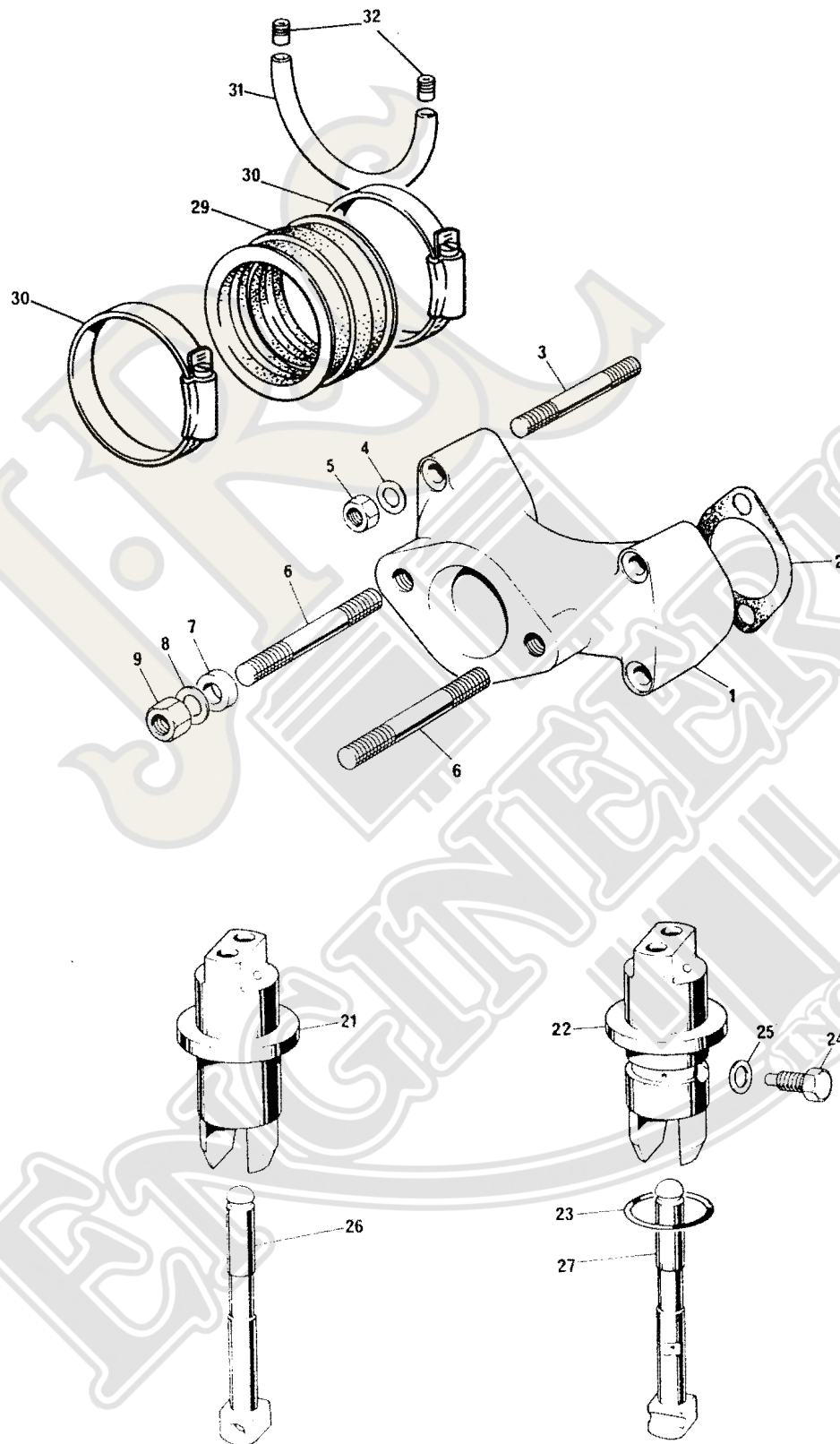
Fig. 4. MANIFOLD AND TAPPETS
