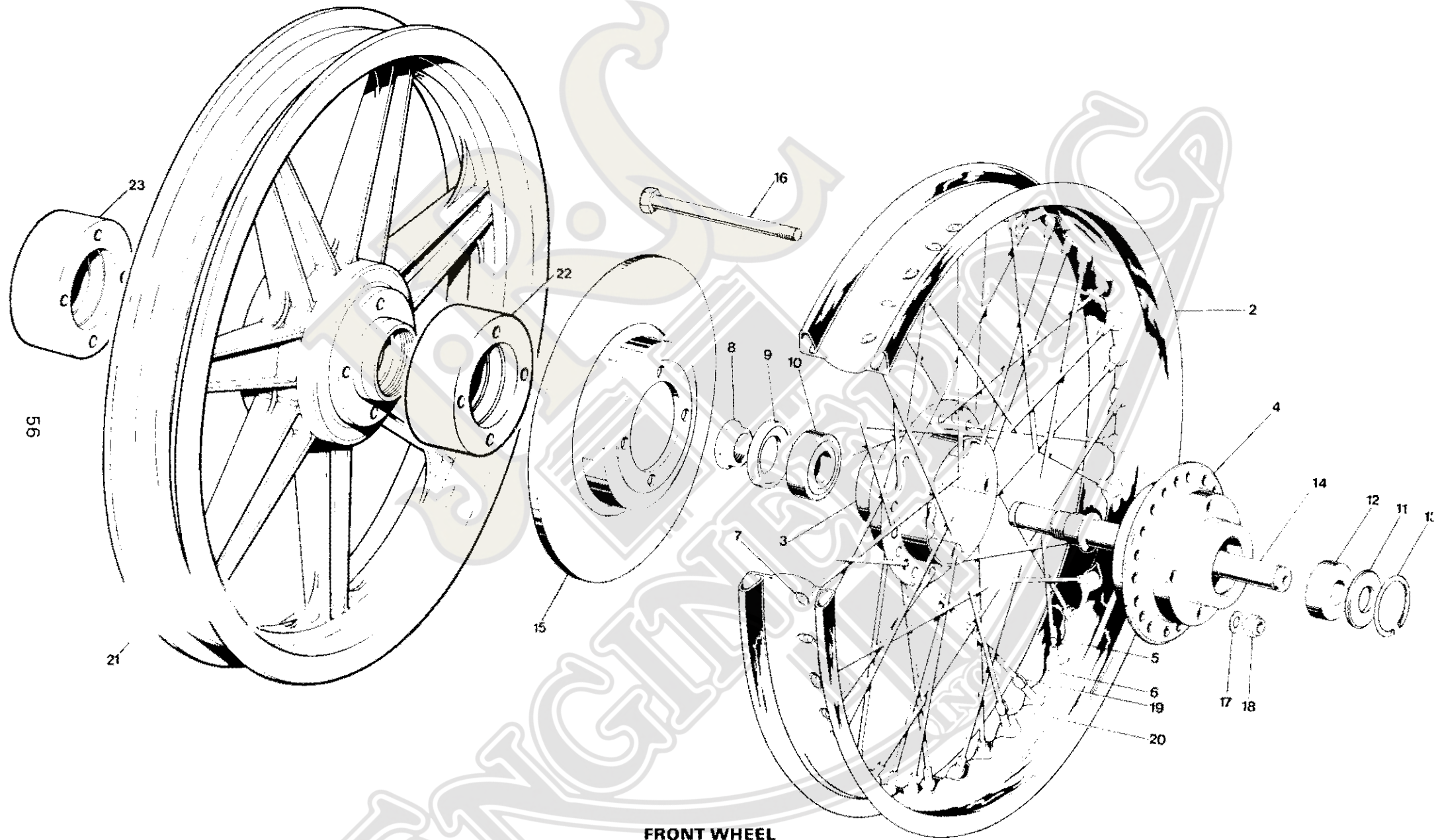
FRONT WHEEL
