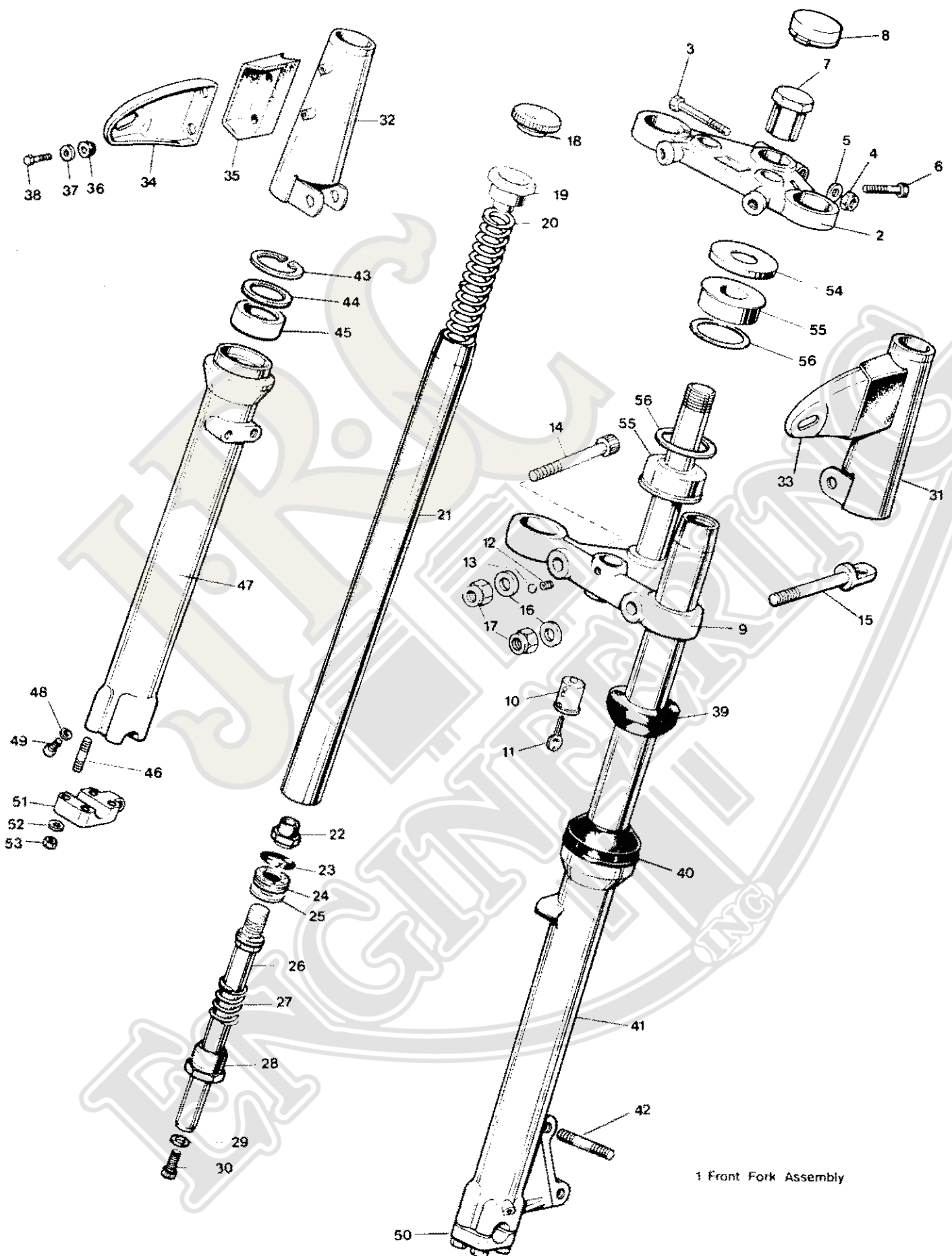
TELESCOPIC FRONT FORK
