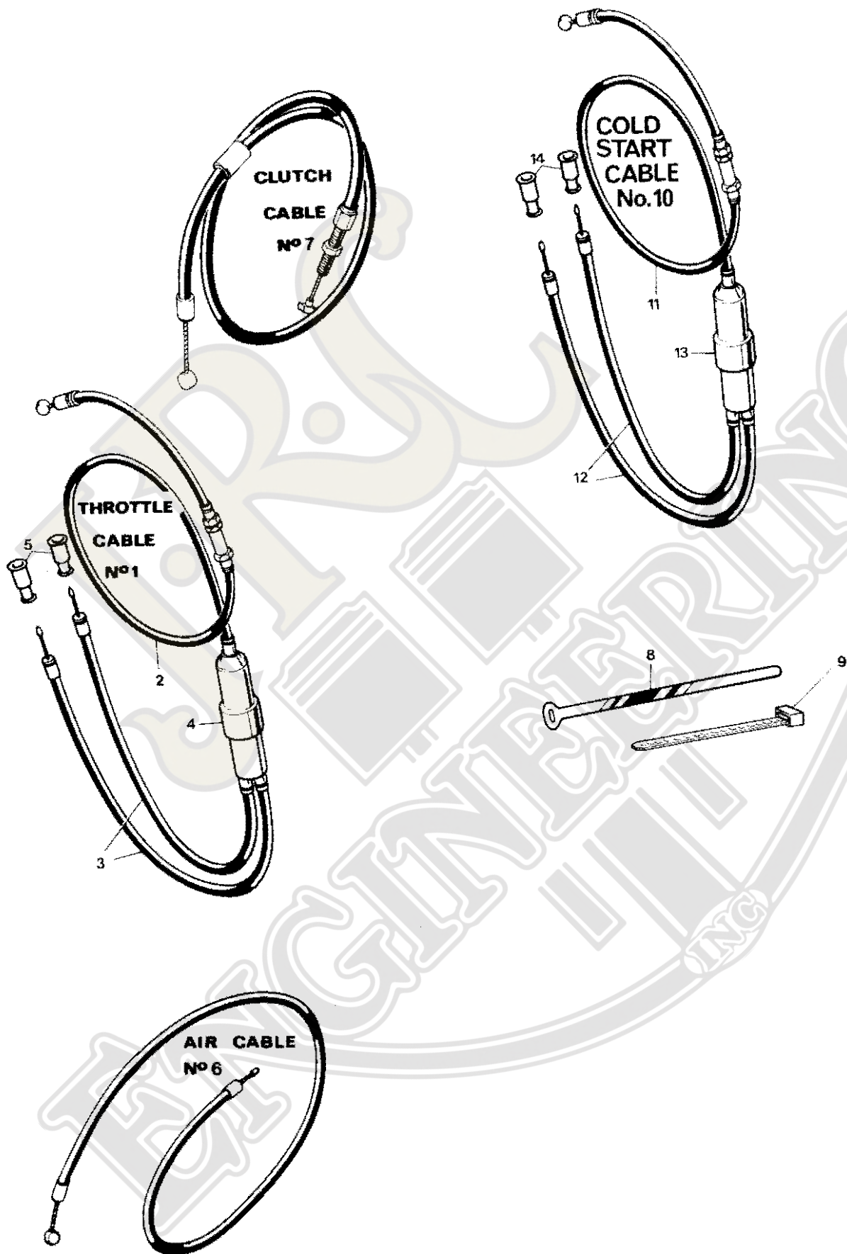
CONTROL CABLES
