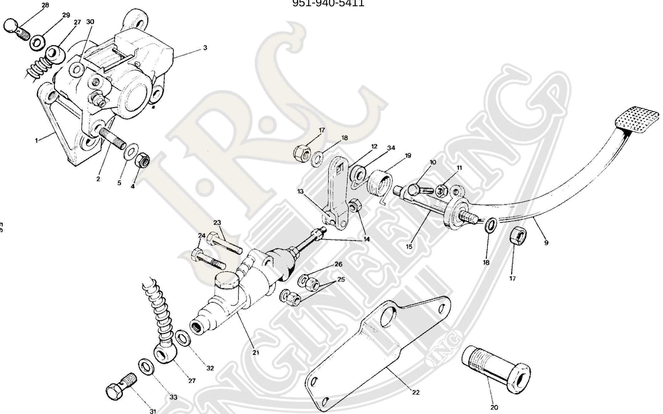
REAR BRAKE
