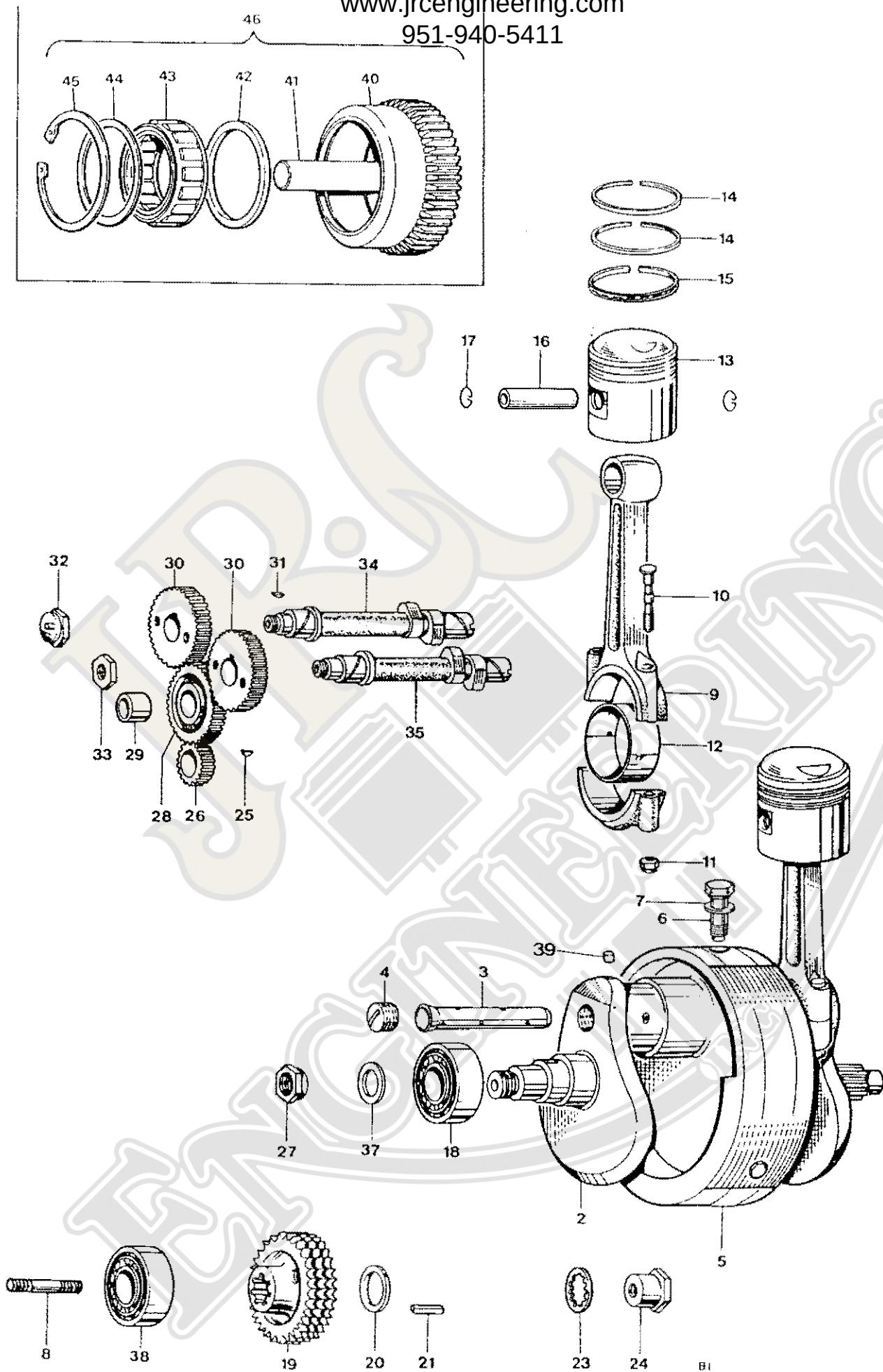
CRANKSHAFT AND CONNECTING RODS
