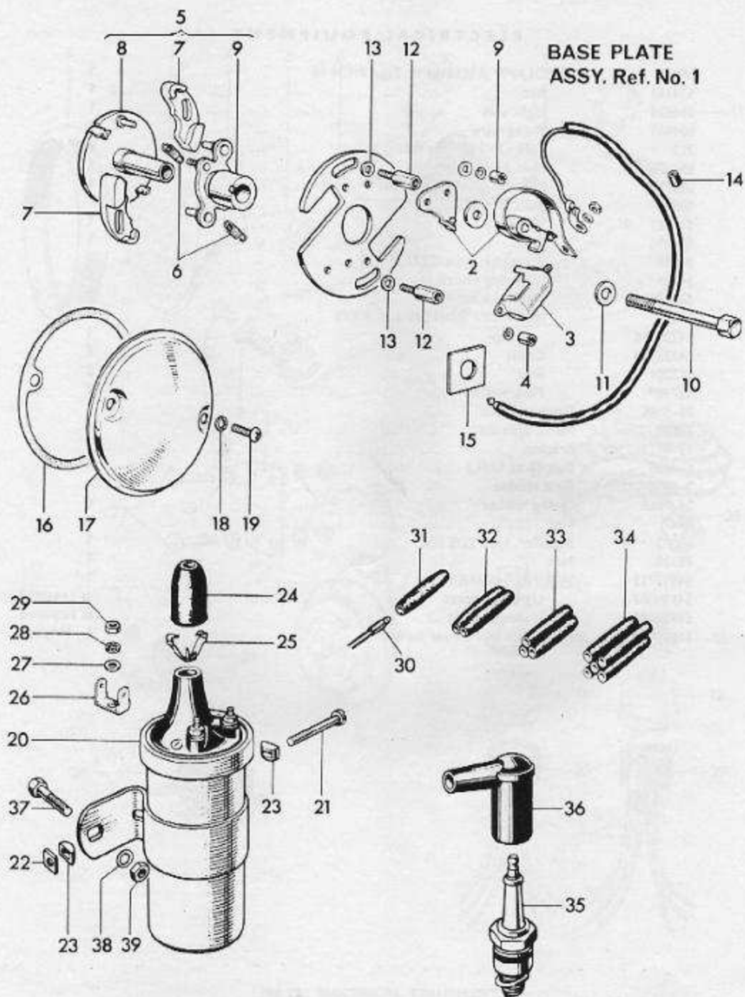
Fig. 24. CONTACT BREAKER AND IGNITION COIL
