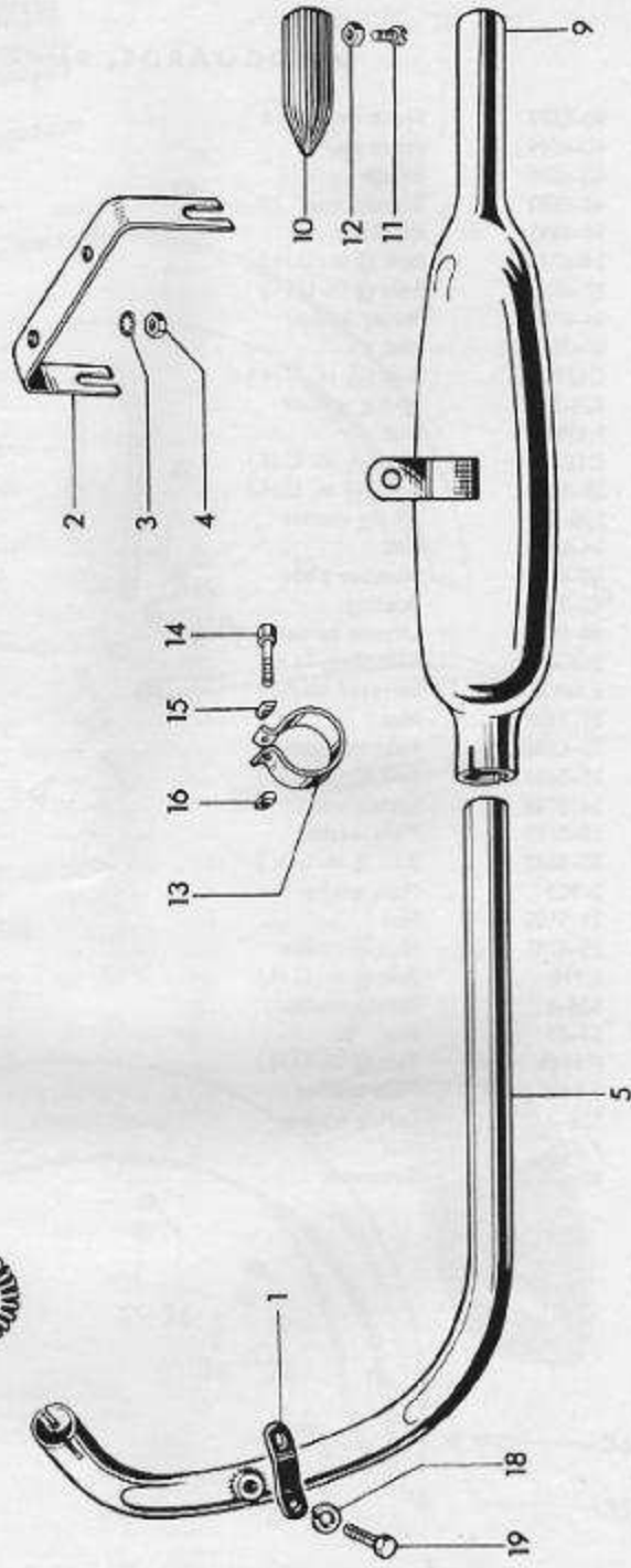
FIG. 16. TWINSEAT AND EXHAUST SYSTEM
