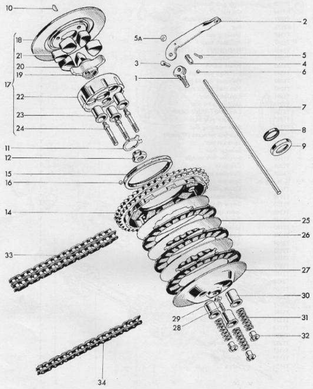
Fig. 6. CLUTCH AND CHAINS
