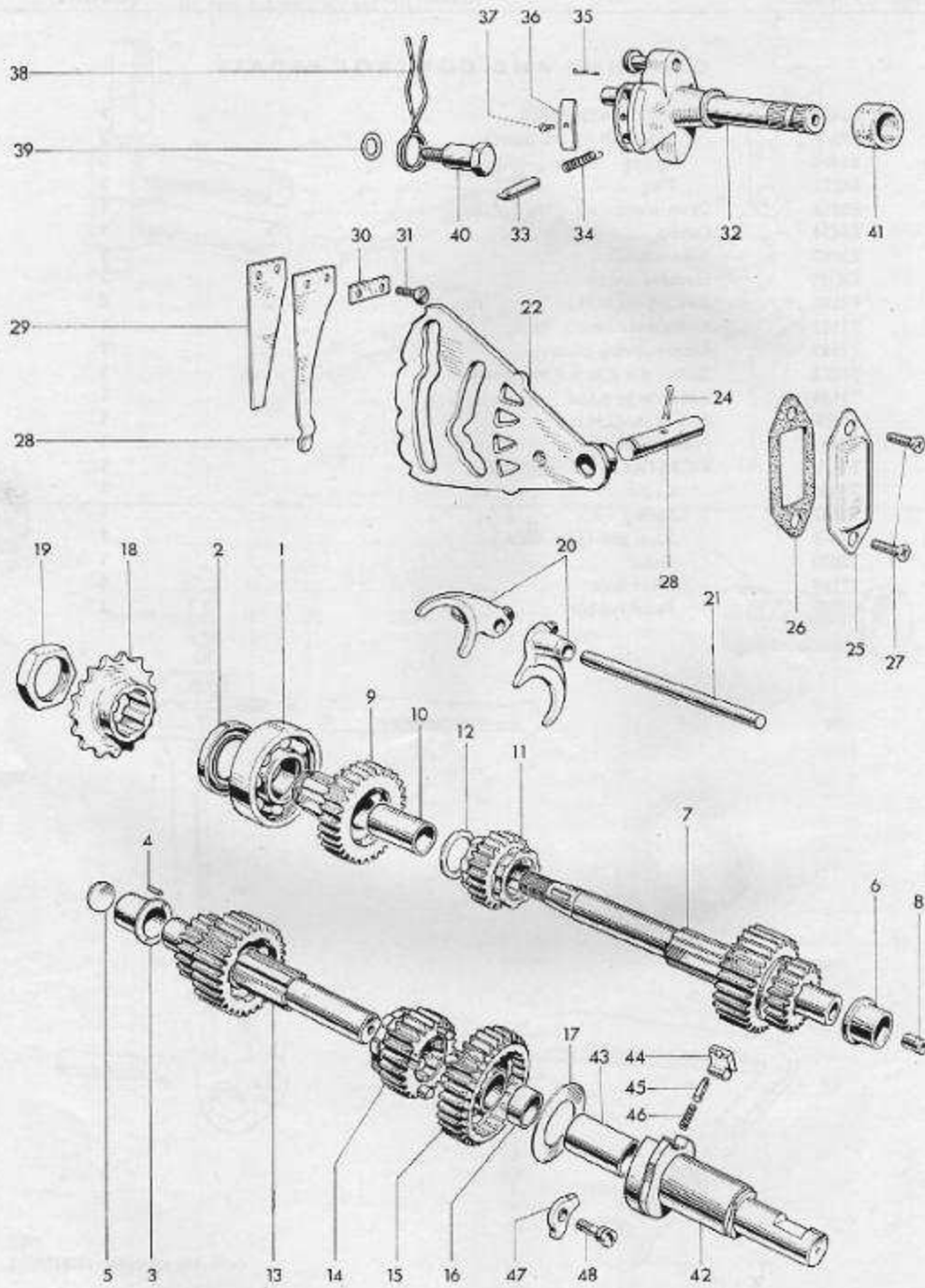
Fig. 5. GEARBOX SHAFTS AND GEARS
