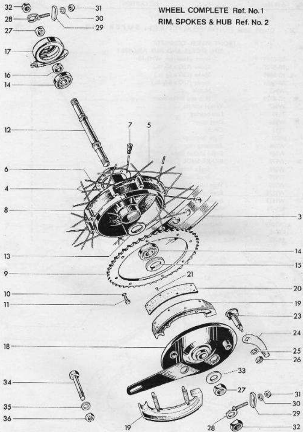
Fig. 12. REAR WHEEL, BANTAM CUB
