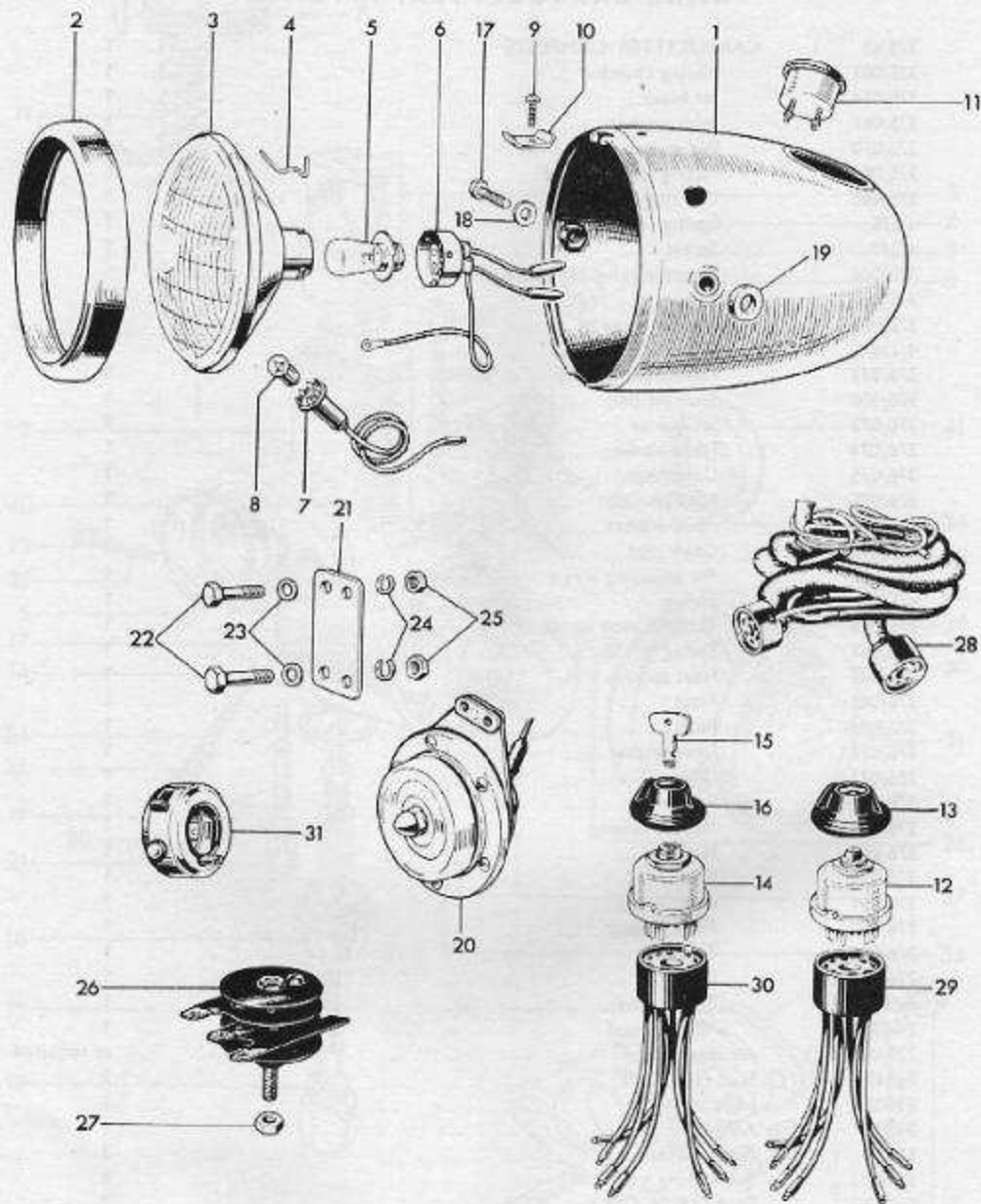
Fig. 23. ELECTRICAL EQUIPMENT
