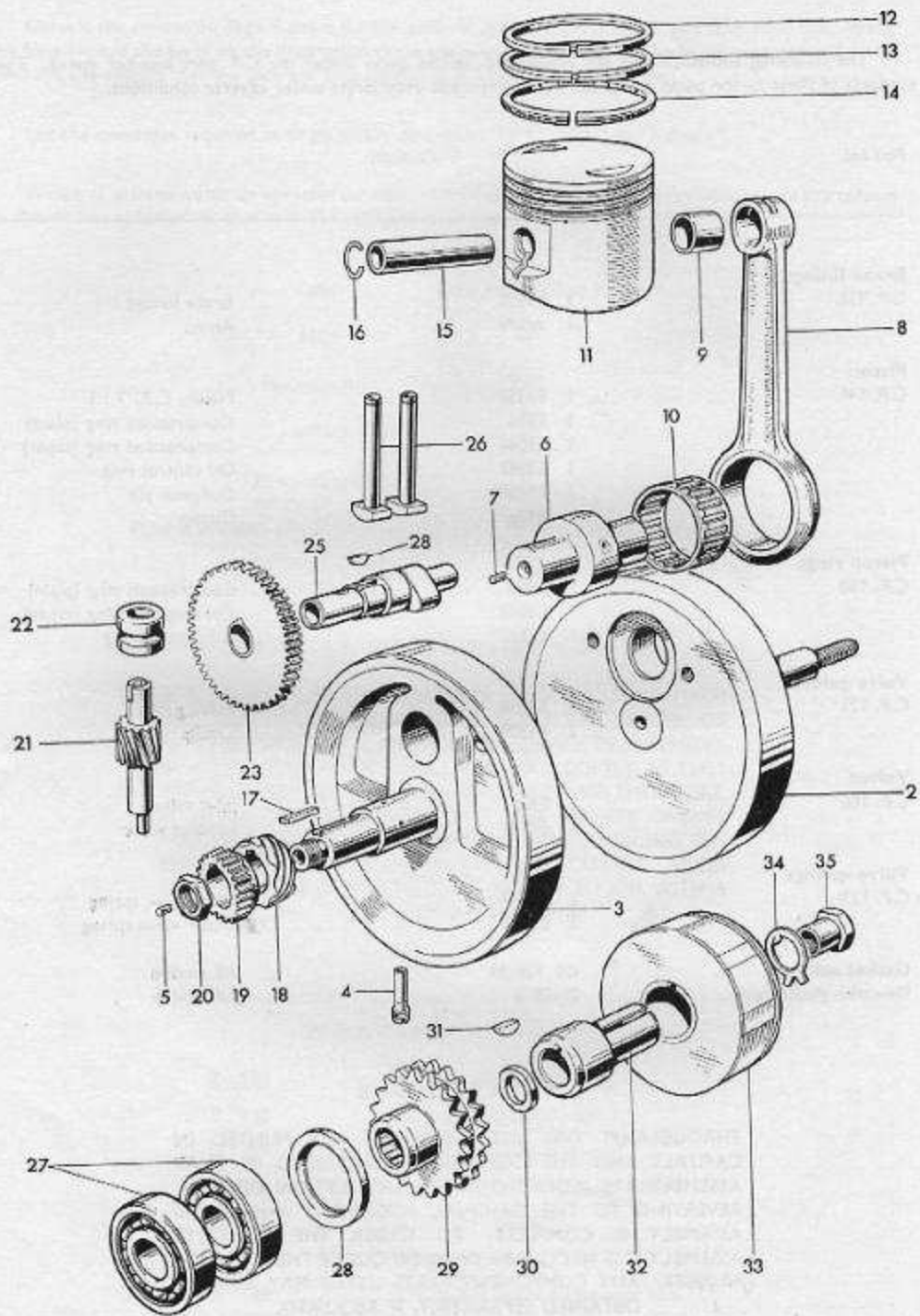
Fig. 1. CRANKSHAFT, PISTON AND TIMING GEARS
