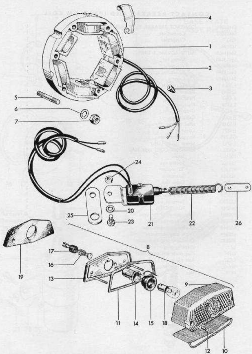
Fig. 25. STATOR, TAIL LAMP AND STOP LAMP SWITCH
