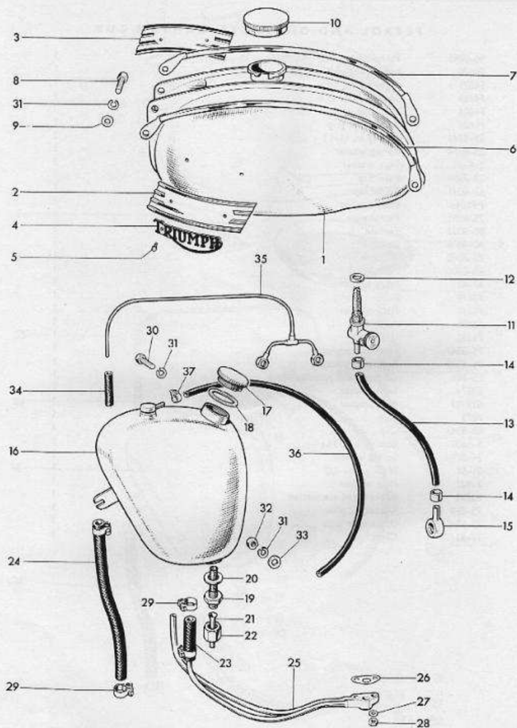
Fig. 10. PETROL AND OIL TANKS, SUPER CUB
