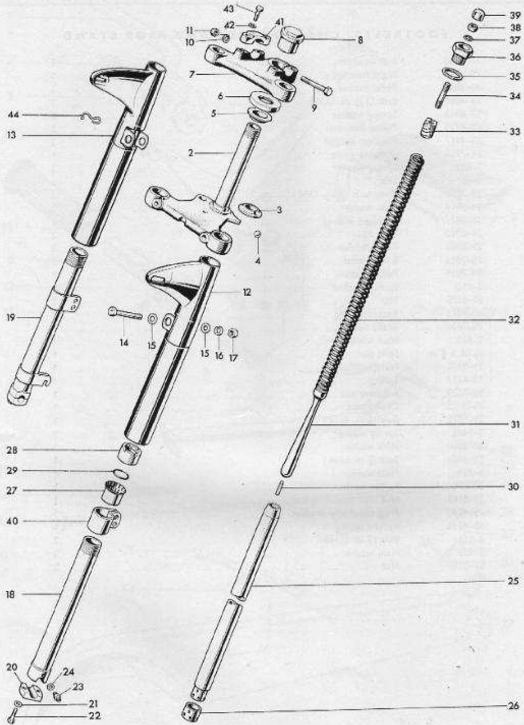
Fig. 9. TELESCOPIC FRONT FORK
