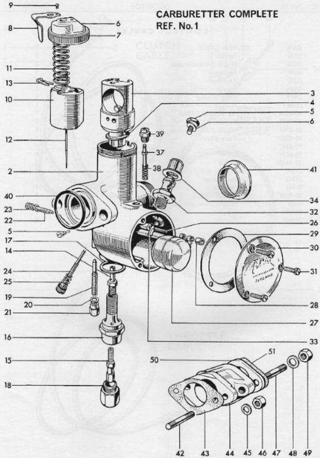
Fig. 22. AMAL CARBURETTER, TYPE 375
