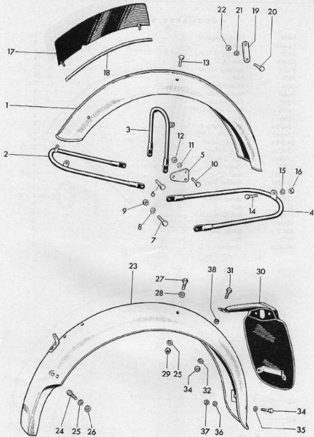
Fig. 15. MUDGUARDS, SUPER CUB
