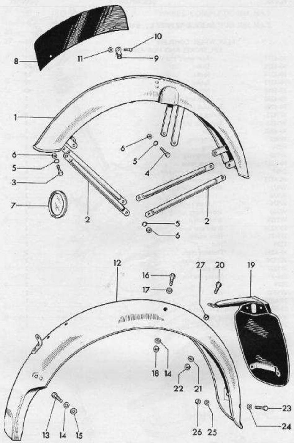
FIG. 14. MUDGUARDS, BANTAM CUB
