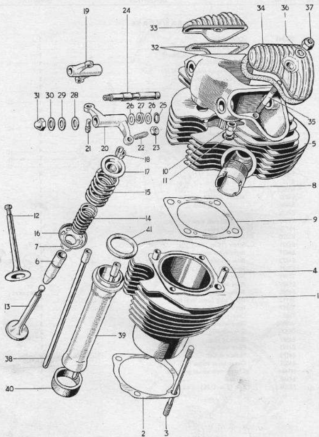
Fig. 3. CYLINDER BARREL AND HEAD
