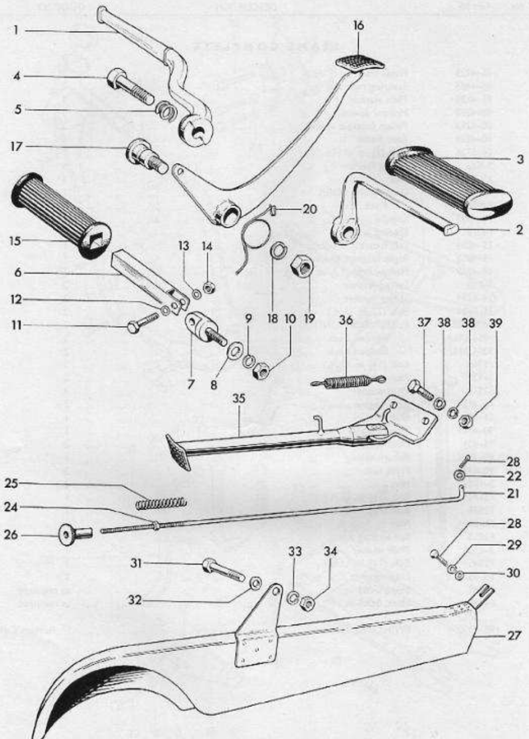
Fig. 8. FOOTRESTS, CHAINGUARD AND PROP STAND
