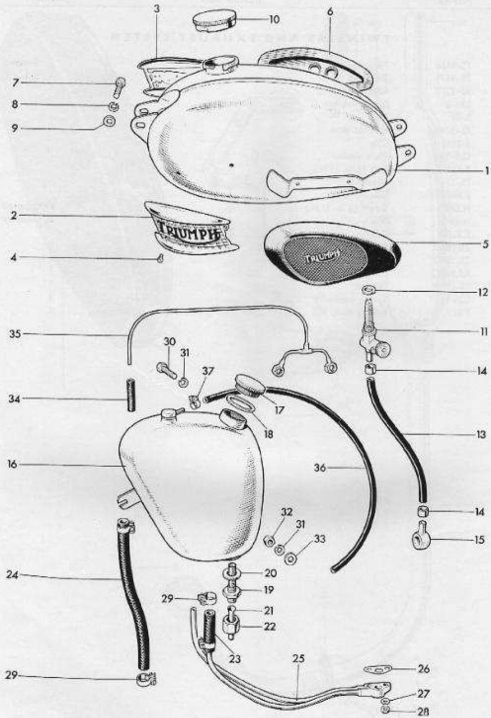
Fig. 17. PETROL AND OIL TANKS, BANTAM CUB
