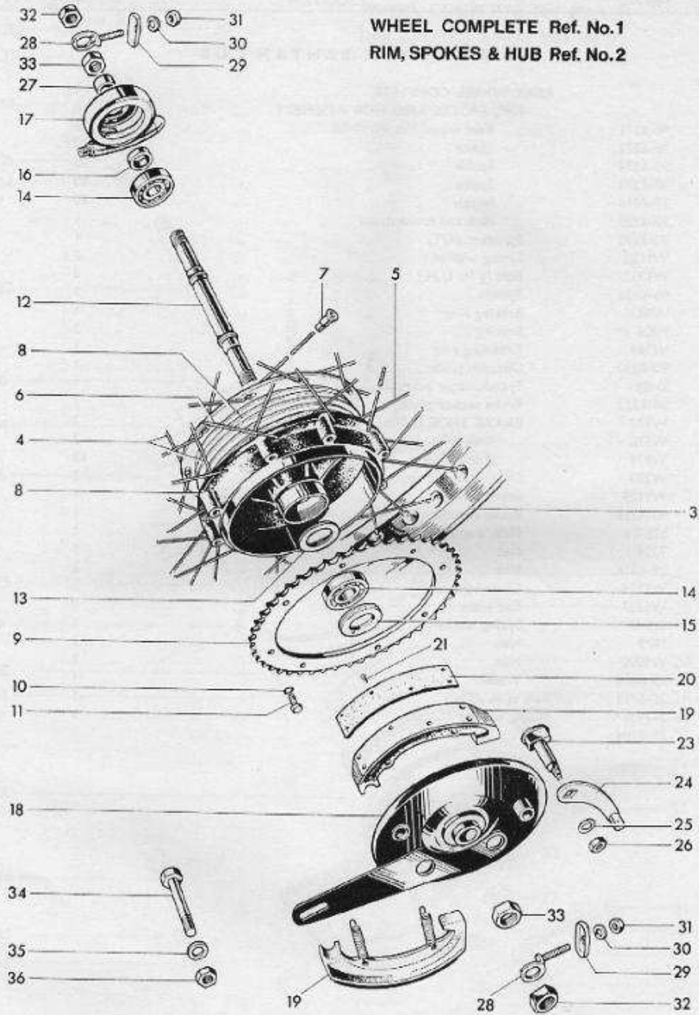
Fig. 13. REAR WHEEL, SUPER CUB
