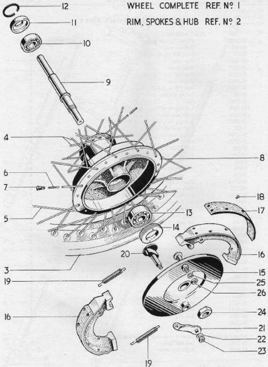
Fig. 10. FRONT WHEEL, BANTAM CUB
