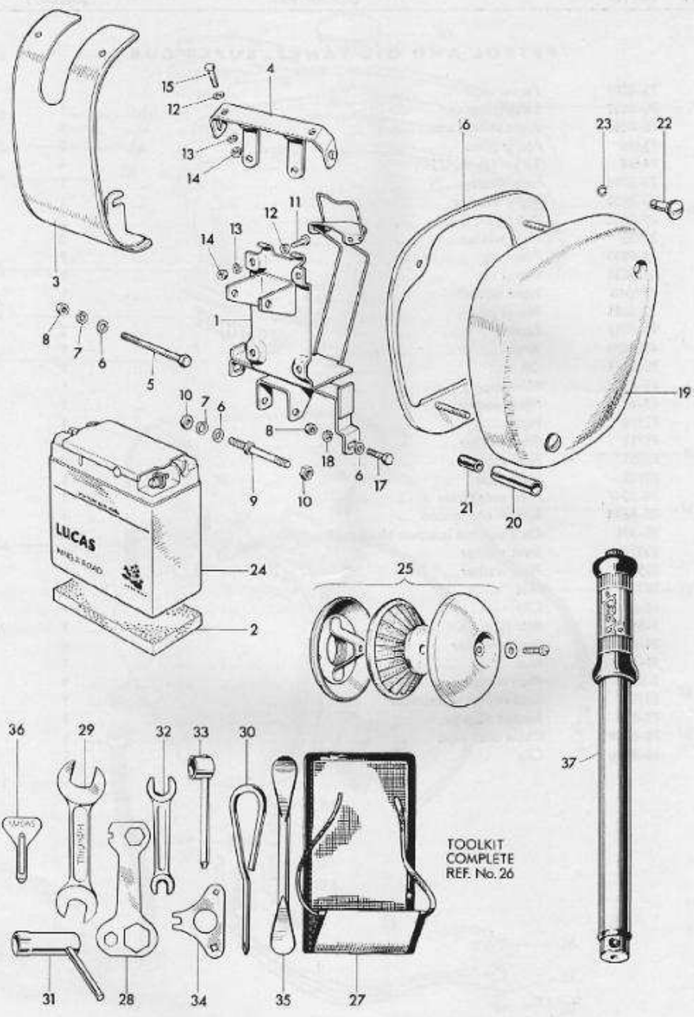
Fig. 19. BATTERY CARRIER, TOOLBOX AND AIR FILTER
