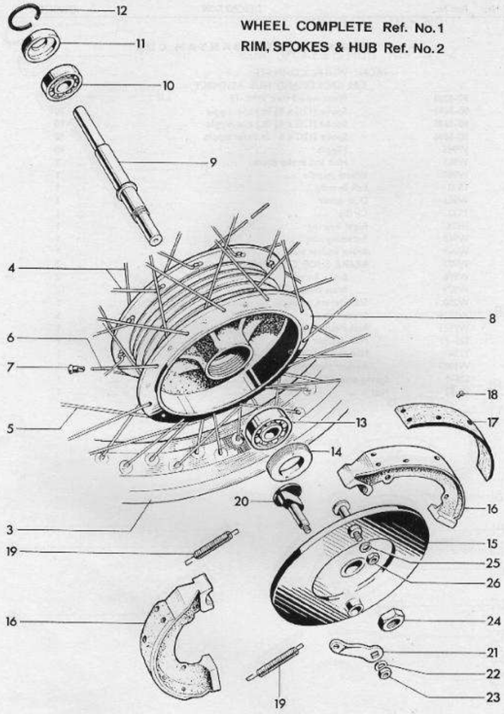
Fig. 11. FRONT WHEEL, SUPER CUB
