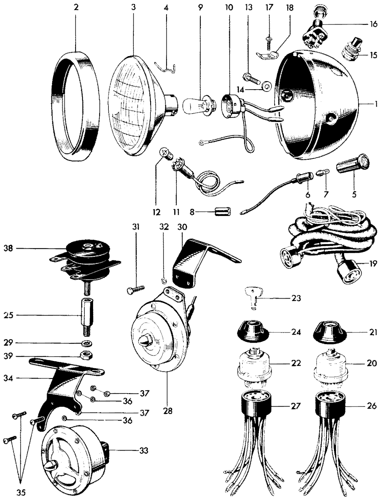
Fig. 19. ELECTRICAL EQUIPMENT
