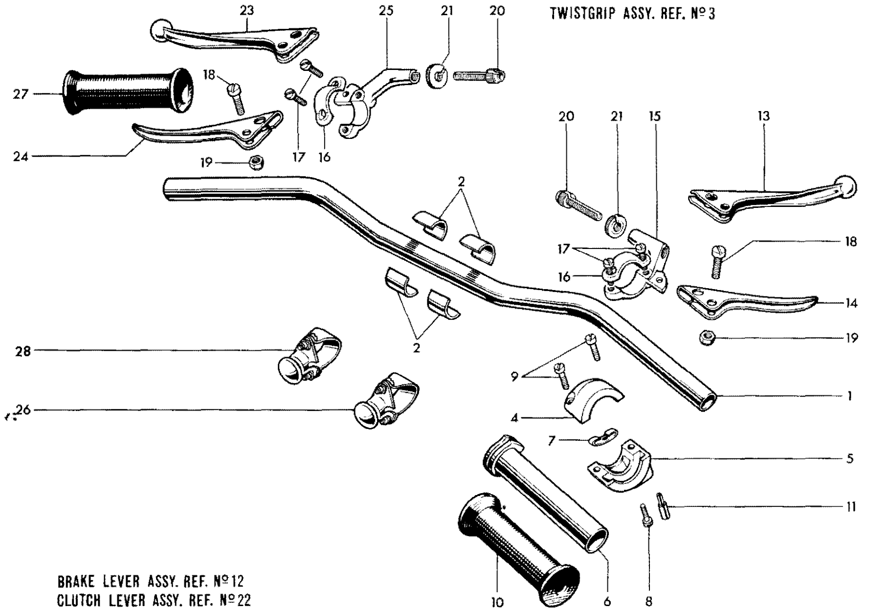
Fig. 16. HANDLEBARS AND CONTROL LEVERS
