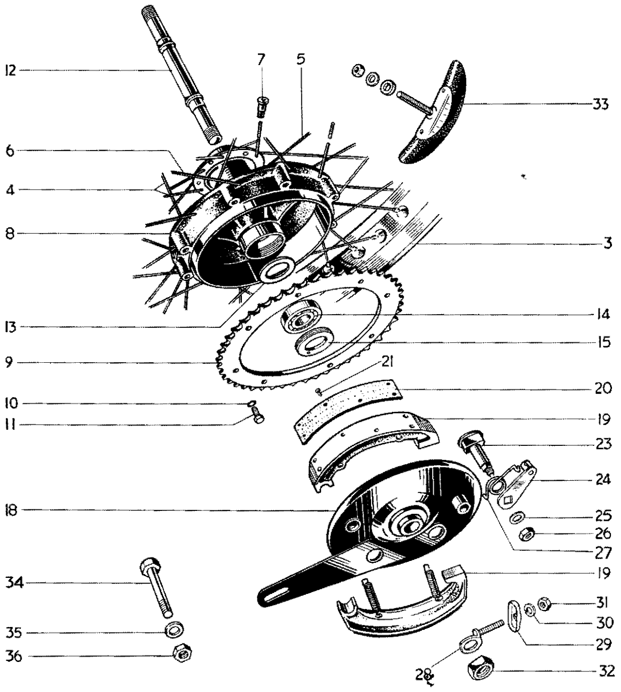
Fig. 11. REAR WHEEL
