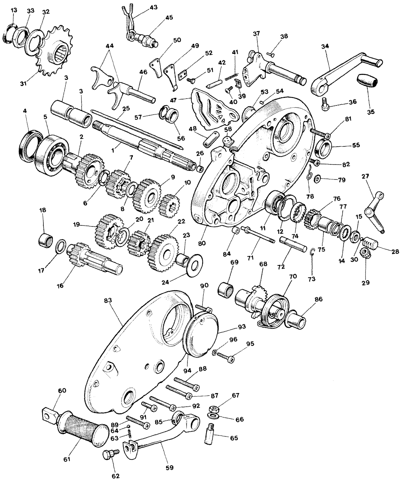
Fig. 3 GEAR CLUSTER
