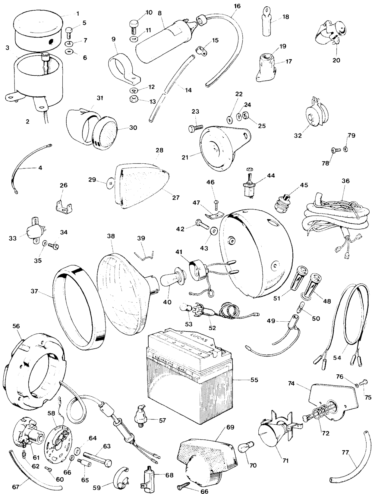
Fig.14 ELECTRICAL EQUIPMENT
