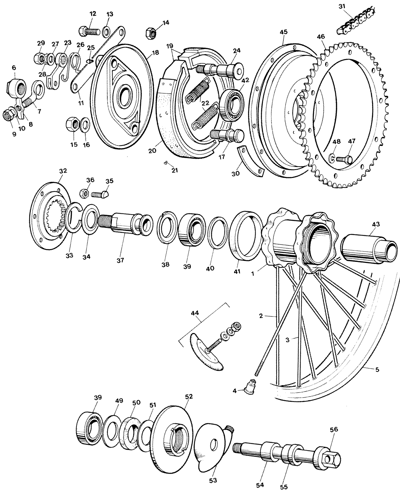
Fig.11 REAR WHEEL
