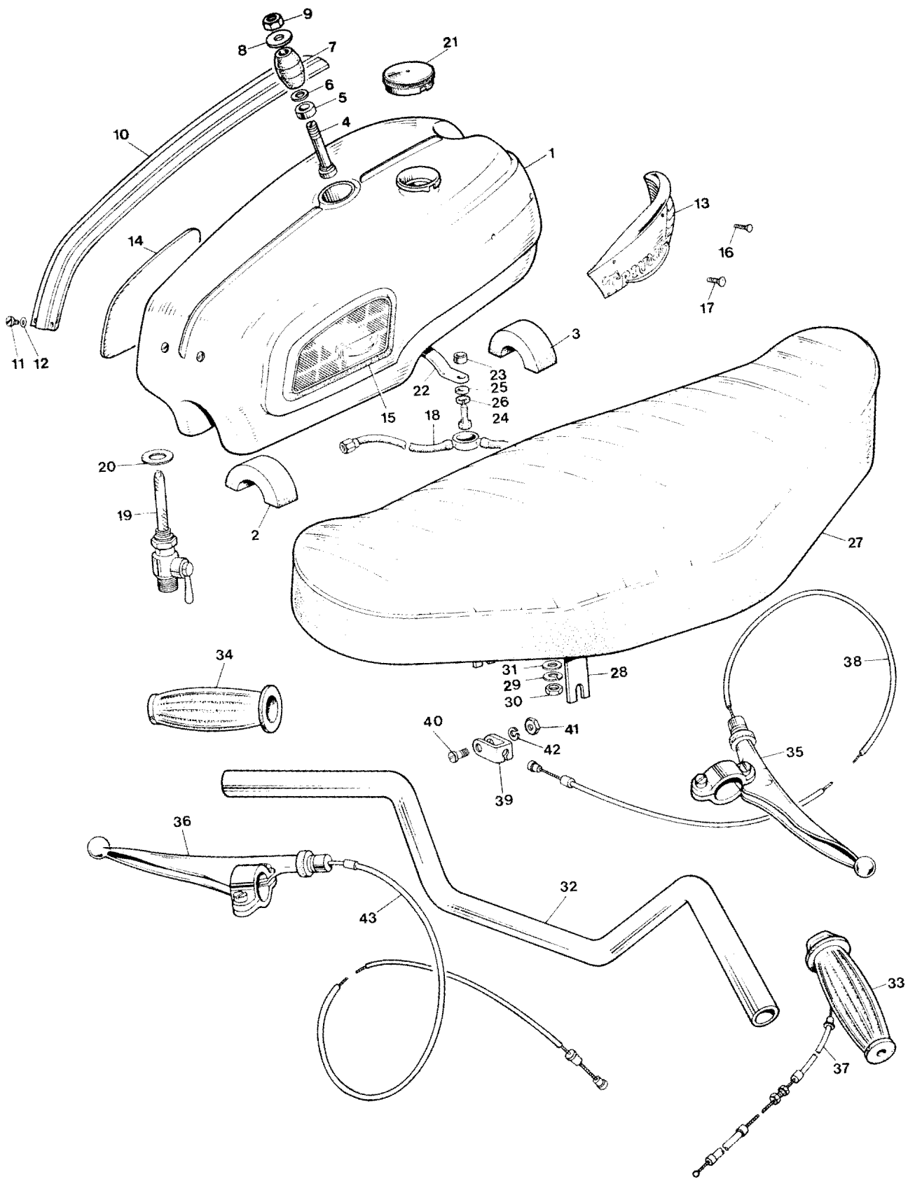
Fig.13 GAS TANK, TWIN SEAT AND HANDLEBARS
