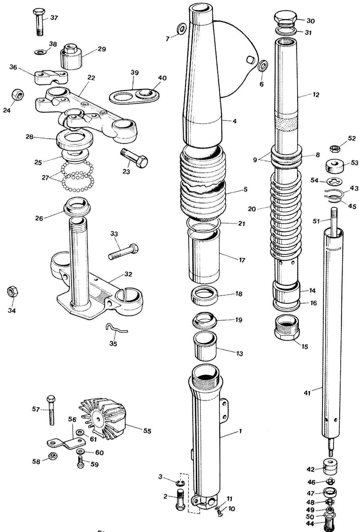
Fig. 9 TELESCOPIC FRONT FORK
