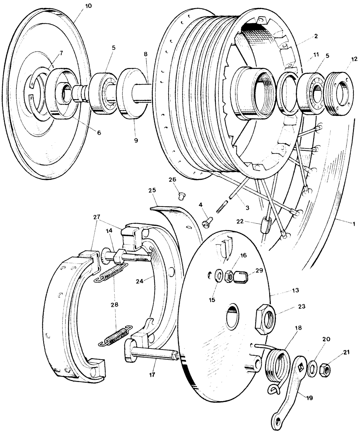
Fig.10 FRONT WHEEL
