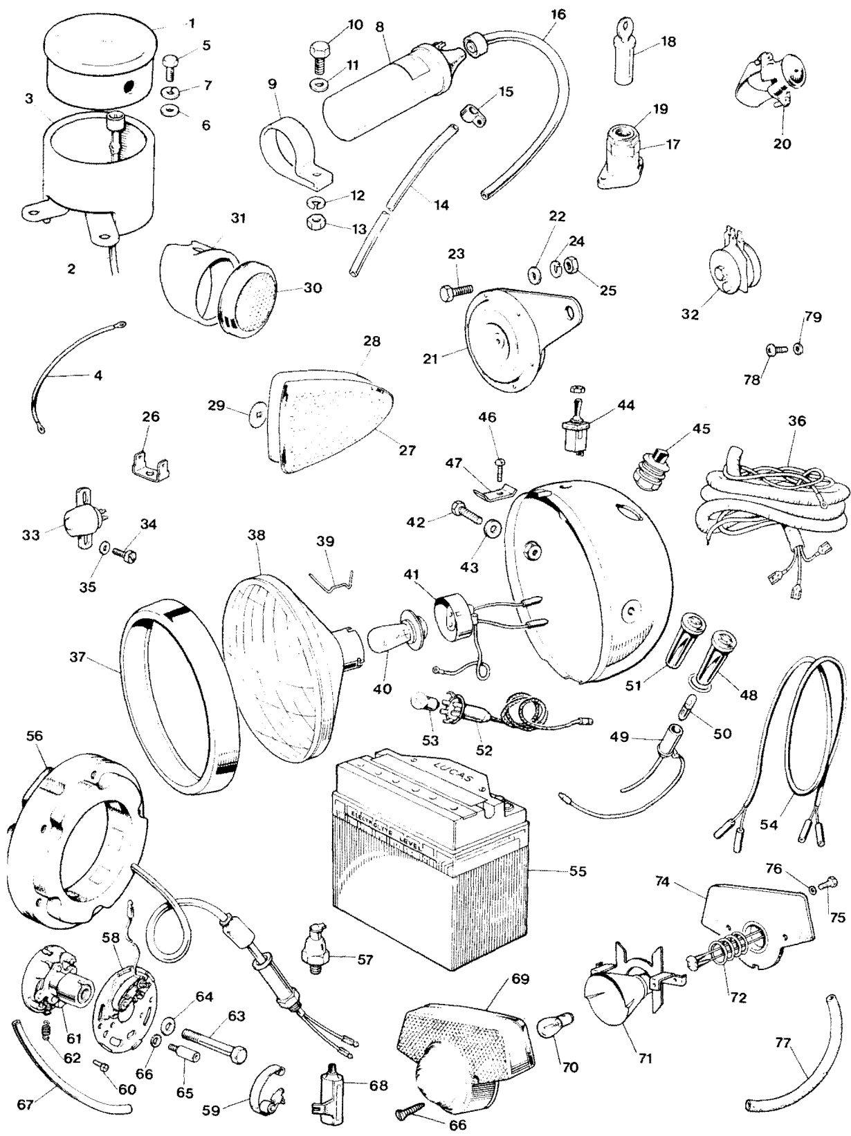
Fig.14 ELECTRICAL EQUIPMENT
