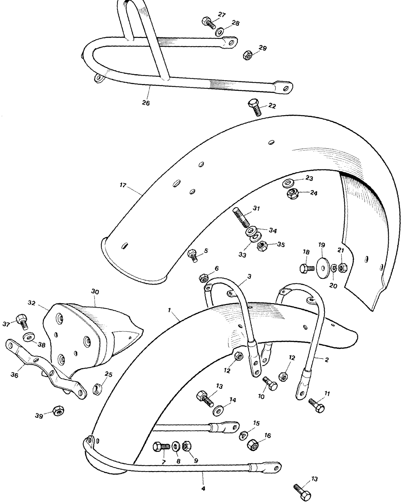
Fig.12 FENDERS
