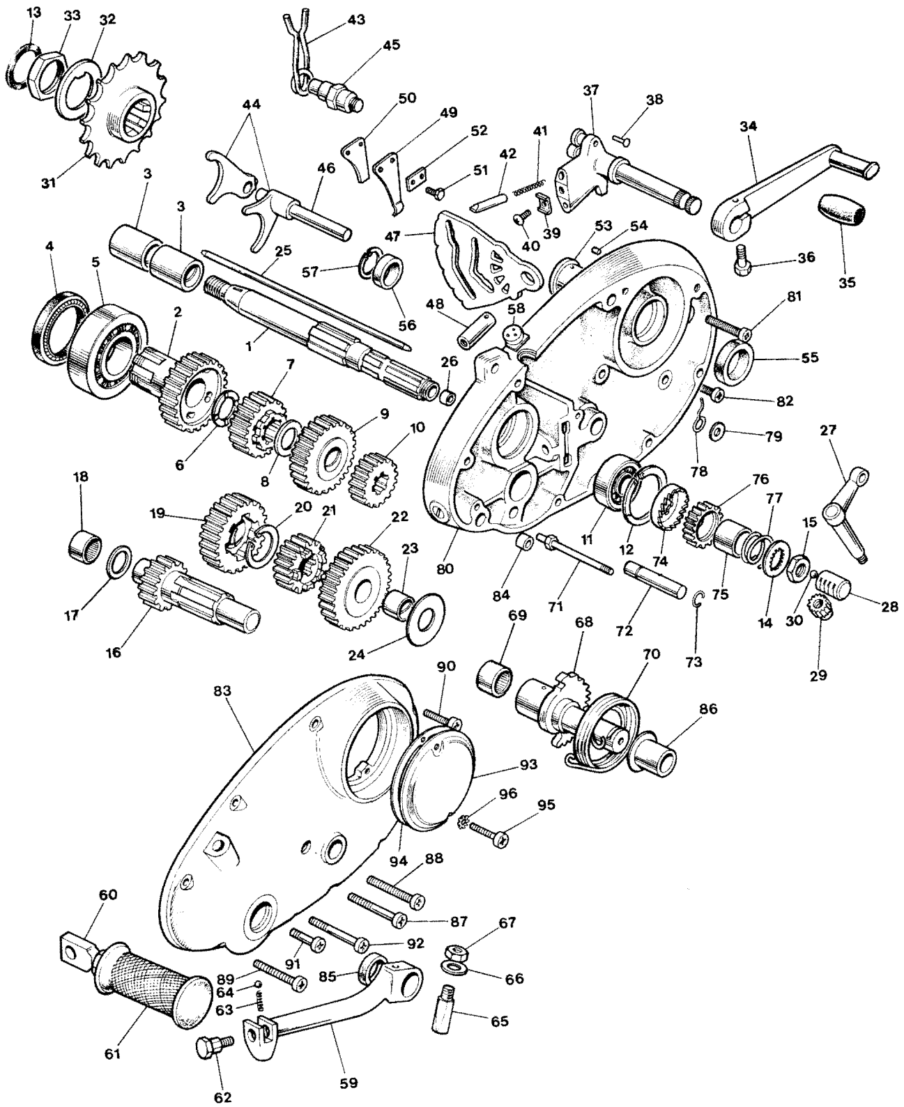
Fig. 3 GEAR CLUSTER
